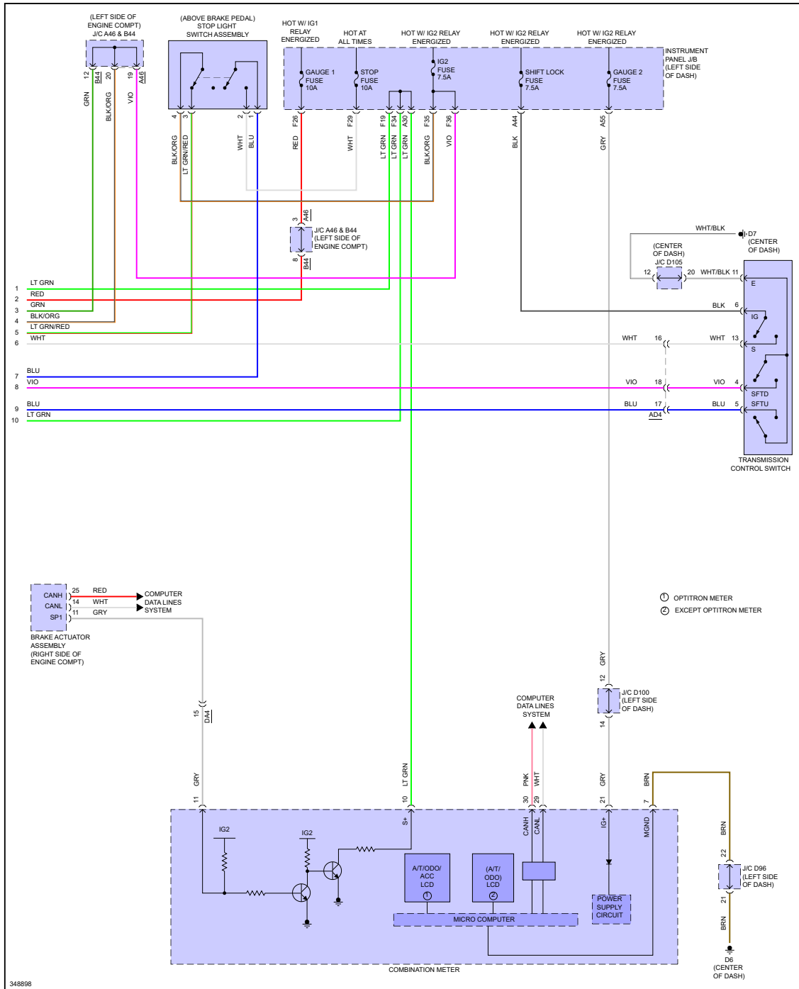
Fig 2: 2.7L, A/T Circuit (2 of 2)
