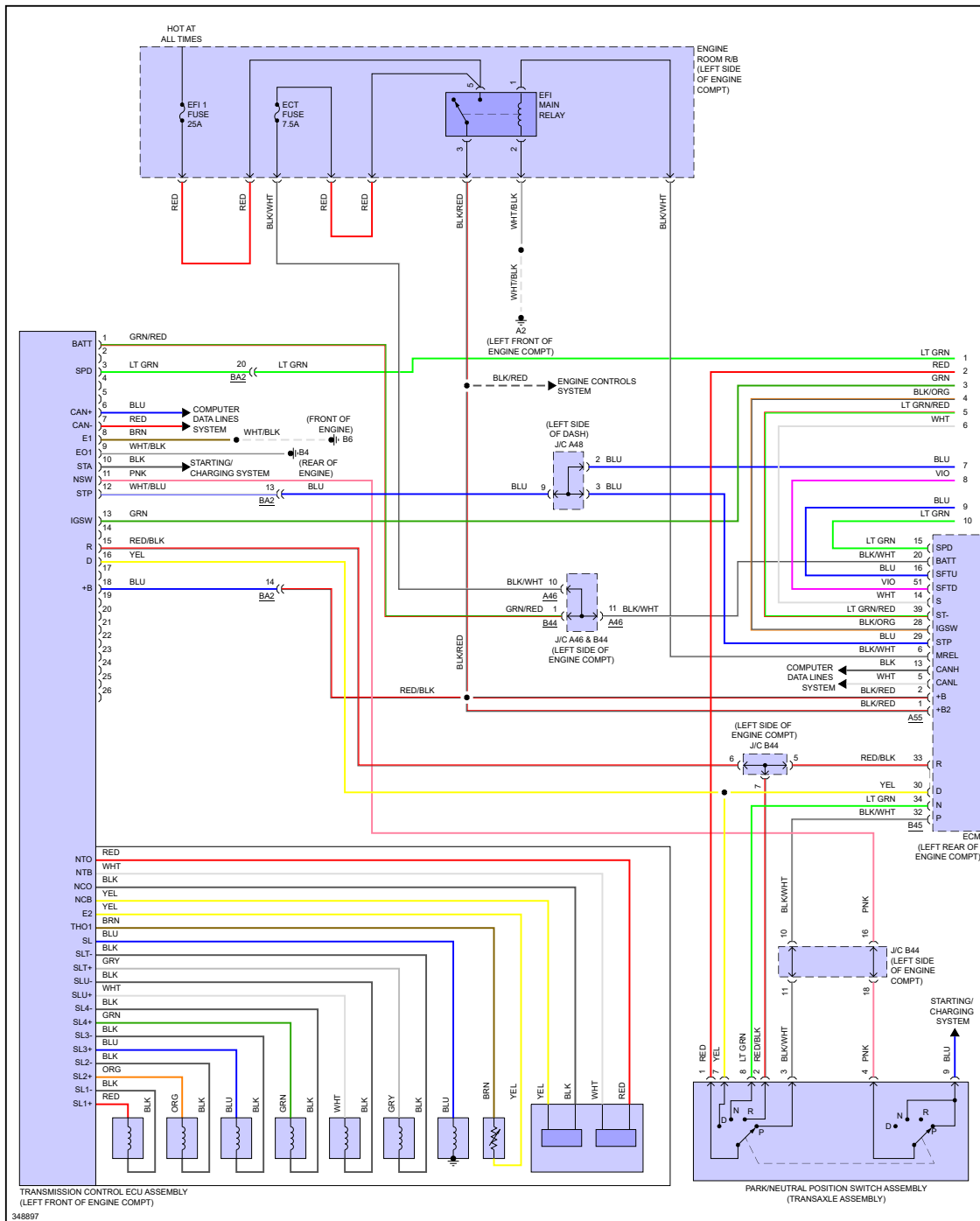
Fig 1: 2.7L, A/T Circuit (1 of 2)
