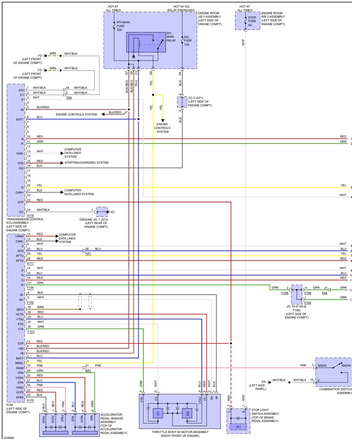
Fig 1: Transmission Circuit (1 of 3)
