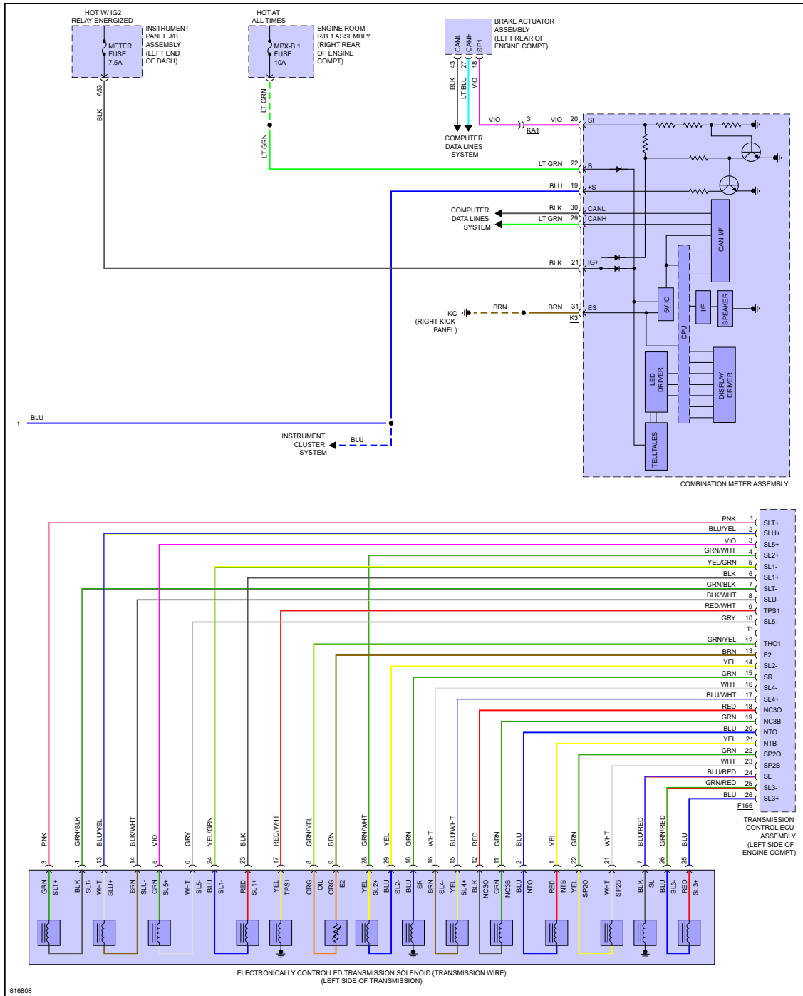
Fig 3: Transmission Circuit (3 of 3)
