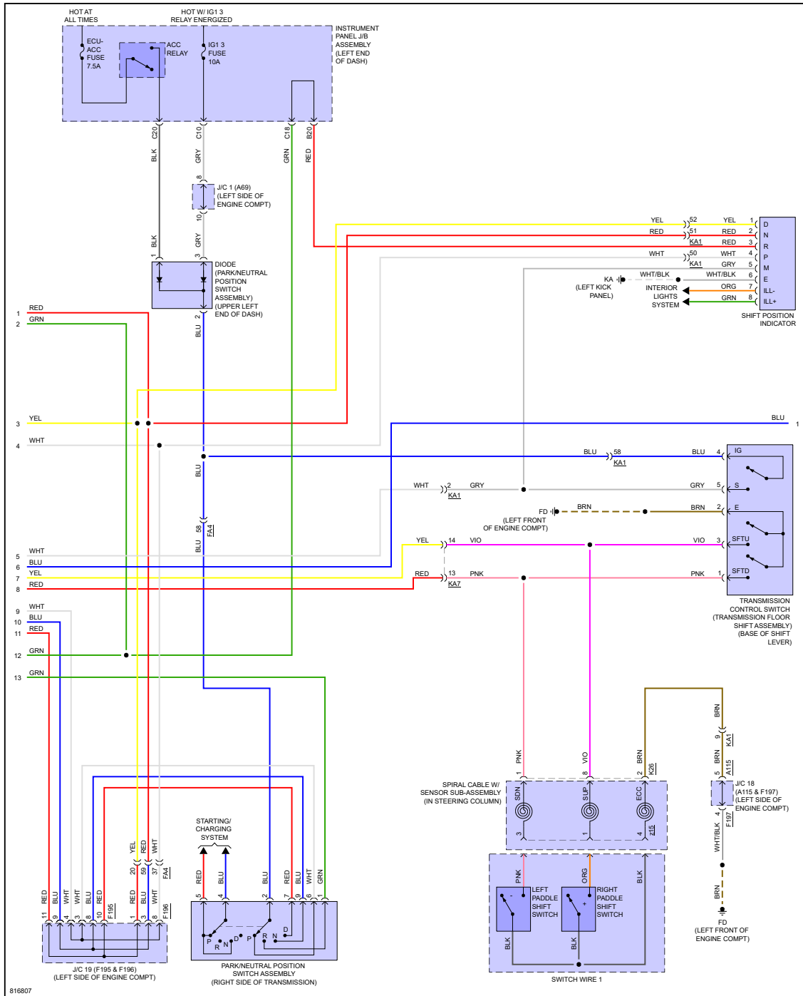
Fig 2: Transmission Circuit (2 of 3)
