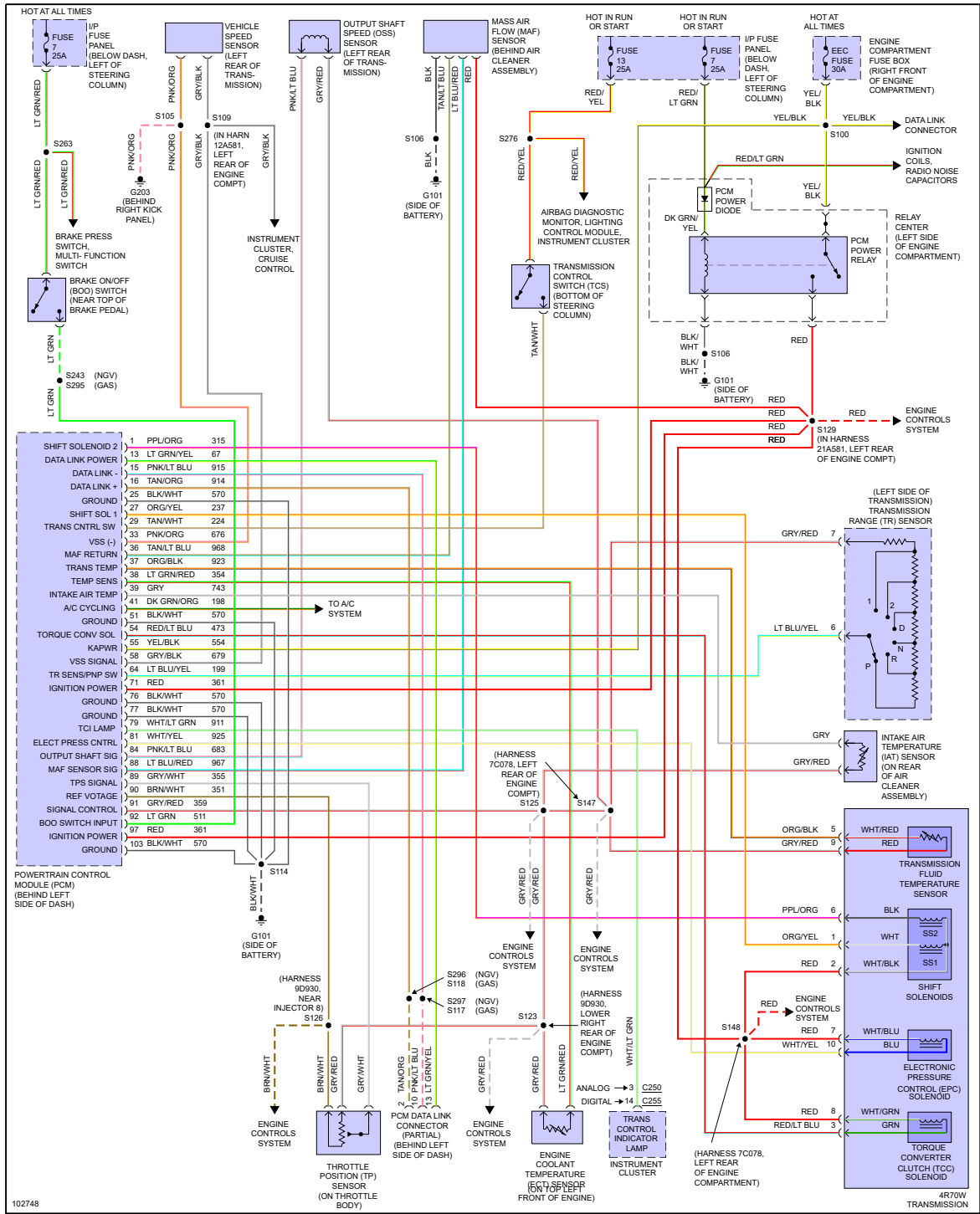
Fig 1: A/T Circuit
