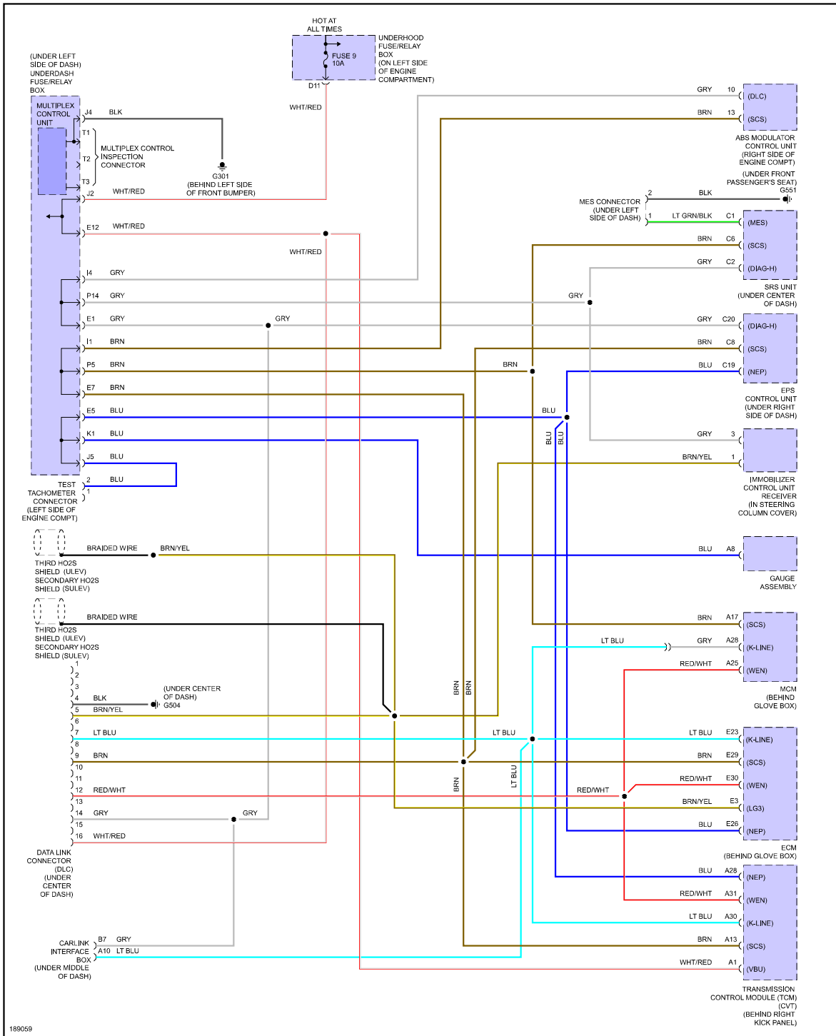
Fig 3: Computer Data Lines Circuit, Hybrid
