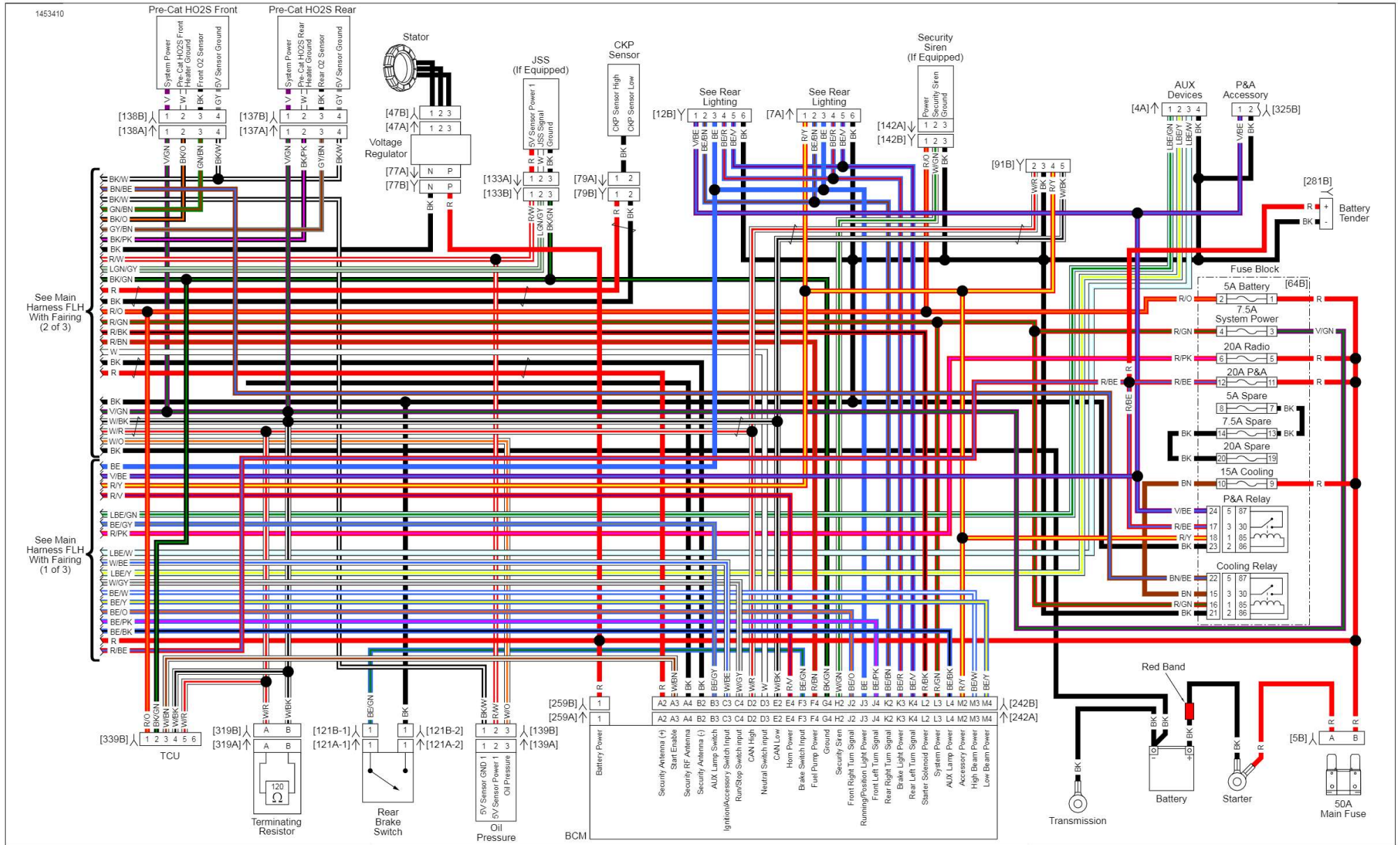
Main Harness FLH (3 of 3): 2021 Touring (with Fairing)
