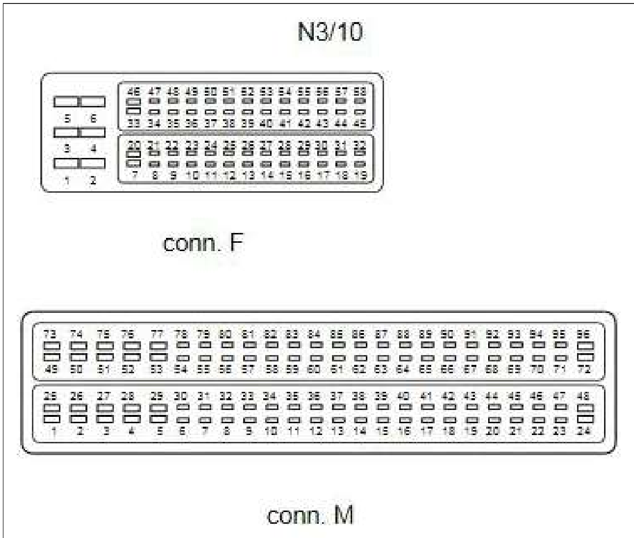
Fig 1: ME-SFI [ME] Control Unit Connector End View (N3/10)
