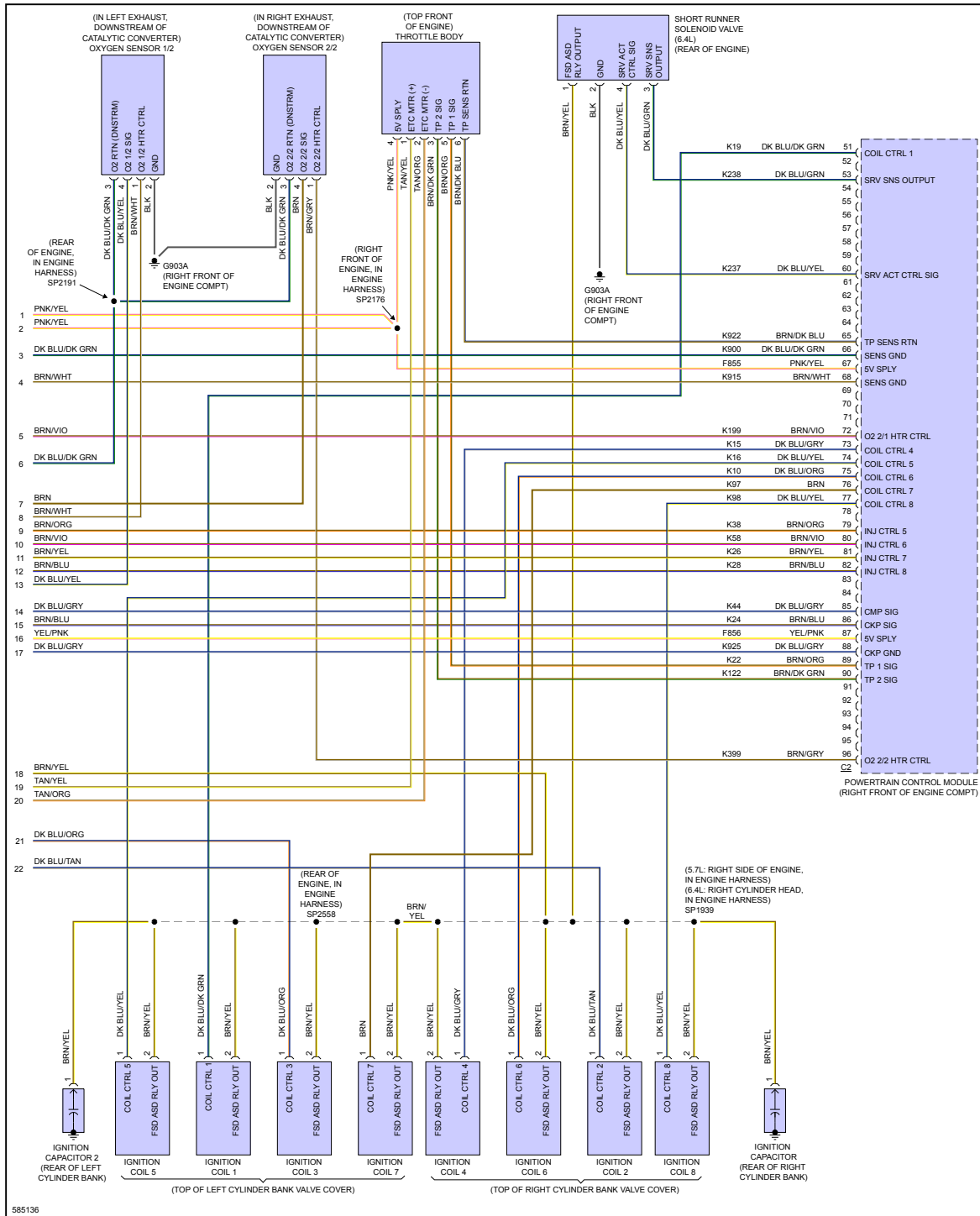
Fig 6: 6.4L, Engine Performance Circuit (6 of 6)
