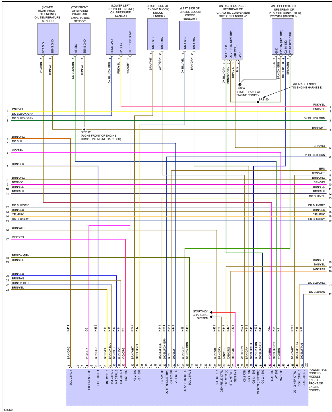
Fig 5: 6.4L, Engine Performance Circuit (5 of 6)
