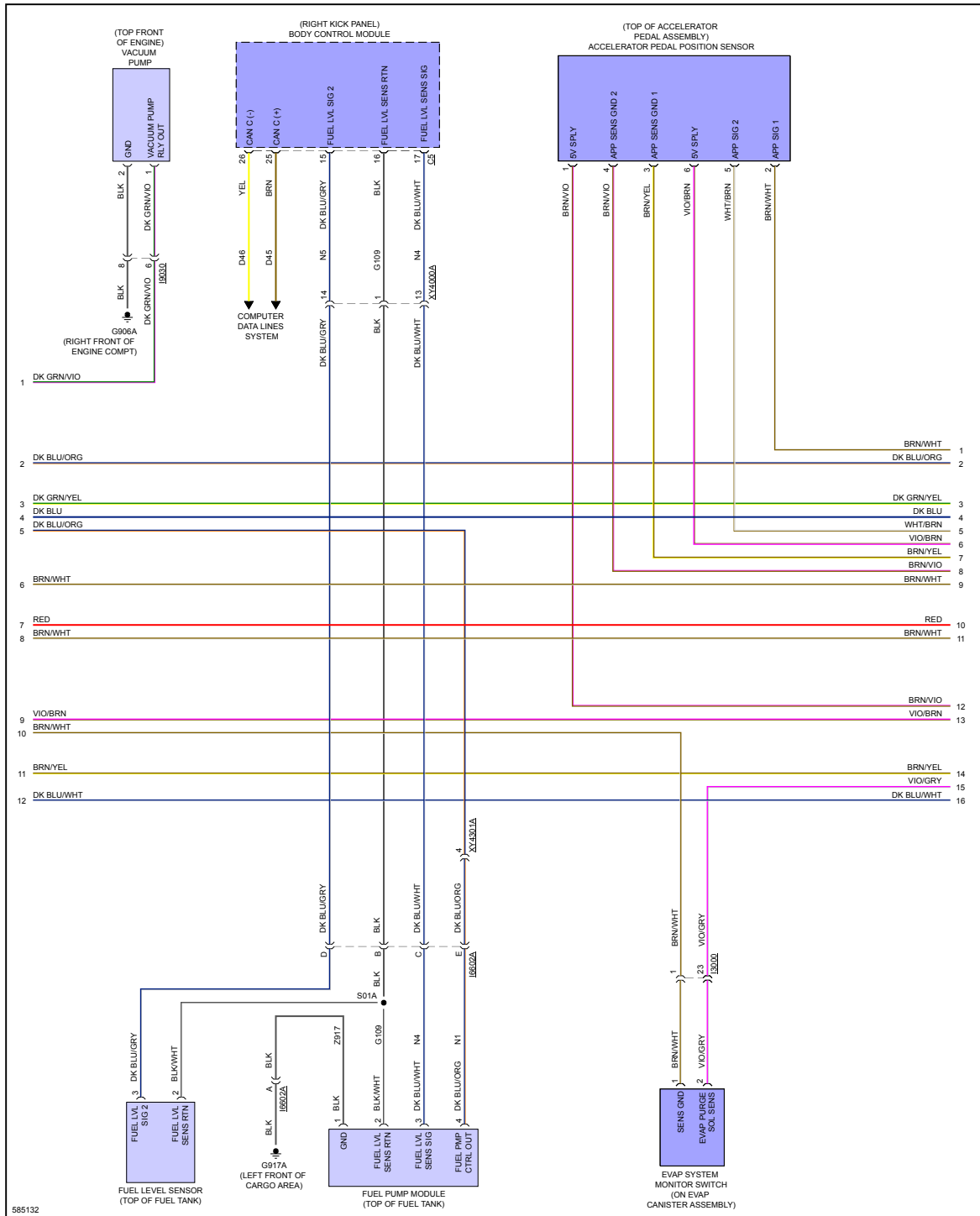
Fig 2: 6.4L, Engine Performance Circuit (2 of 6)
