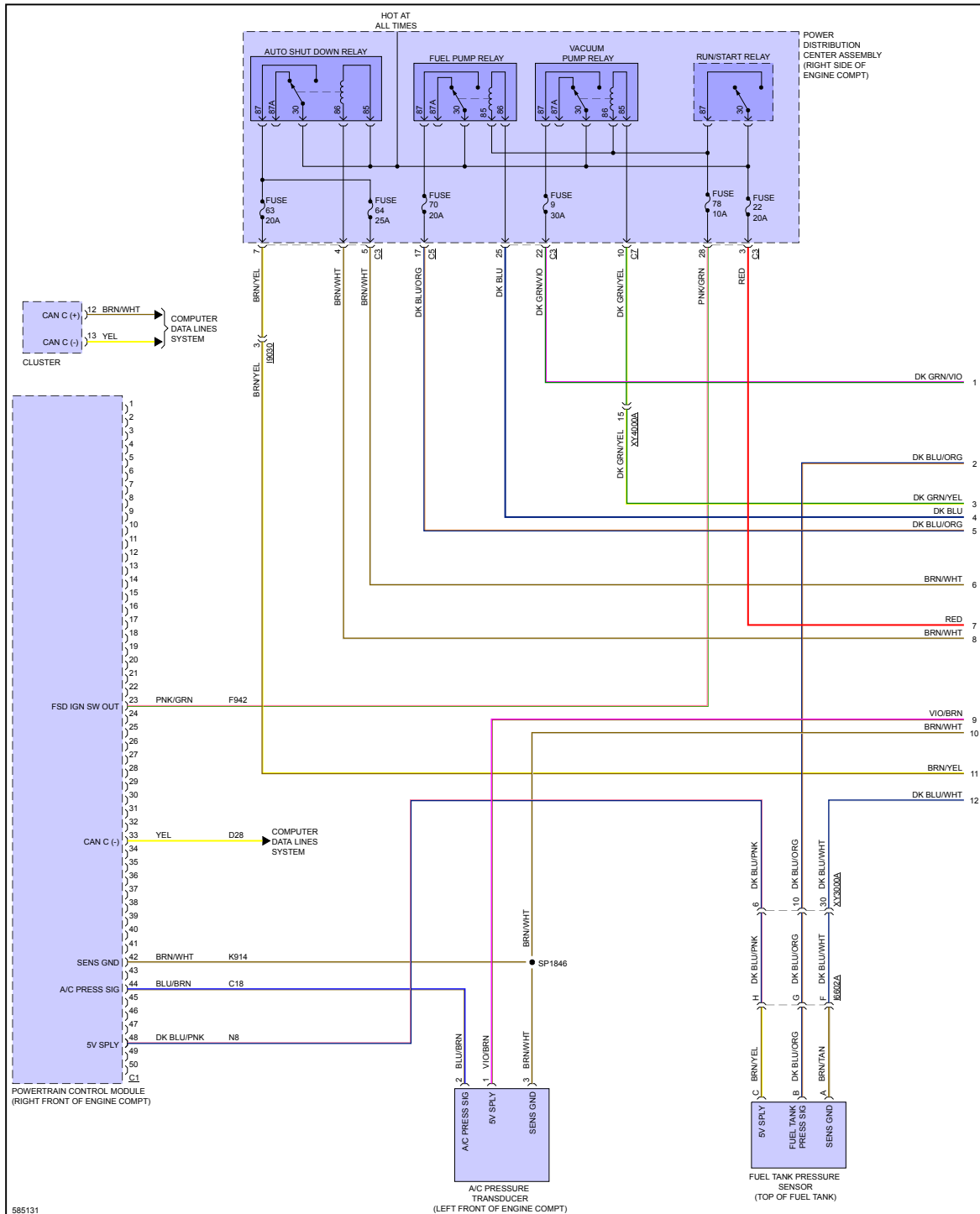
Fig 1: 6.4L, Engine Performance Circuit (1 of 6)
