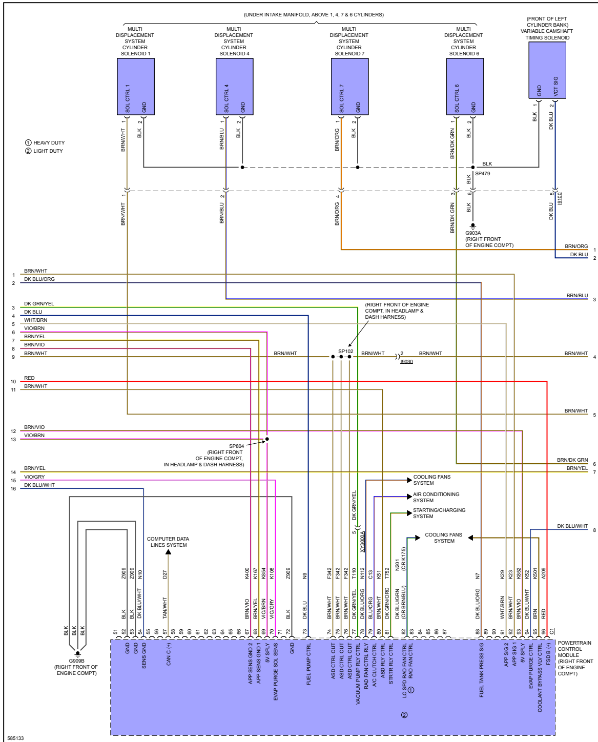
Fig 3: 6.4L, Engine Performance Circuit (3 of 6)
