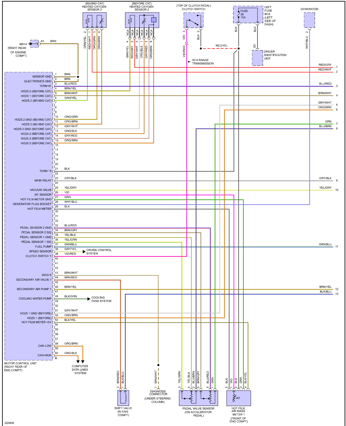
Fig 1: 3.2L, Engine Performance Circuit (1 of 4)
