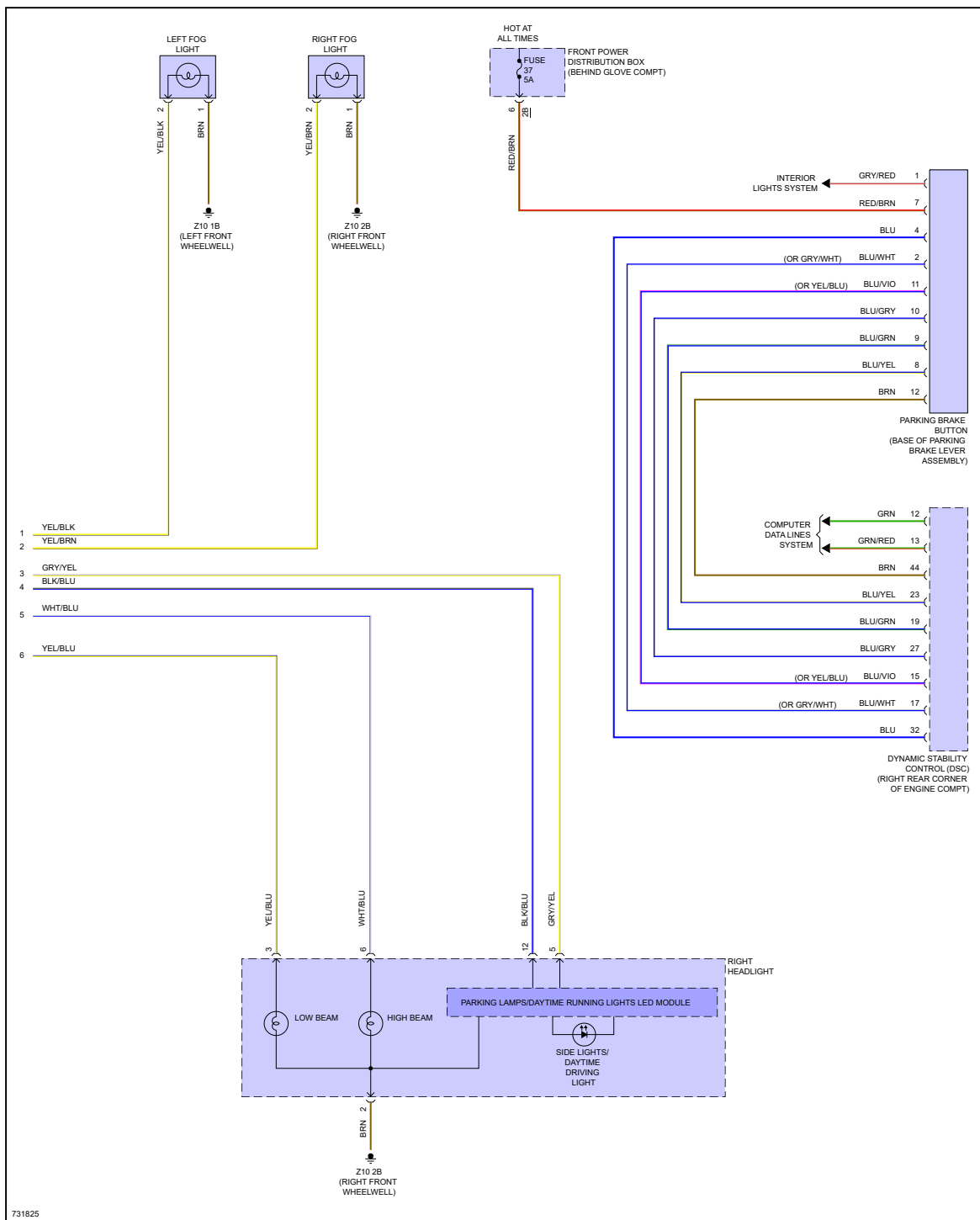
Fig 4: Headlights Circuit, W/O LED Headlamps (2 of 2)
