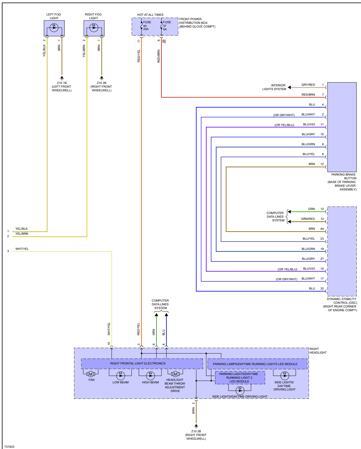
Fig 2: Headlights Circuit, W/ LED Headlamps (2 of 2)
