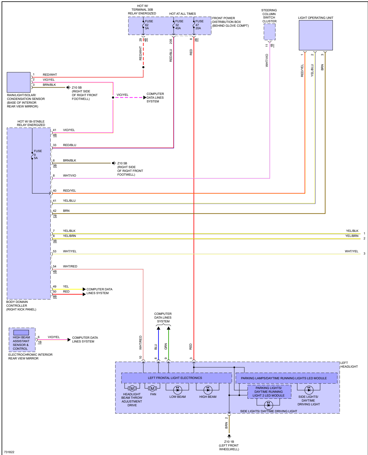
Fig 1: Headlights Circuit, W/ LED Headlamps (1 of 2)
