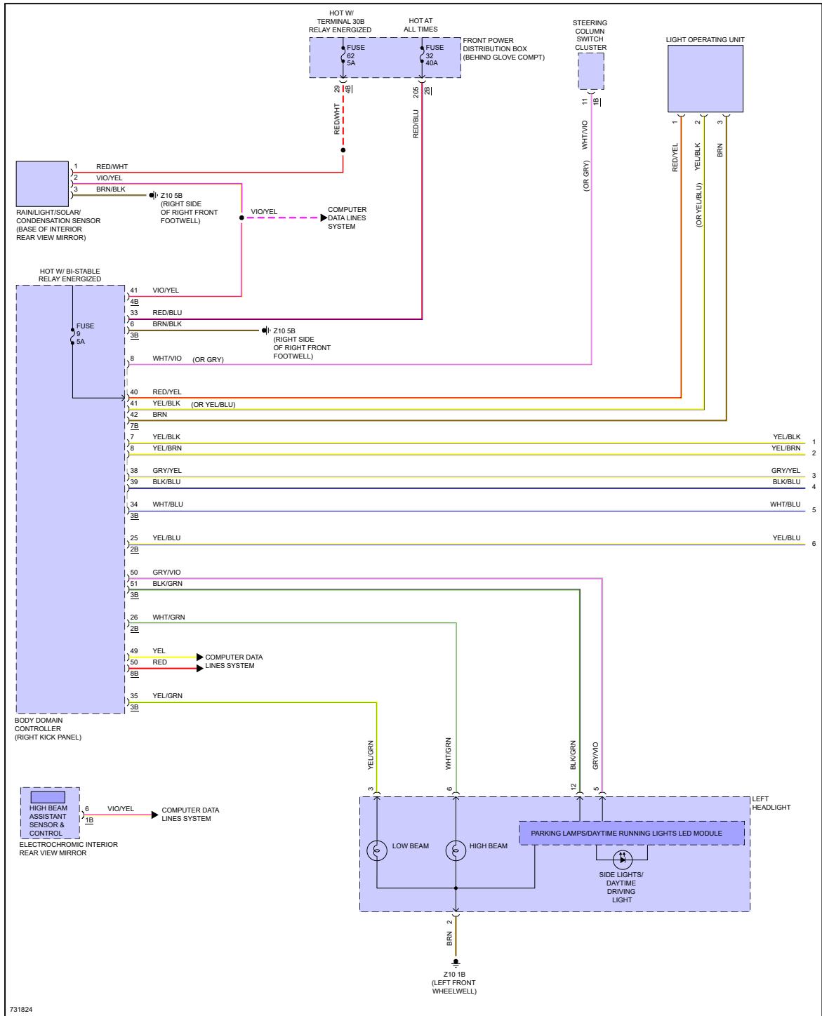
Fig 3: Headlights Circuit, W/O LED Headlamps (1 of 2)
