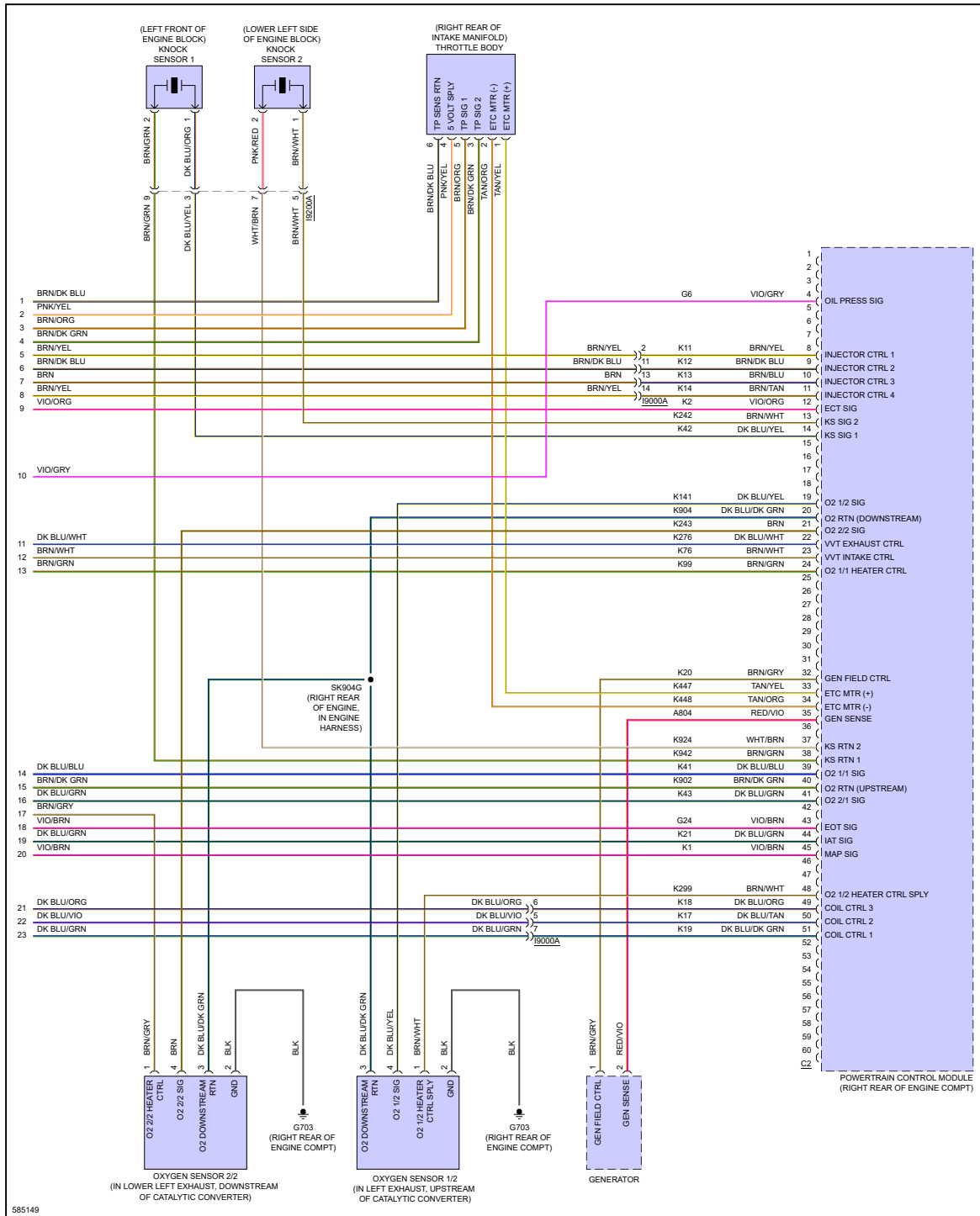
Fig 7: 3.6L, Engine Performance Circuit (7 of 7)
