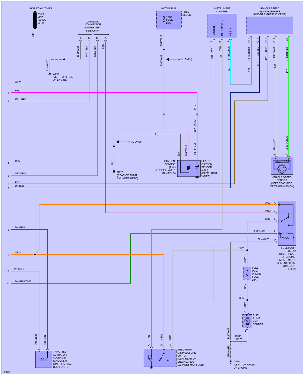
Fig 6: 7.4L (VIN N), Engine Performance Circuits, M/T (3 of 3)
