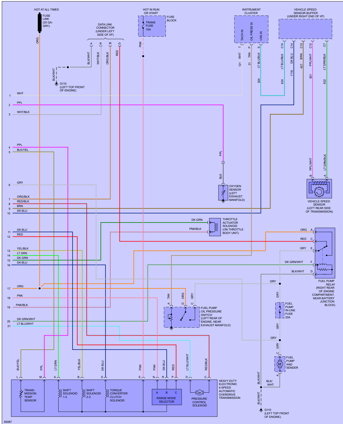
Fig 3: 7.4L (VIN N), Engine Performance Circuits, A/T (3 of 3)
