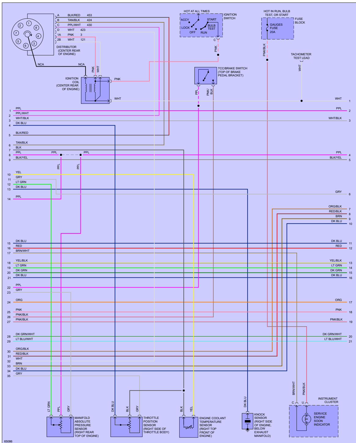
Fig 2: 7.4L (VIN N), Engine Performance Circuits, A/T (2 of 3)
