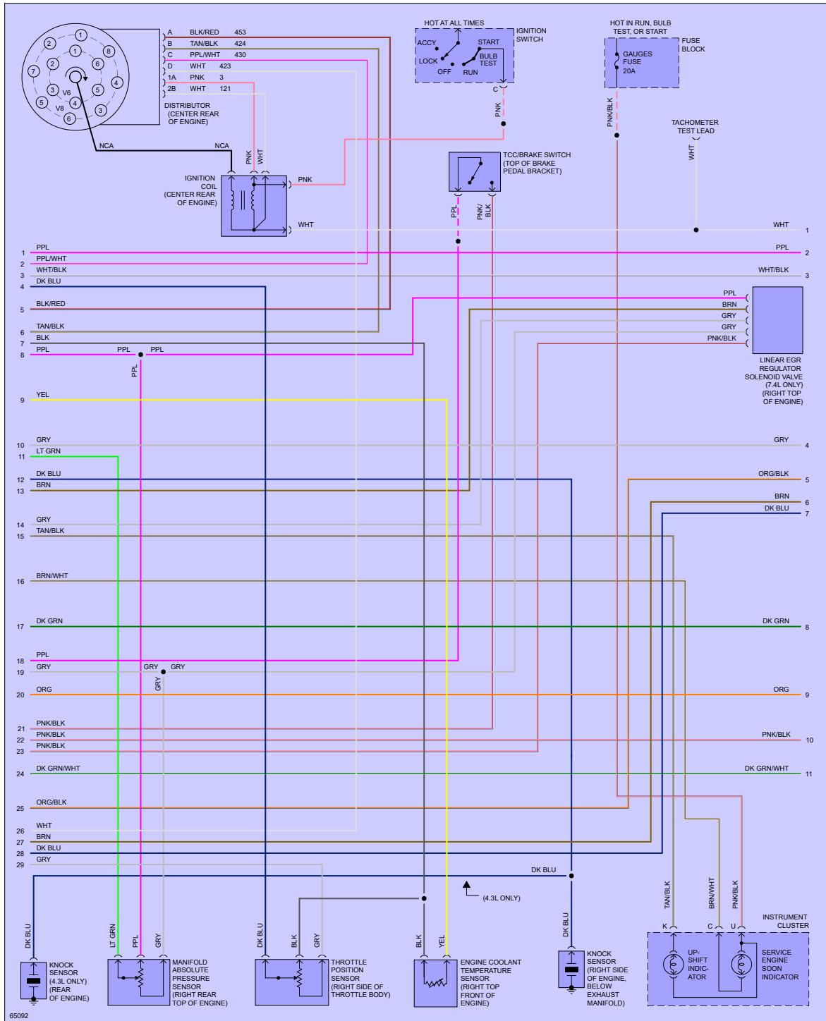
Fig 5: 7.4L (VIN N), Engine Performance Circuits, M/T (2 of 3)
