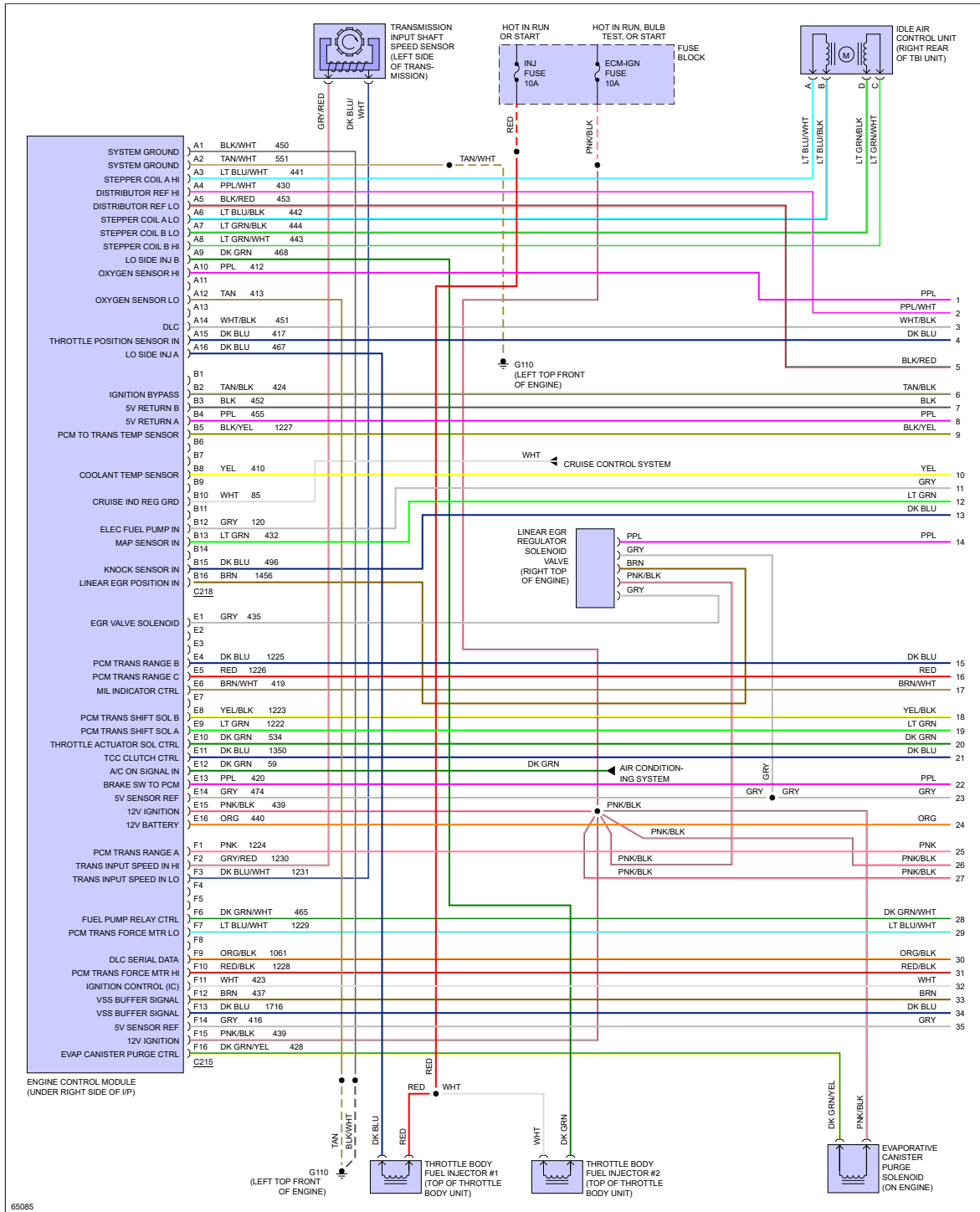
Fig 1: 7.4L (VIN N), Engine Performance Circuits, A/T (1 of 3)
