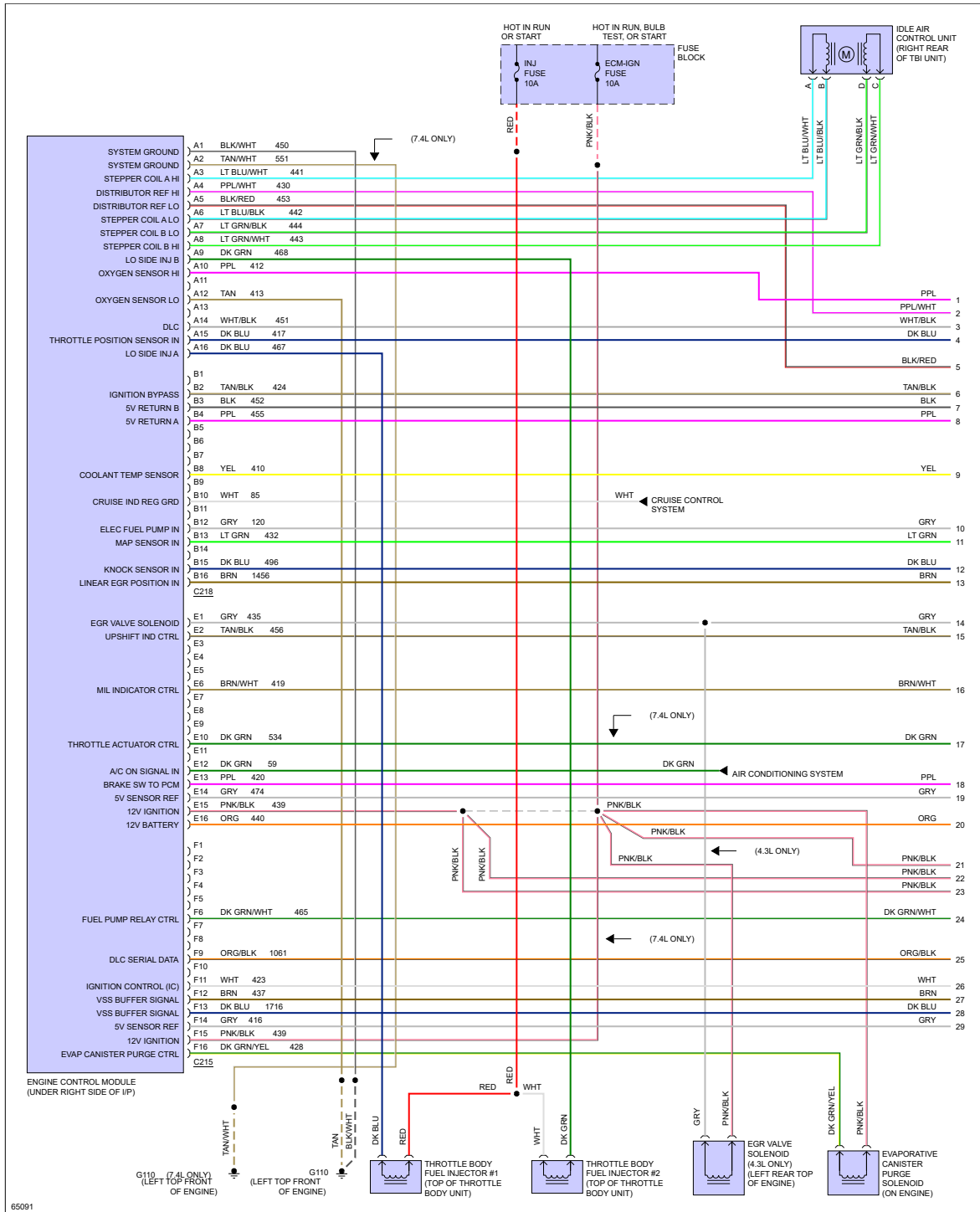
Fig 4: 7.4L (VIN N), Engine Performance Circuits, M/T (1 of 3)
