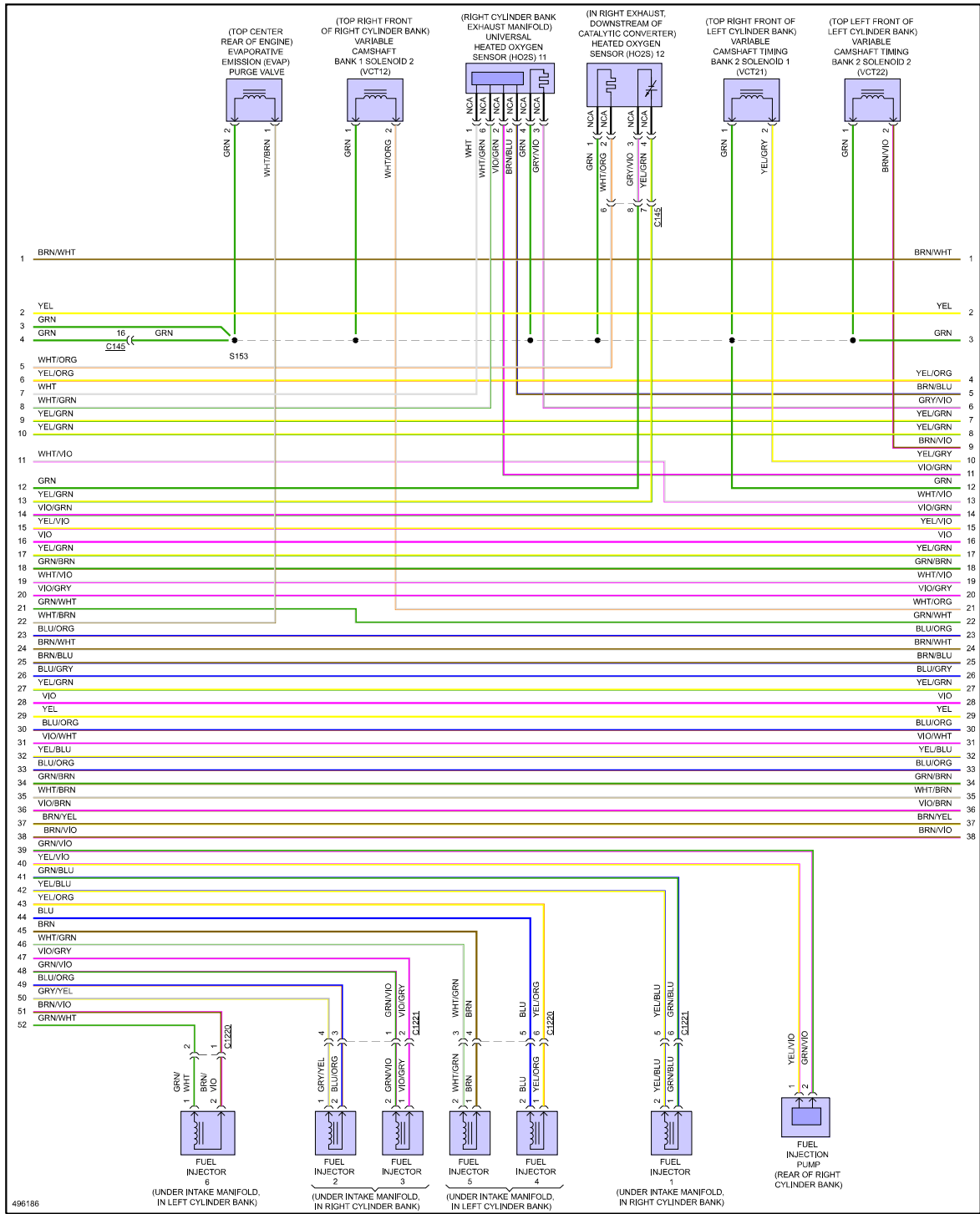
Fig 7: 2.7L Turbo, Engine Performance Circuit (7 of 9)
