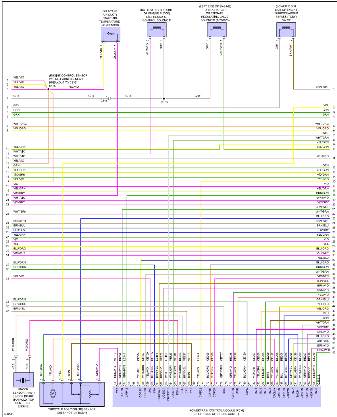
Fig 6: 2.7L Turbo, Engine Performance Circuit (6 of 9)
