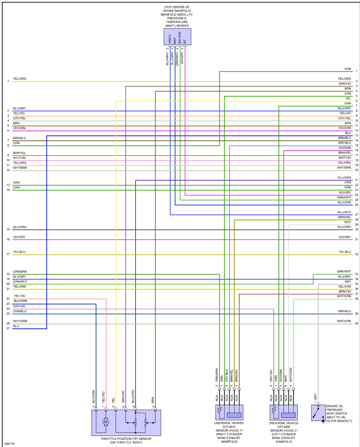
Fig 6: 3.5L, Engine Performance Circuit (6 of 7)
