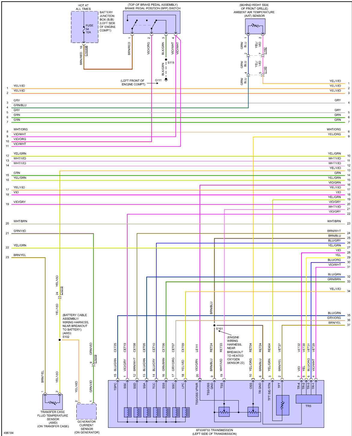
Fig 5: 2.7L Turbo, Engine Performance Circuit (5 of 9)
