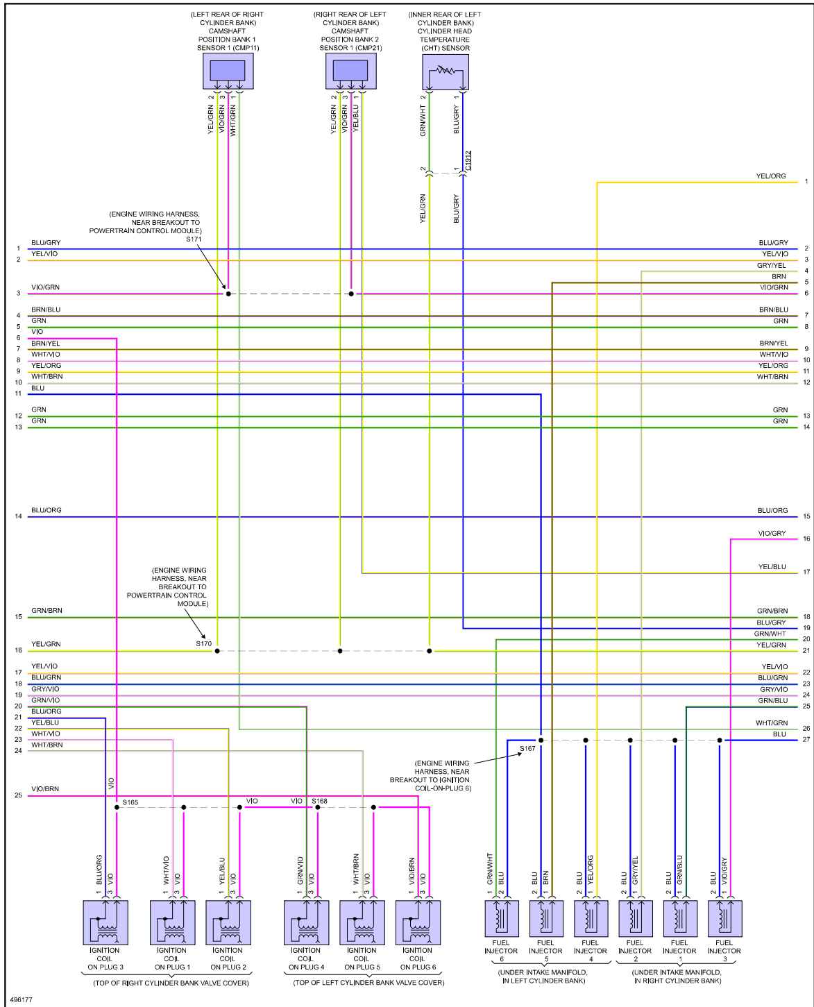
Fig 5: 3.5L, Engine Performance Circuit (5 of 7)
