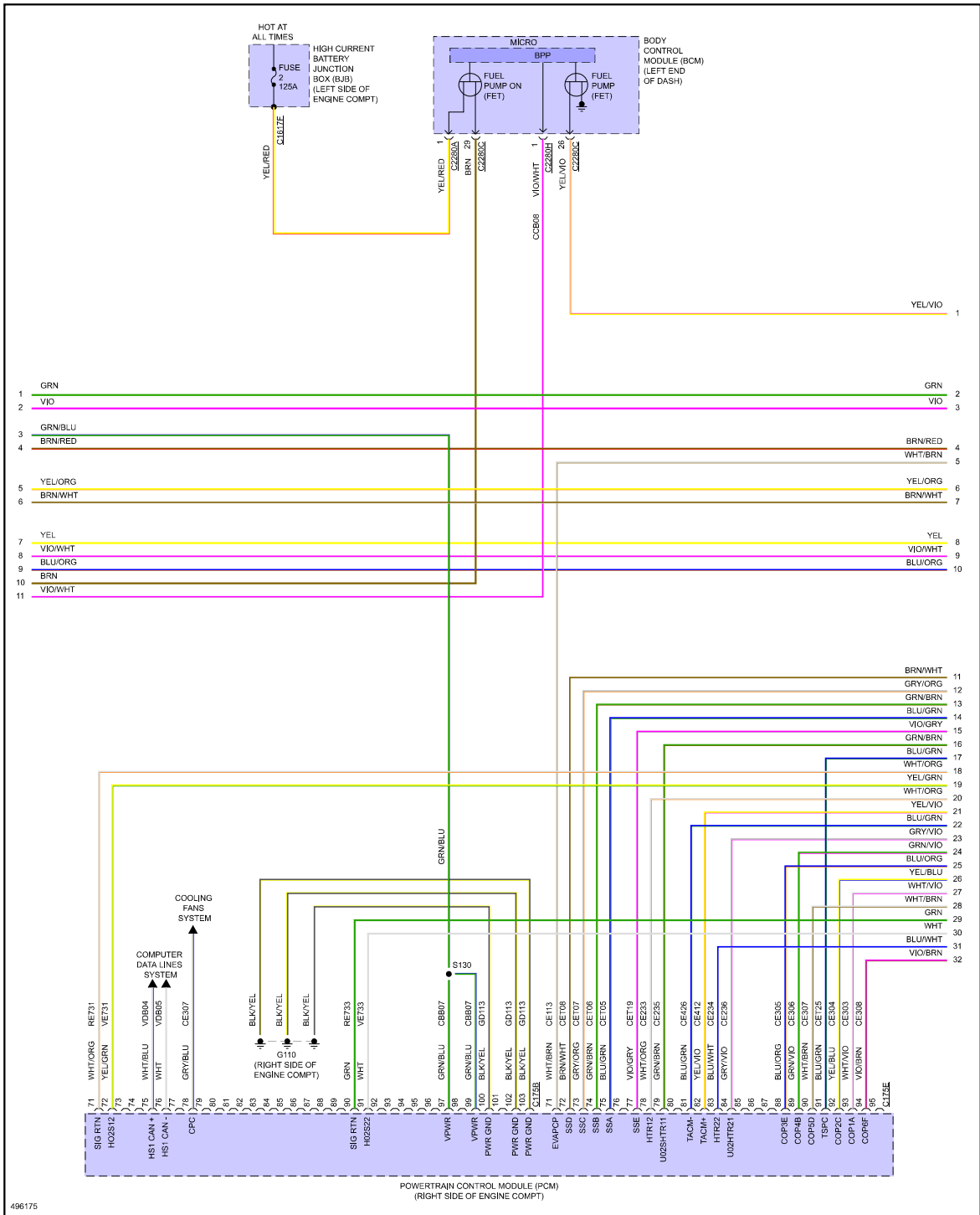
Fig 3: 3.5L, Engine Performance Circuit (3 of 7)
