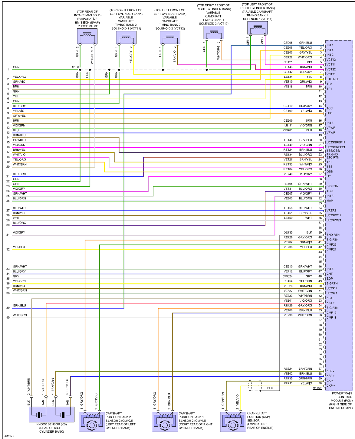
Fig 7: 3.5L, Engine Performance Circuit (7 of 7)
