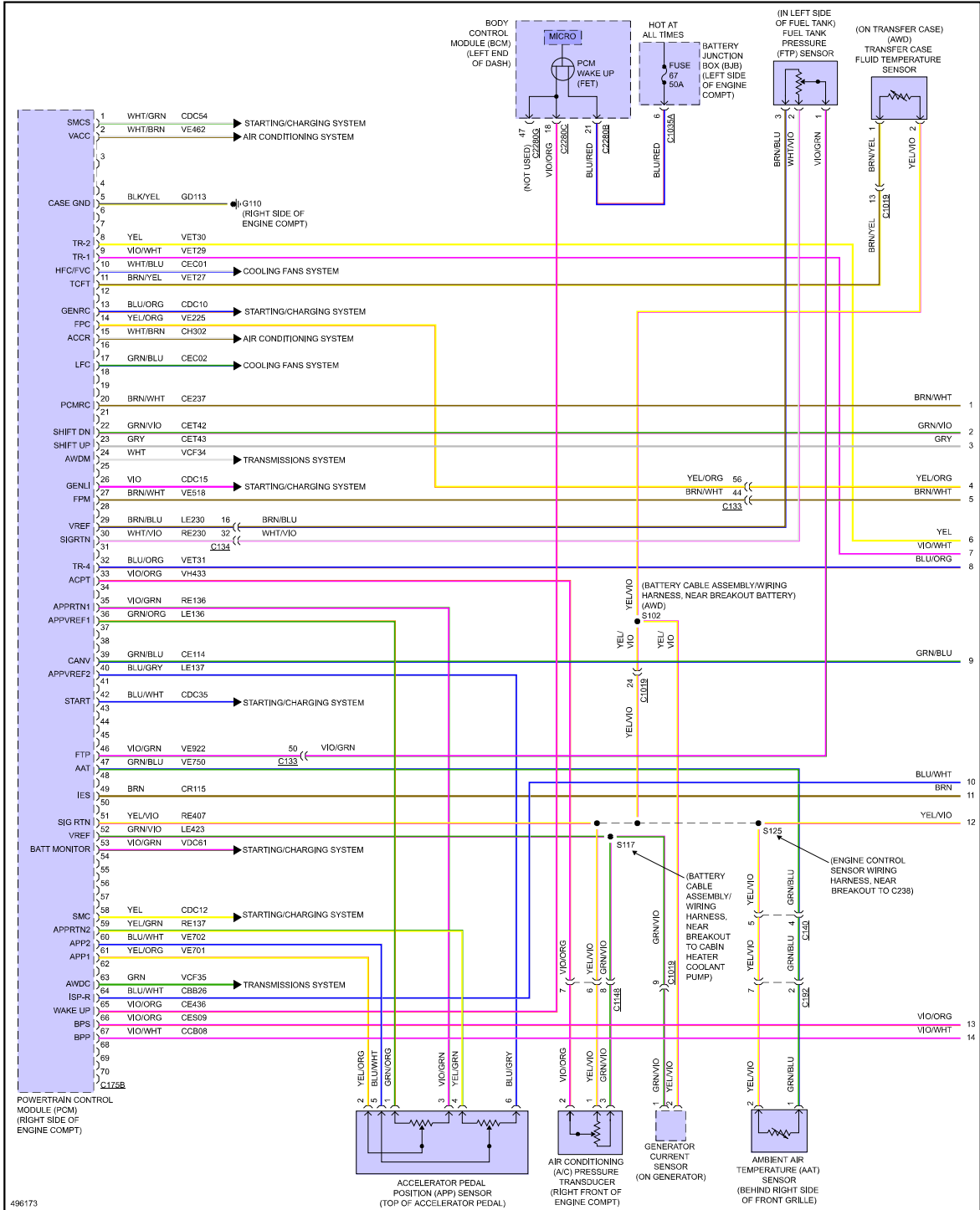
Fig 1: 3.5L, Engine Performance Circuit (1 of 7)
