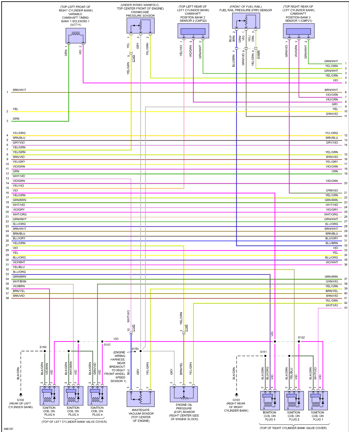
Fig 8: 2.7L Turbo, Engine Performance Circuit (8 of 9)
