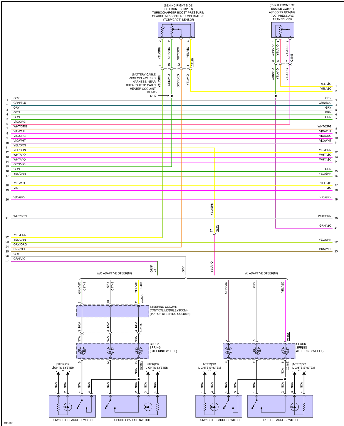
Fig 4: 2.7L Turbo, Engine Performance Circuit (4 of 9)
