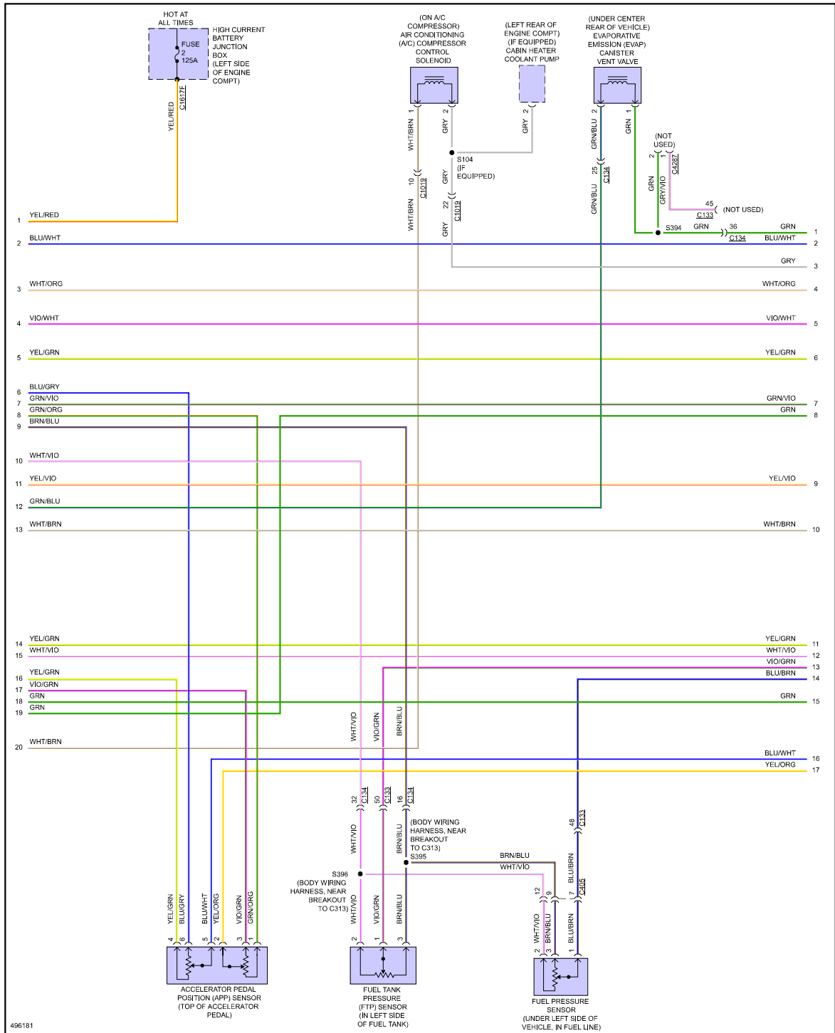
Fig 2: 2.7L Turbo, Engine Performance Circuit (2 of 9)
