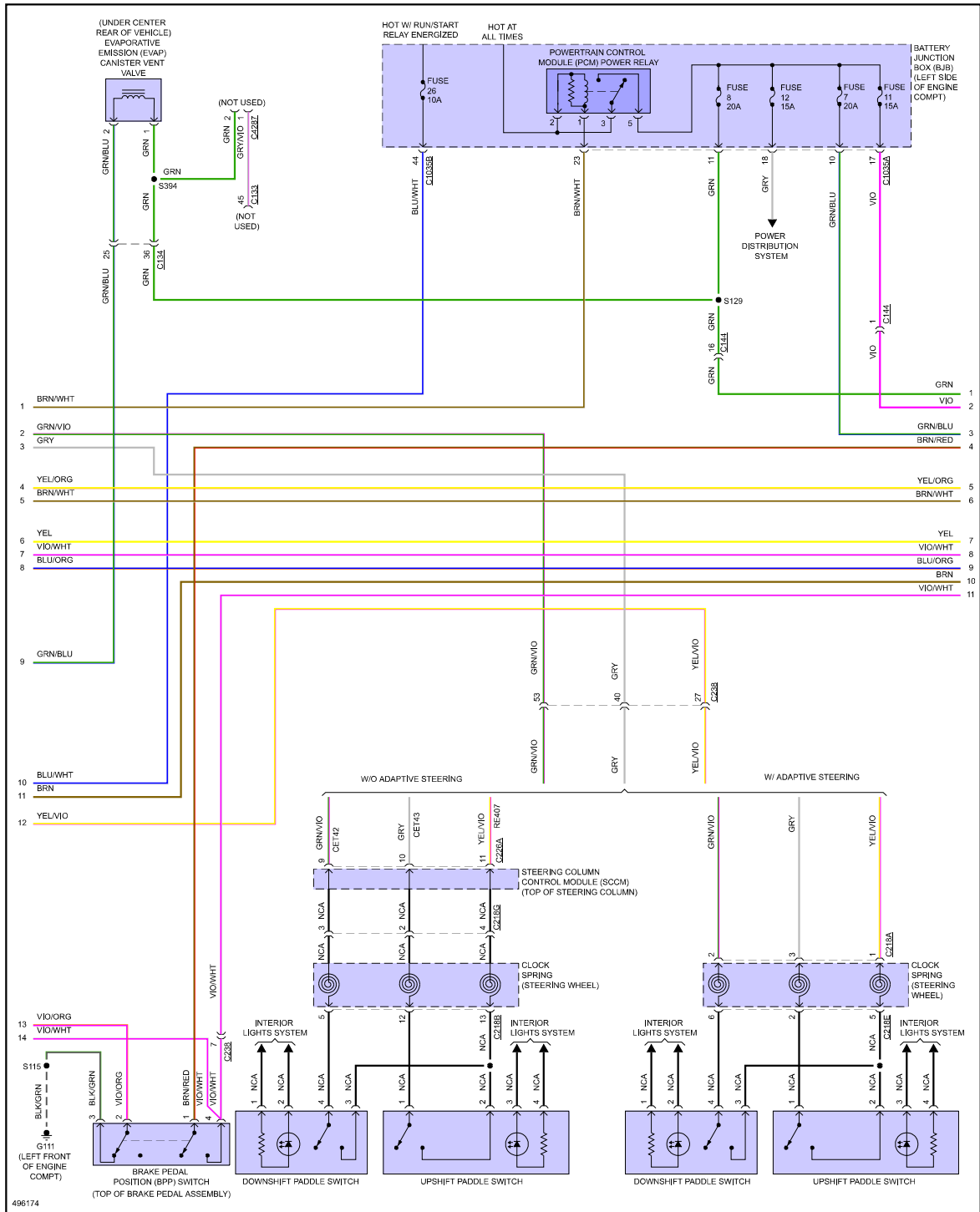
Fig 2: 3.5L, Engine Performance Circuit (2 of 7)
