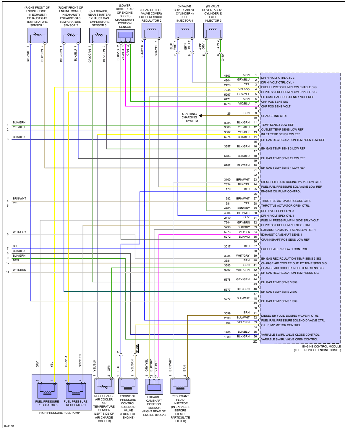
Fig 9: 3.0L VIN T, Engine Performance Circuit (9 of 9)
