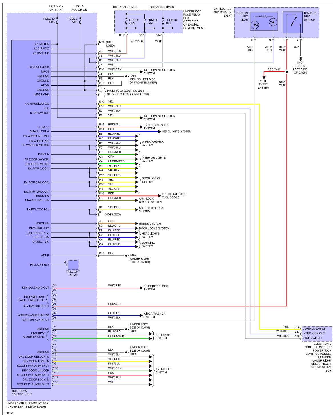
Fig 1: Multiplex Control Circuit
