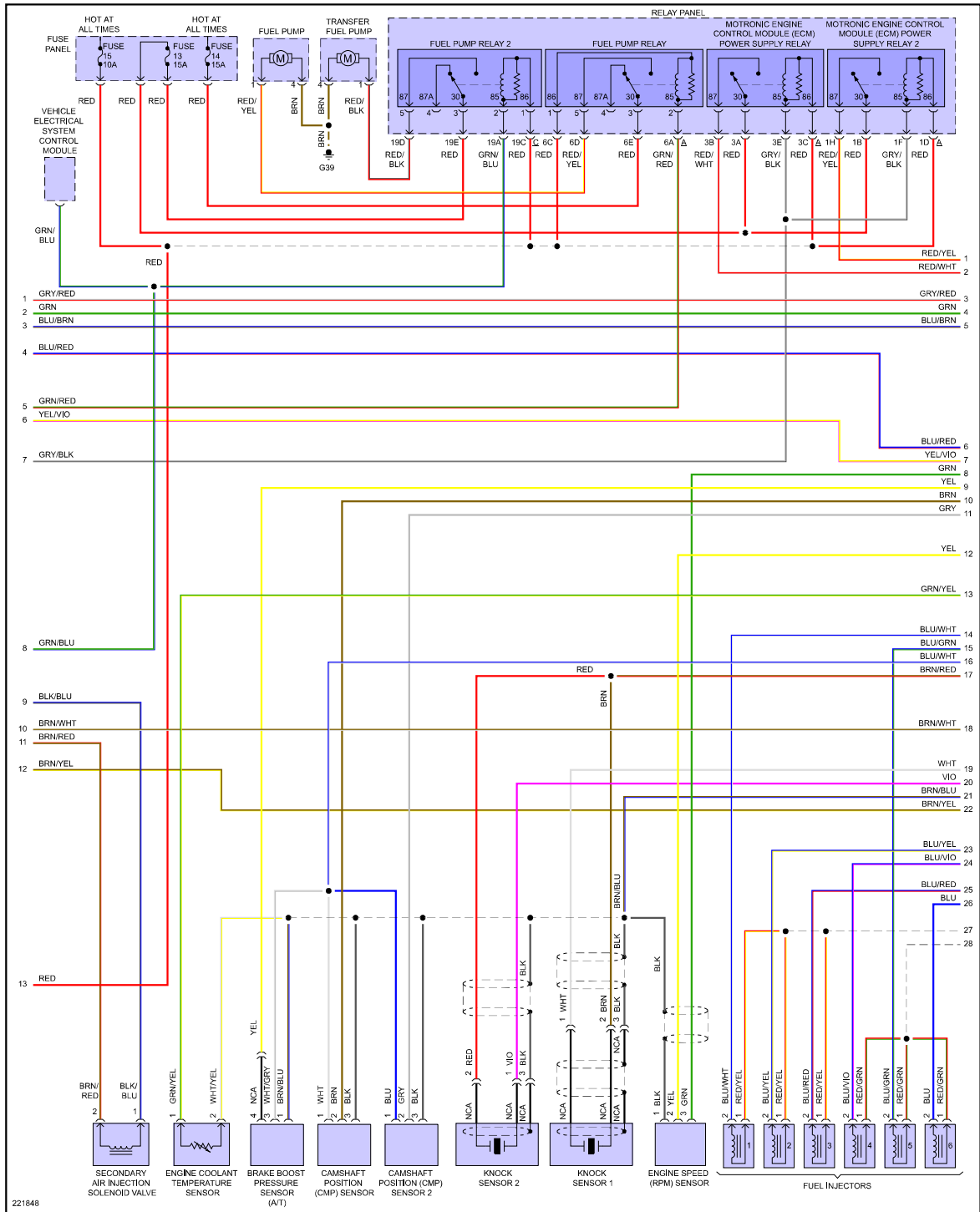
Fig 2: 3.2L, Engine Performance Circuit (2 of 3)
