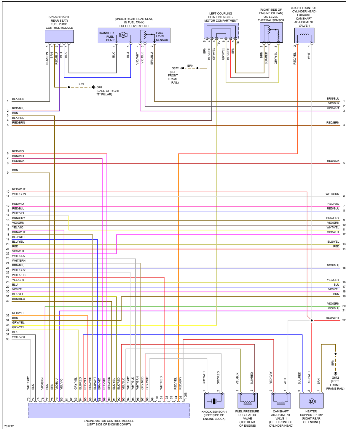
Fig 7: 2.0L Turbo, Engine Performance Circuit (7 of 8)
