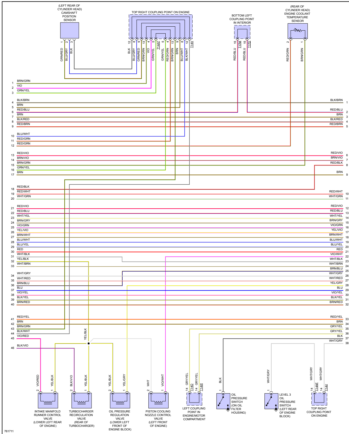
Fig 6: 2.0L Turbo, Engine Performance Circuit (6 of 8)
