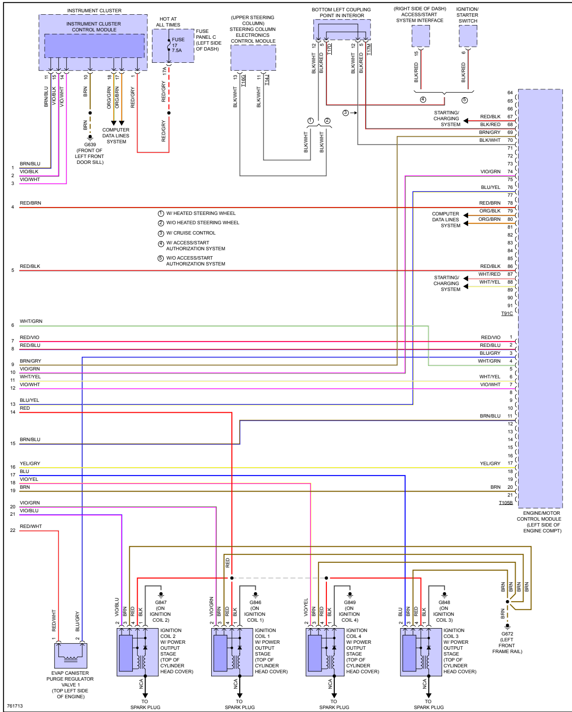
Fig 8: 2.0L Turbo, Engine Performance Circuit (8 of 8)
