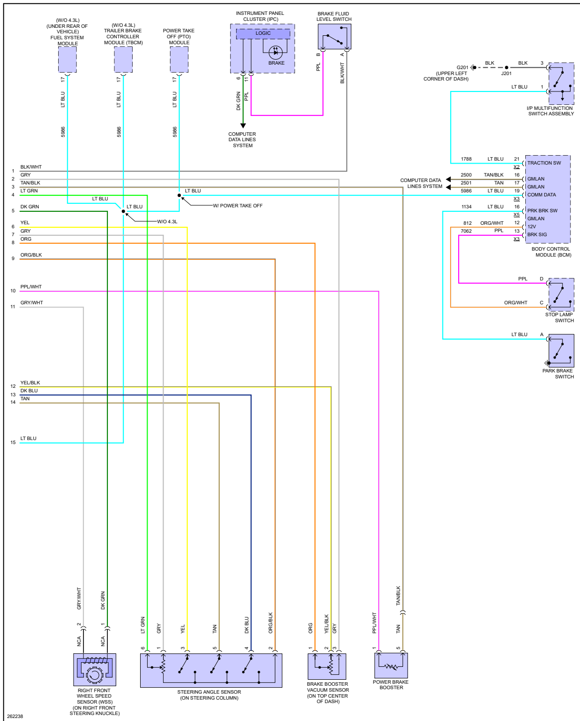
Fig 2: Anti-Lock Brake Circuit, W/ JL4 (2 of 2)
