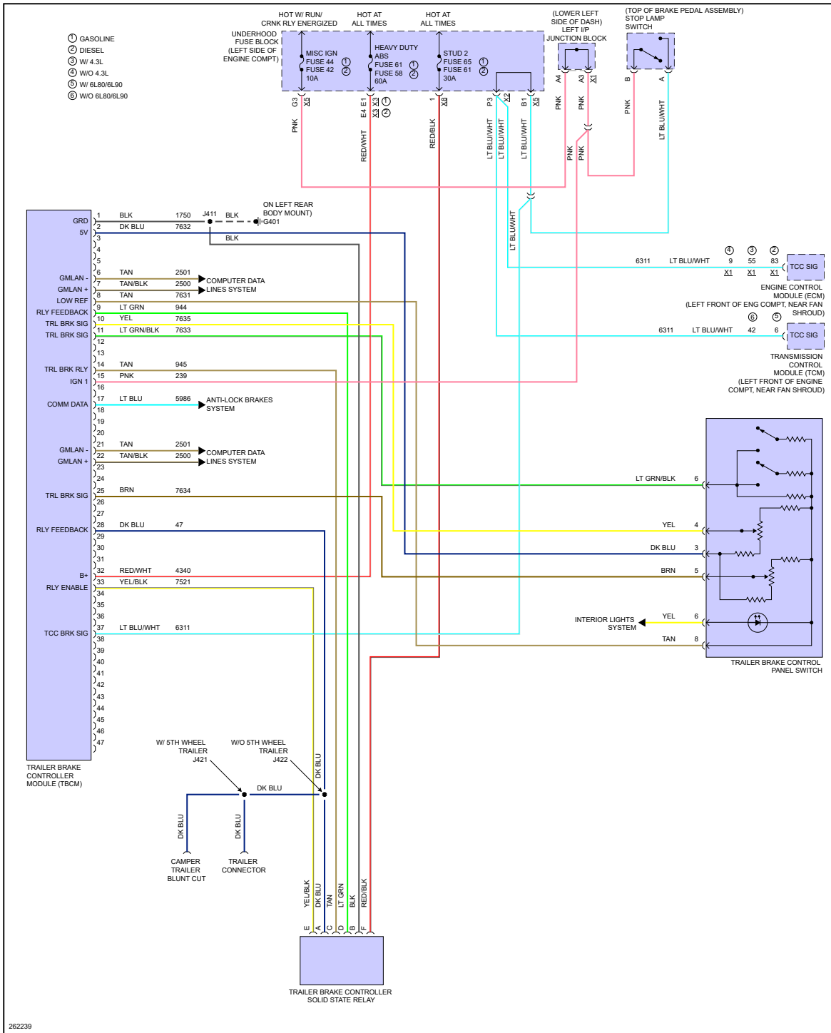
Fig 4: Trailer ABS Circuit
