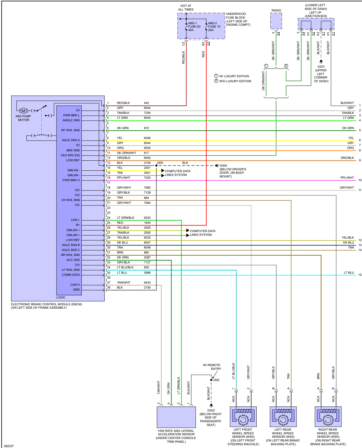
Fig 1: Anti-Lock Brake Circuit, W/ JL4 (1 of 2)
