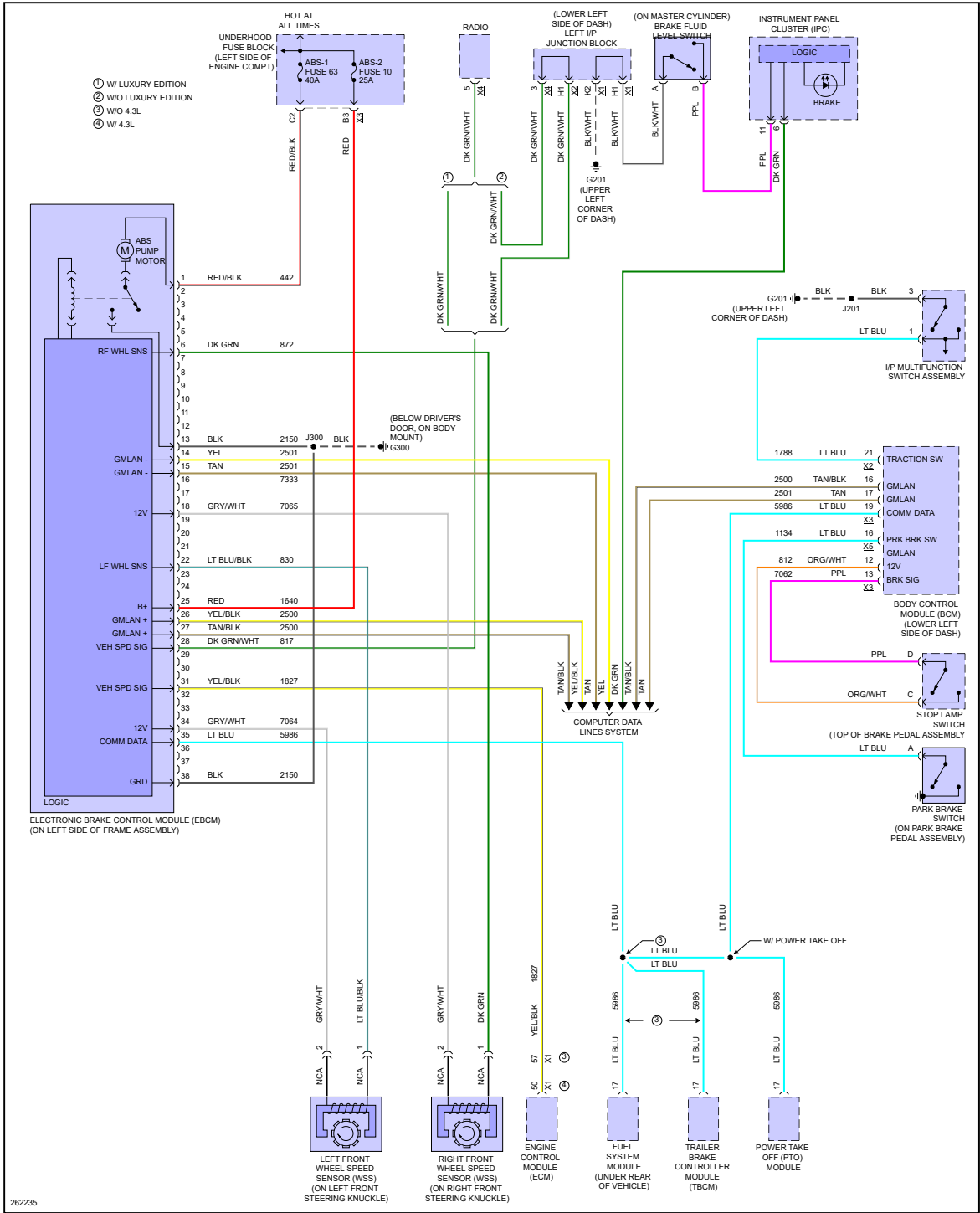
Fig 3: Anti-Lock Brake Circuit, W/O JL4
