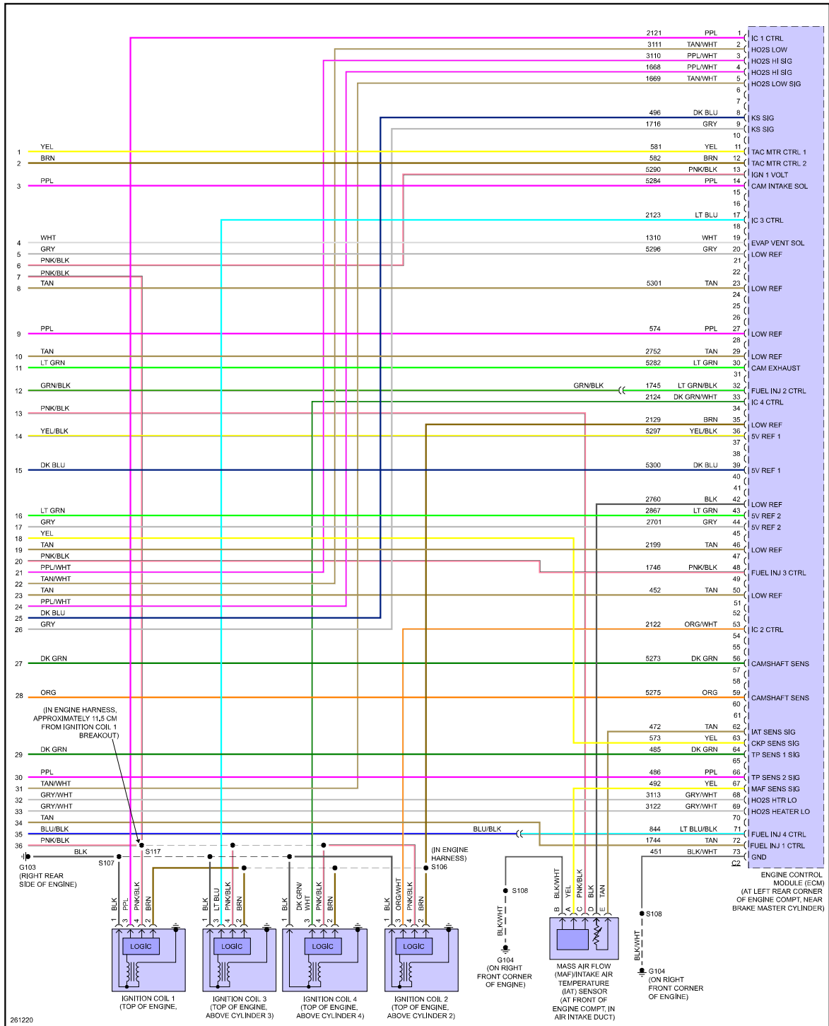
Fig 4: 2.4L VIN B, Engine Performance Circuit (4 of 4)
