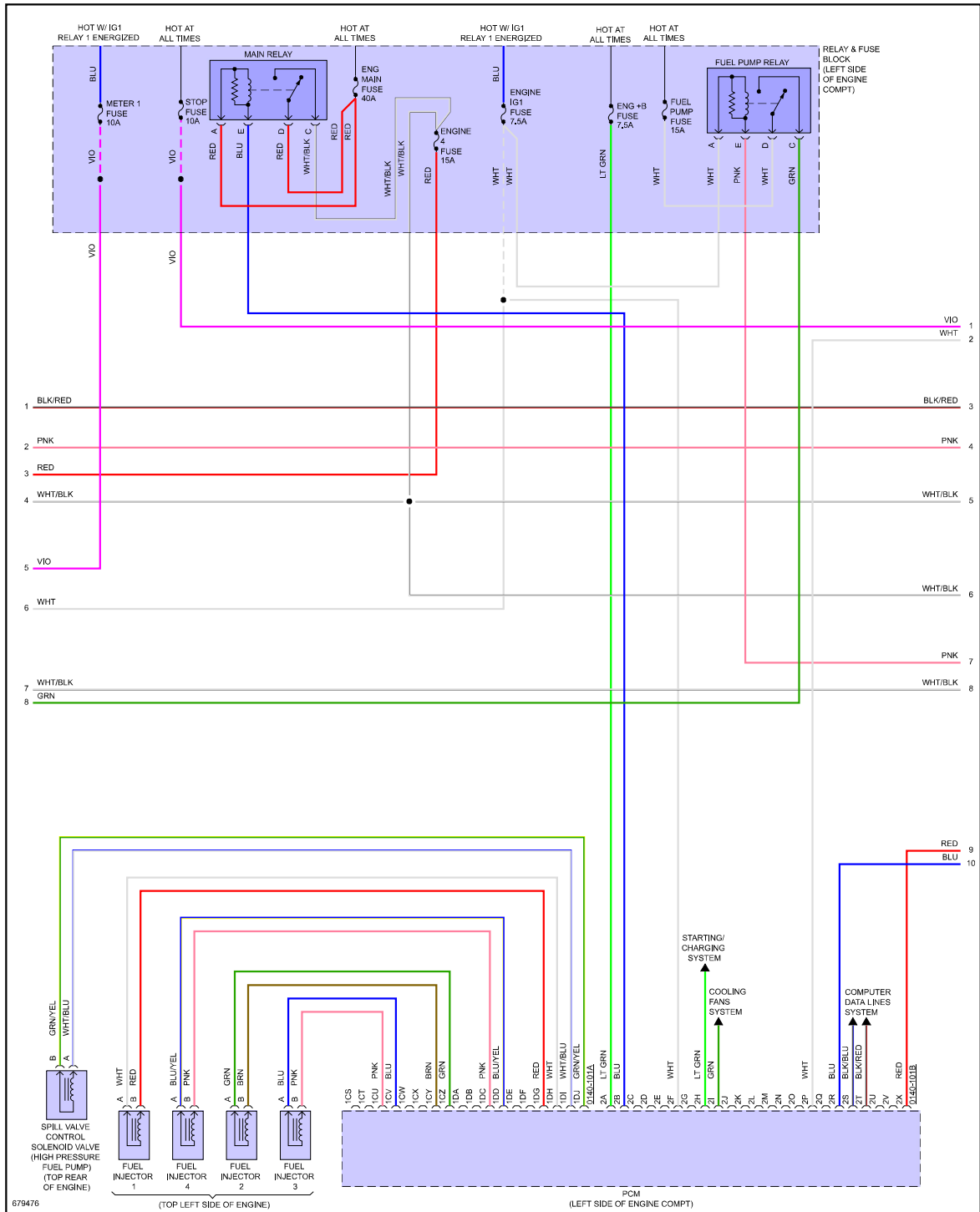
Fig 4: 2.0L SKYACTIV, Engine Performance Circuit (4 of 5)
