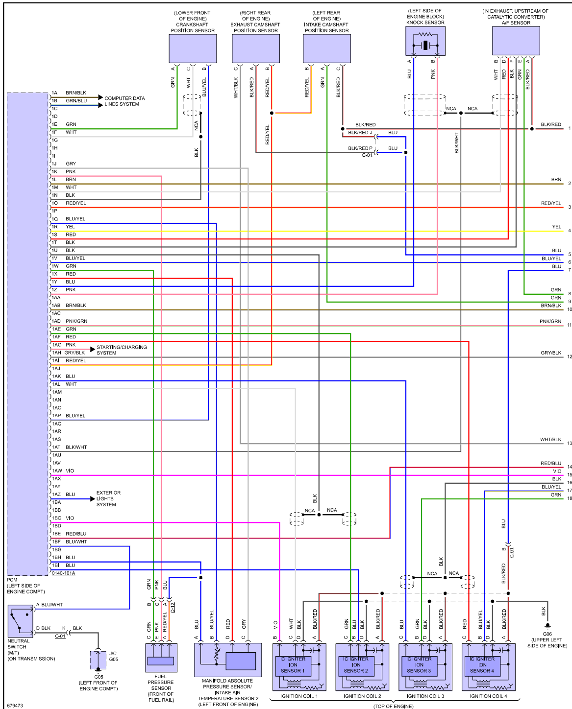
Fig 1: 2.0L SKYACTIV, Engine Performance Circuit (1 of 5)
