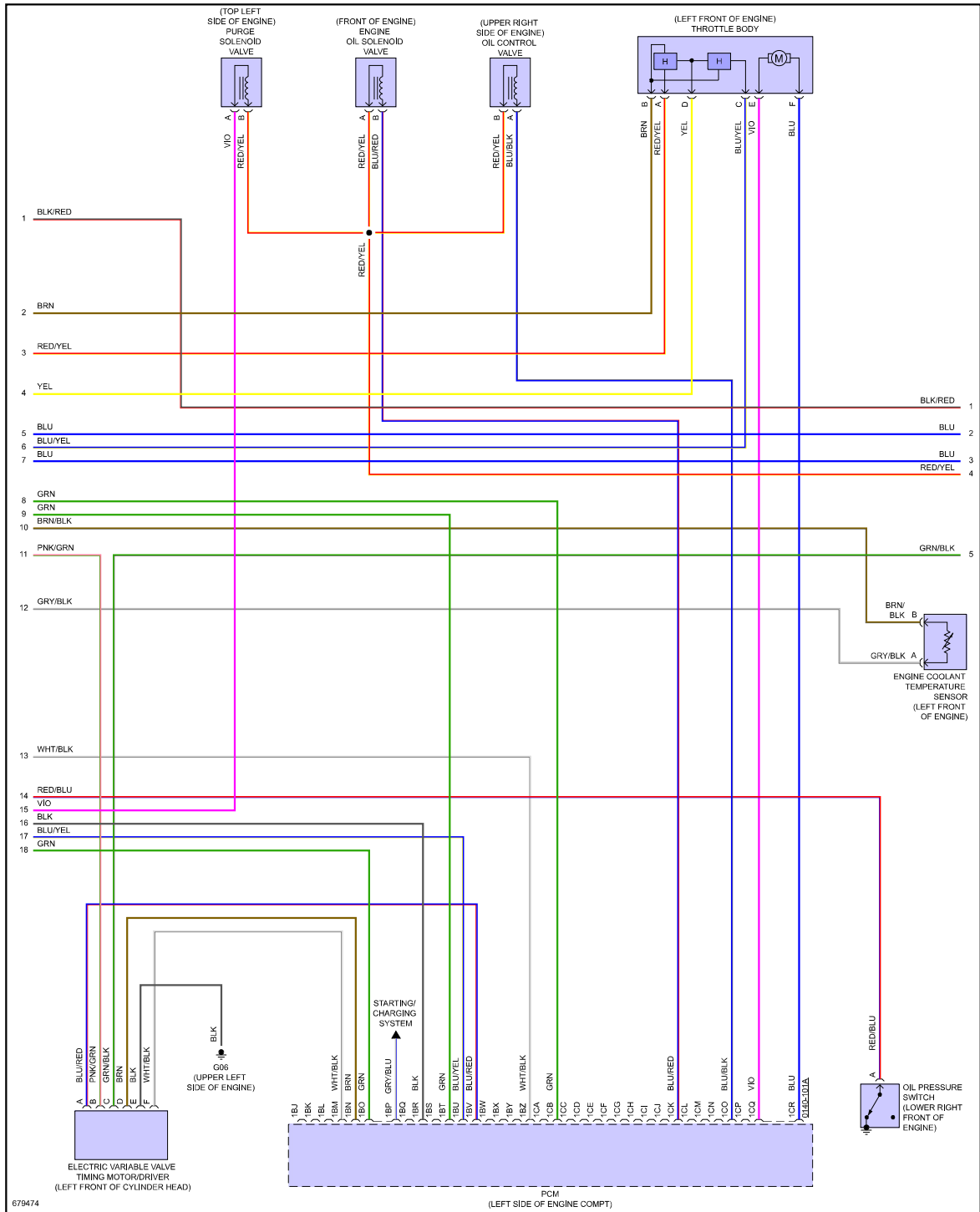
Fig 2: 2.0L SKYACTIV, Engine Performance Circuit (2 of 5)
