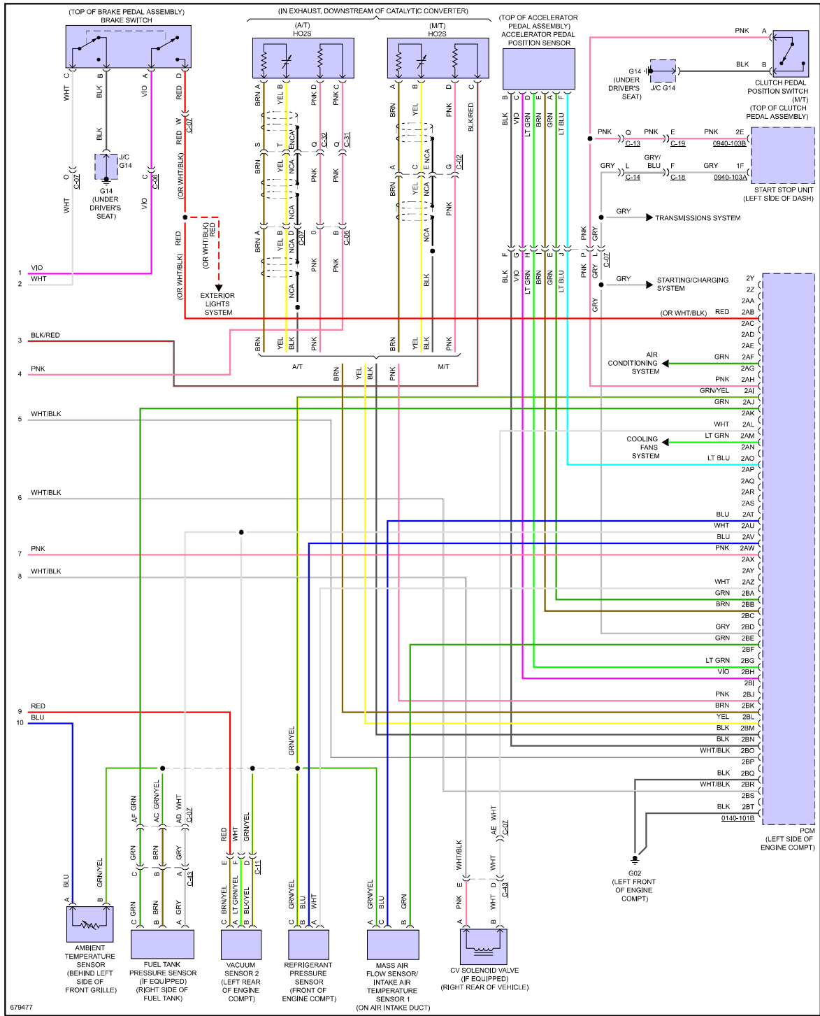
Fig 5: 2.0L SKYACTIV, Engine Performance Circuit (5 of 5)
