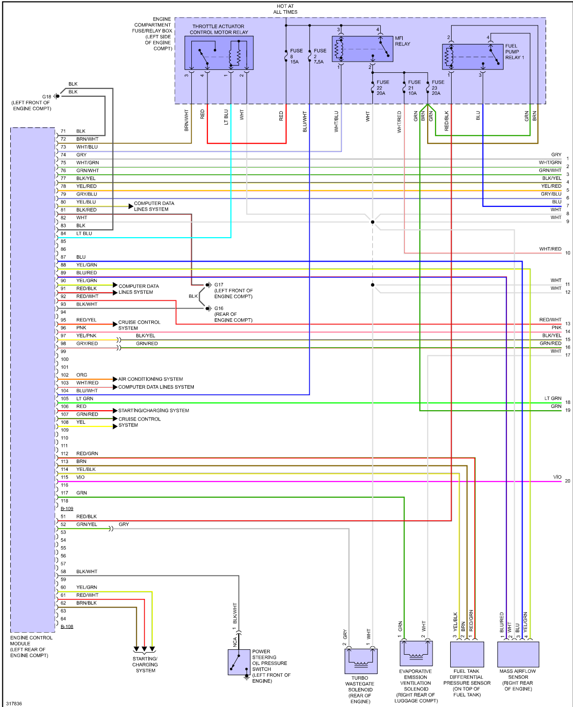
Fig 1: 2.0L Turbo, Engine Performance Circuit (1 of 4)
