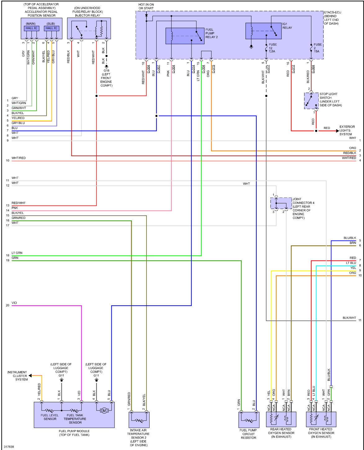
Fig 2: 2.0L Turbo, Engine Performance Circuit (2 of 4)
