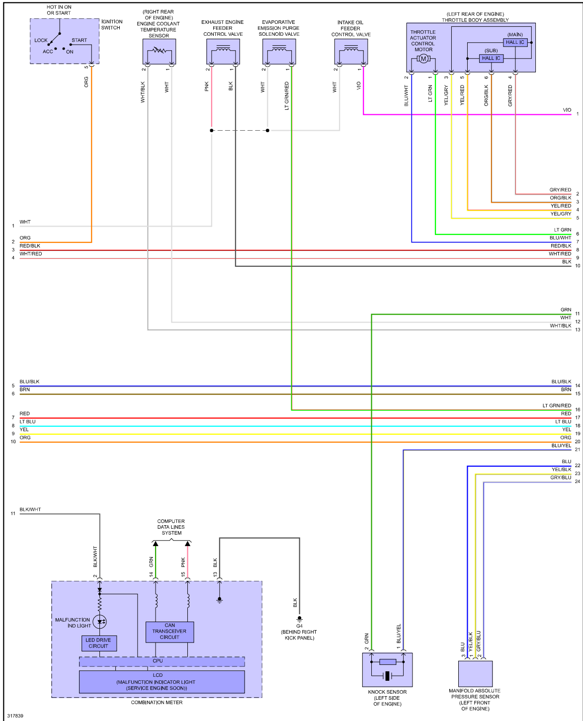
Fig 3: 2.0L Turbo, Engine Performance Circuit (3 of 4)
