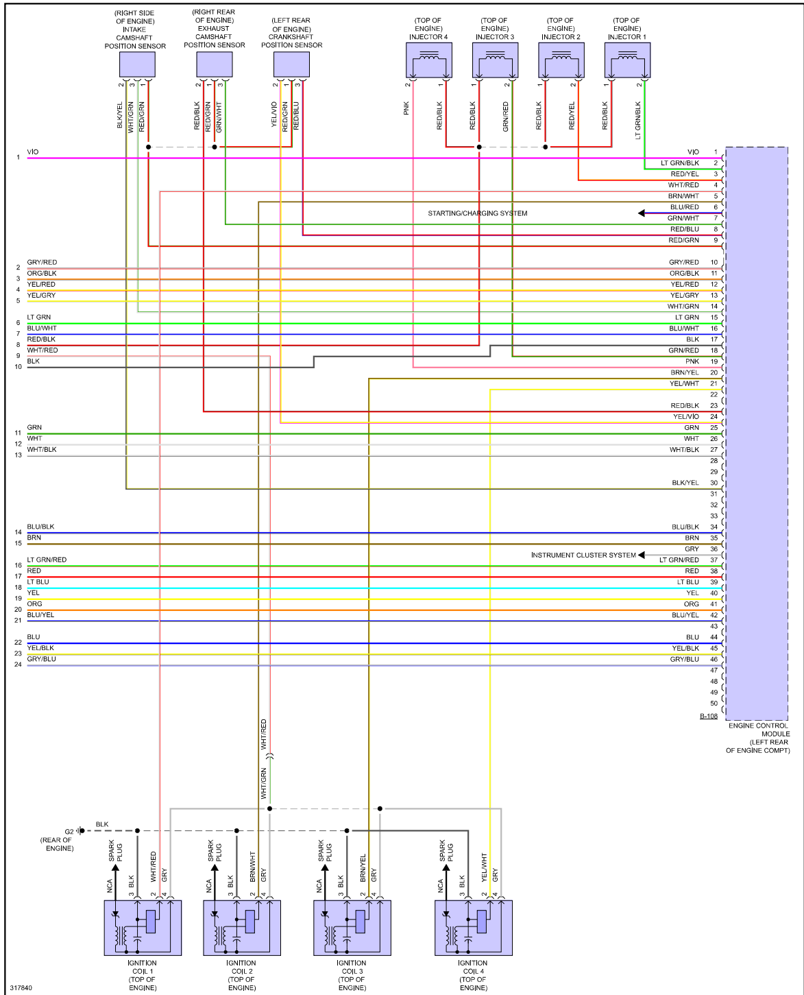
Fig 4: 2.0L Turbo, Engine Performance Circuit (4 of 4)
