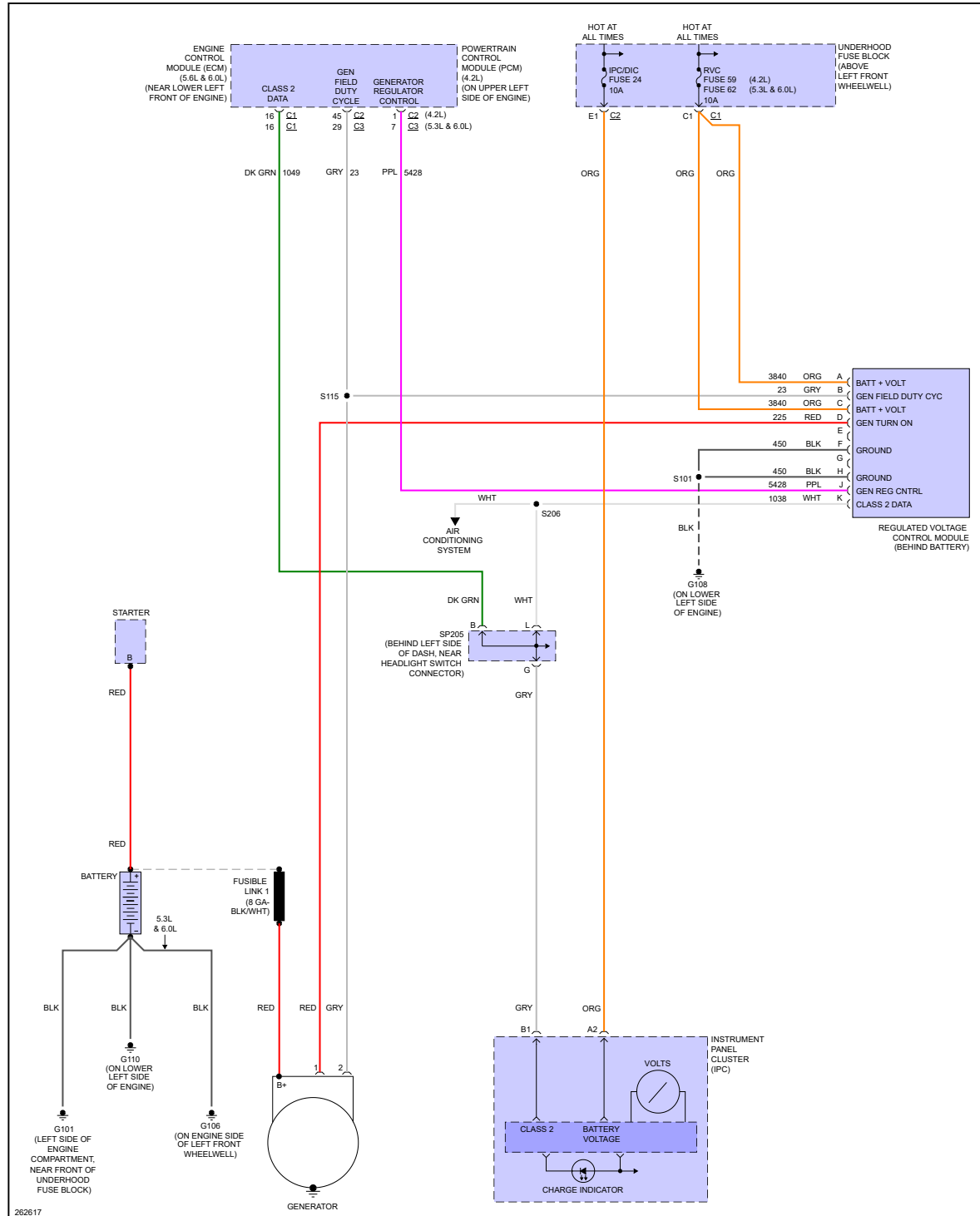
Fig 1: Charging Circuit
