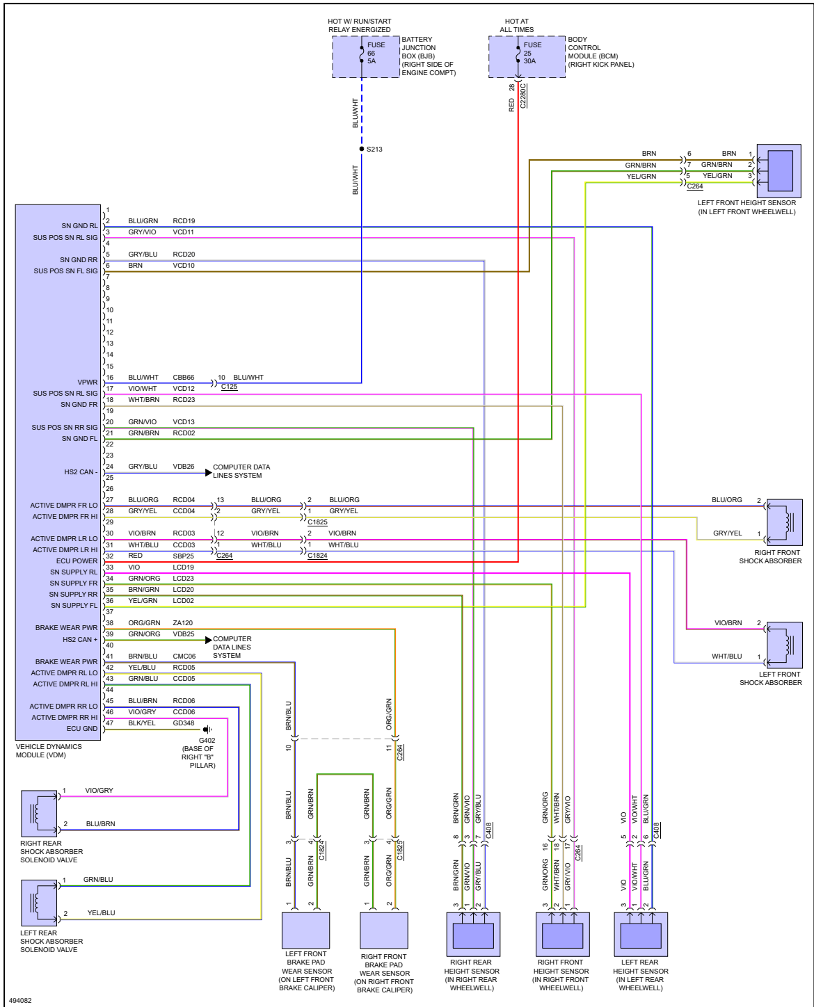
Fig 1: Electronic Suspension Circuit
