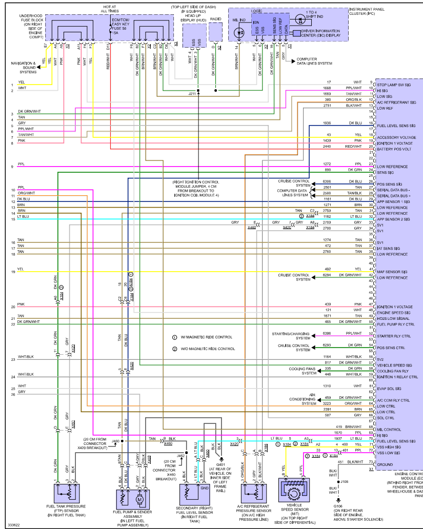
Fig 4: 7.0L VIN E, Engine Performance Circuit (4 of 4)
