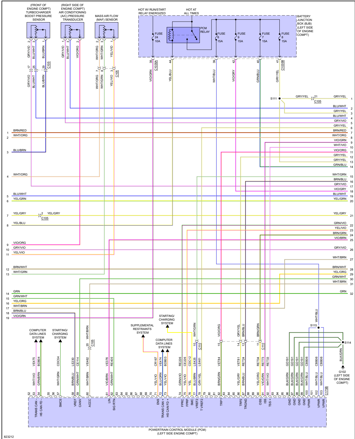
Fig 2: 1.5L Turbo, Engine Performance Circuit (2 of 8)
