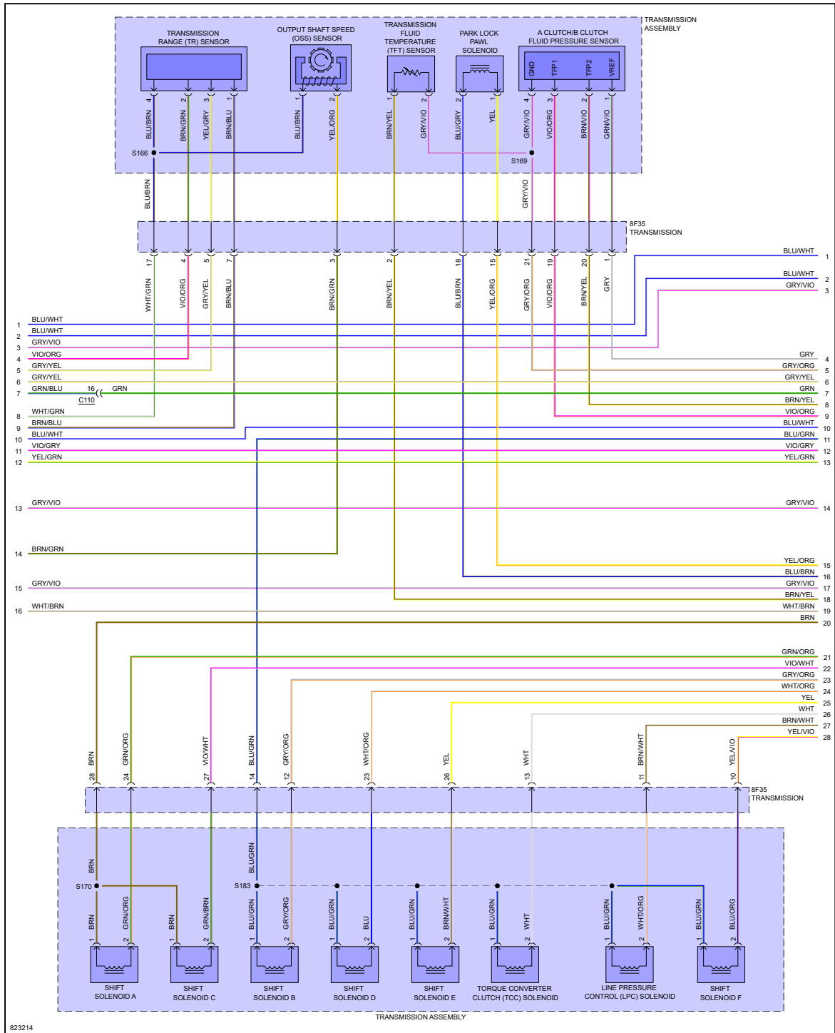
Fig 4: 1.5L Turbo, Engine Performance Circuit (4 of 8)
