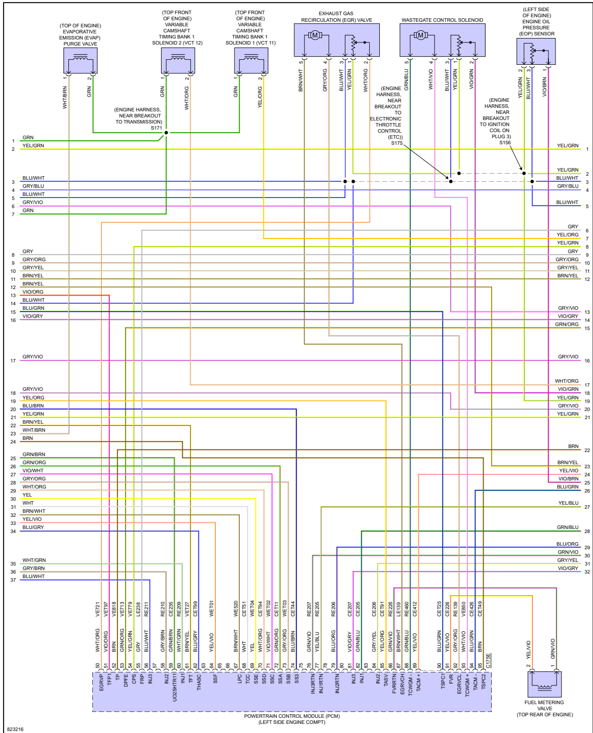
Fig 6: 1.5L Turbo, Engine Performance Circuit (6 of 8)
