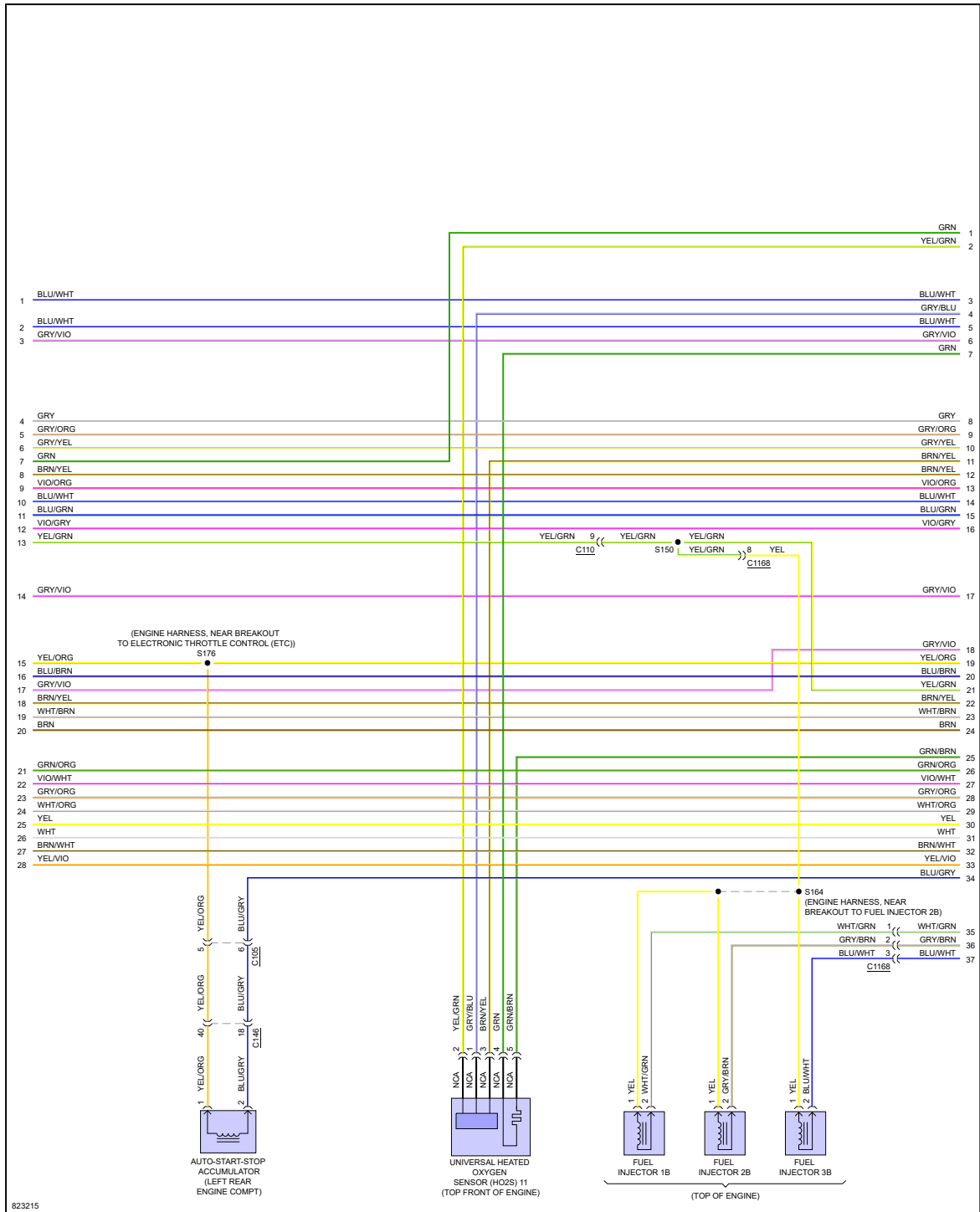
Fig 5: 1.5L Turbo, Engine Performance Circuit (5 of 8)
