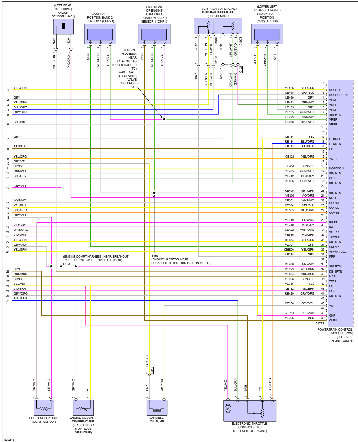
Fig 8: 1.5L Turbo, Engine Performance Circuit (8 of 8)
