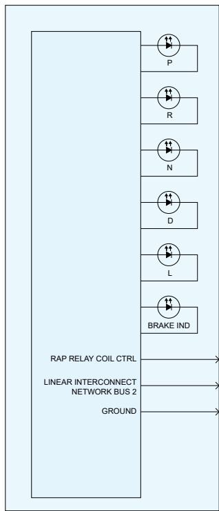
TRANSMISSION SHIFT LEVER POSITION INDICATOR
