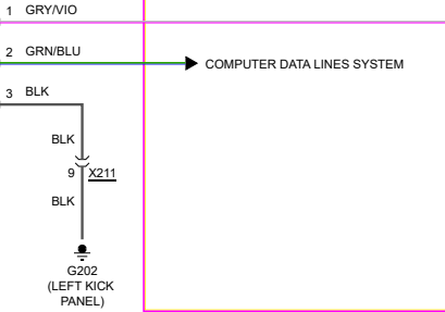
TRANSMISSION SHIFT LEVER POSITION INDICATOR
