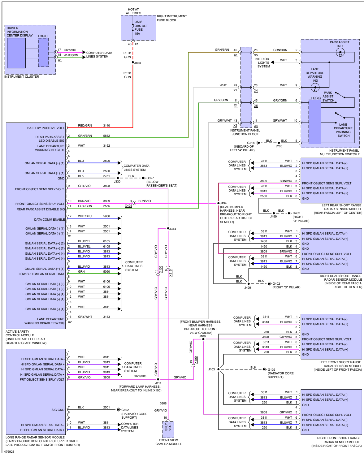
Fig 1: Collision Avoidance Circuit
