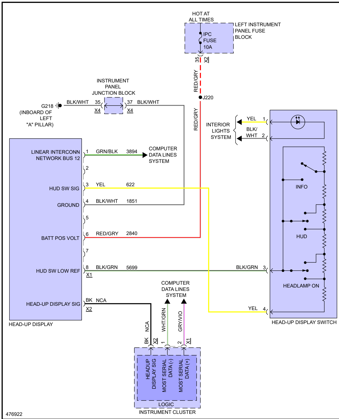
Fig 2: Head-Up Display Circuit
