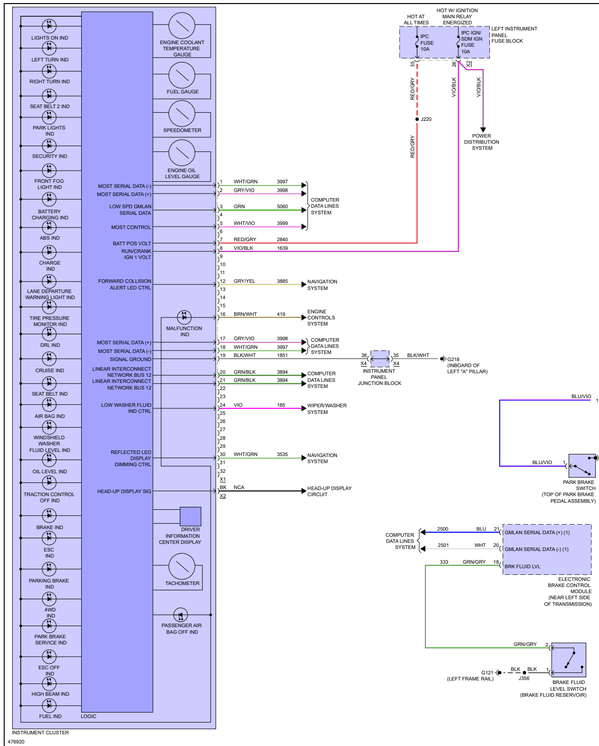
Fig 3: Instrument Cluster Circuit (1 of 2)
