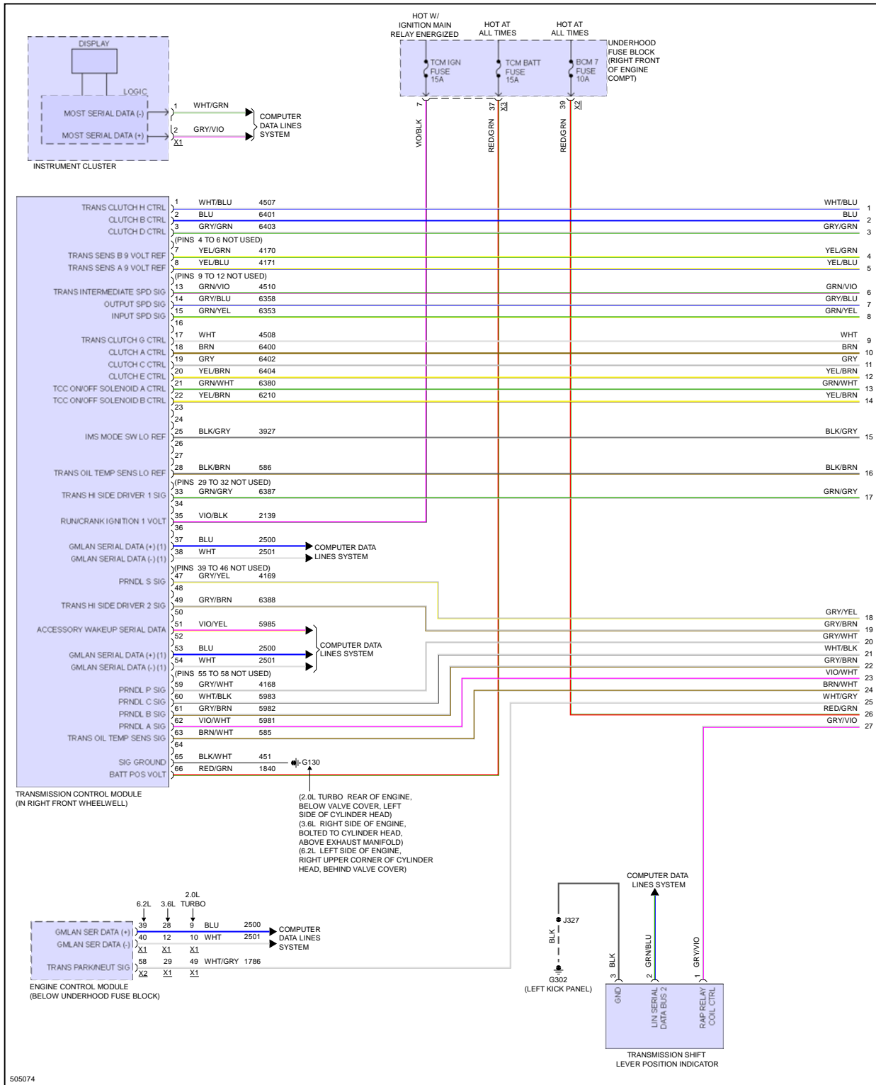
Fig 1: Transmission Circuit (1 of 3)
