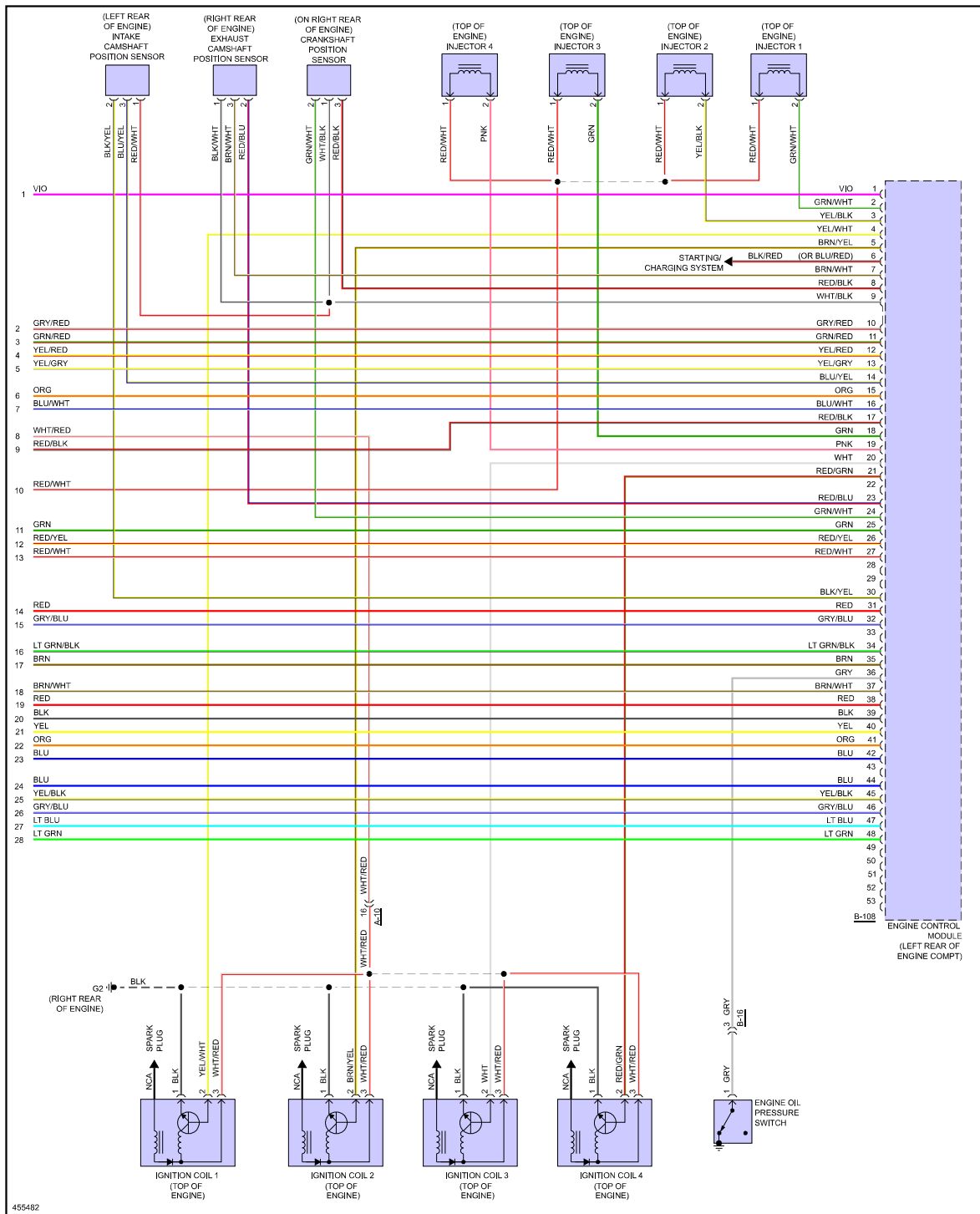
Fig 4: 2.4L, Engine Performance Circuit (4 of 4)
