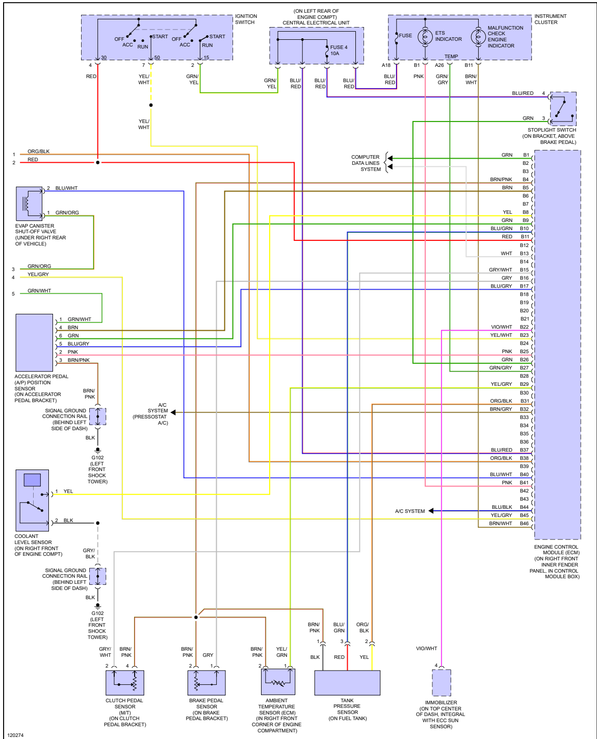
Fig 3: 2.3L Turbo, Engine Performance Circuit (3 of 3)
