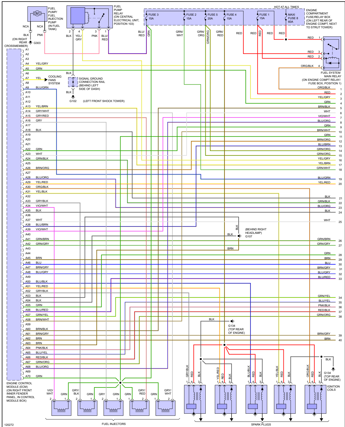
Fig 1: 2.3L Turbo, Engine Performance Circuit (1 of 3)
