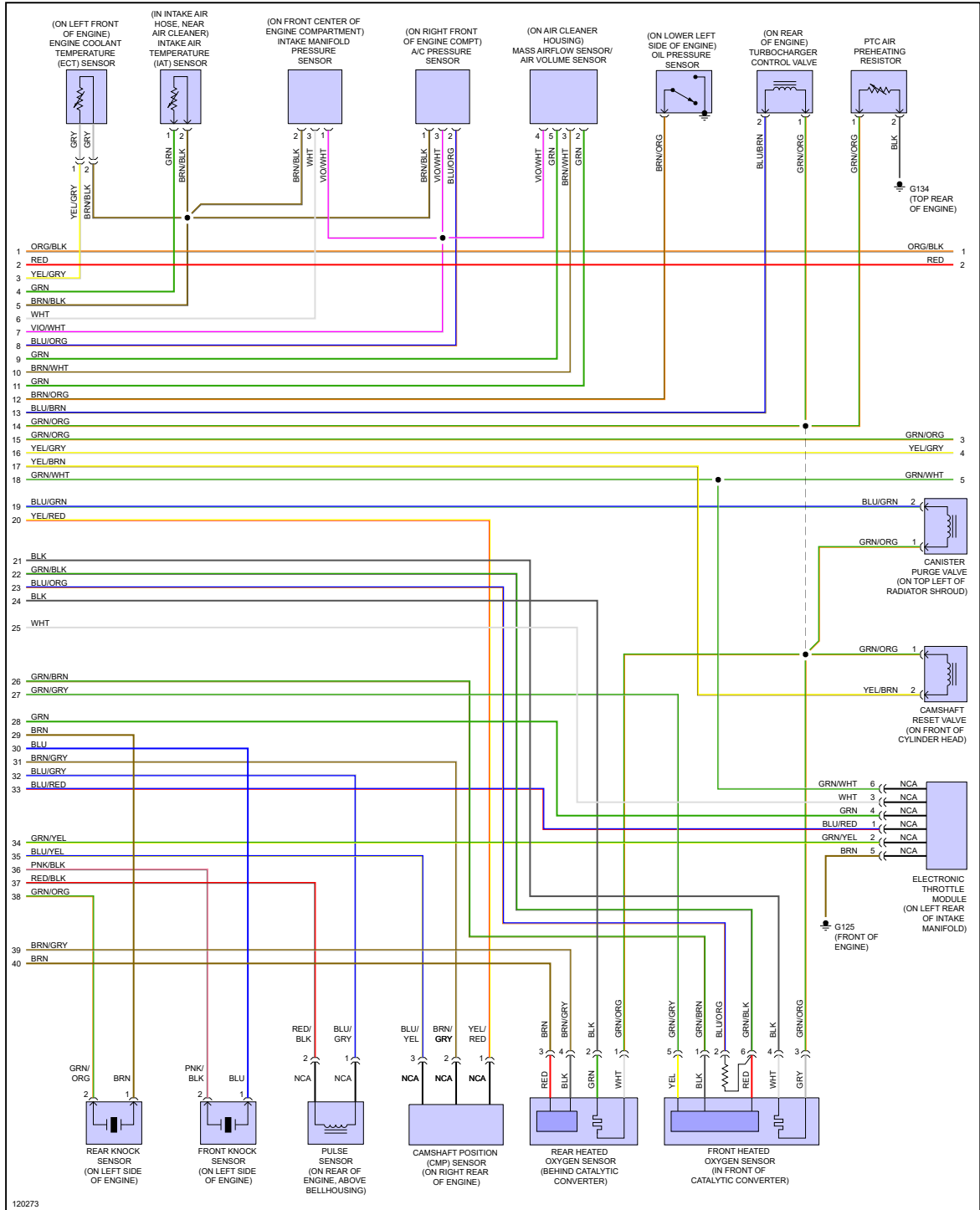
Fig 2: 2.3L Turbo, Engine Performance Circuit (2 of 3)
