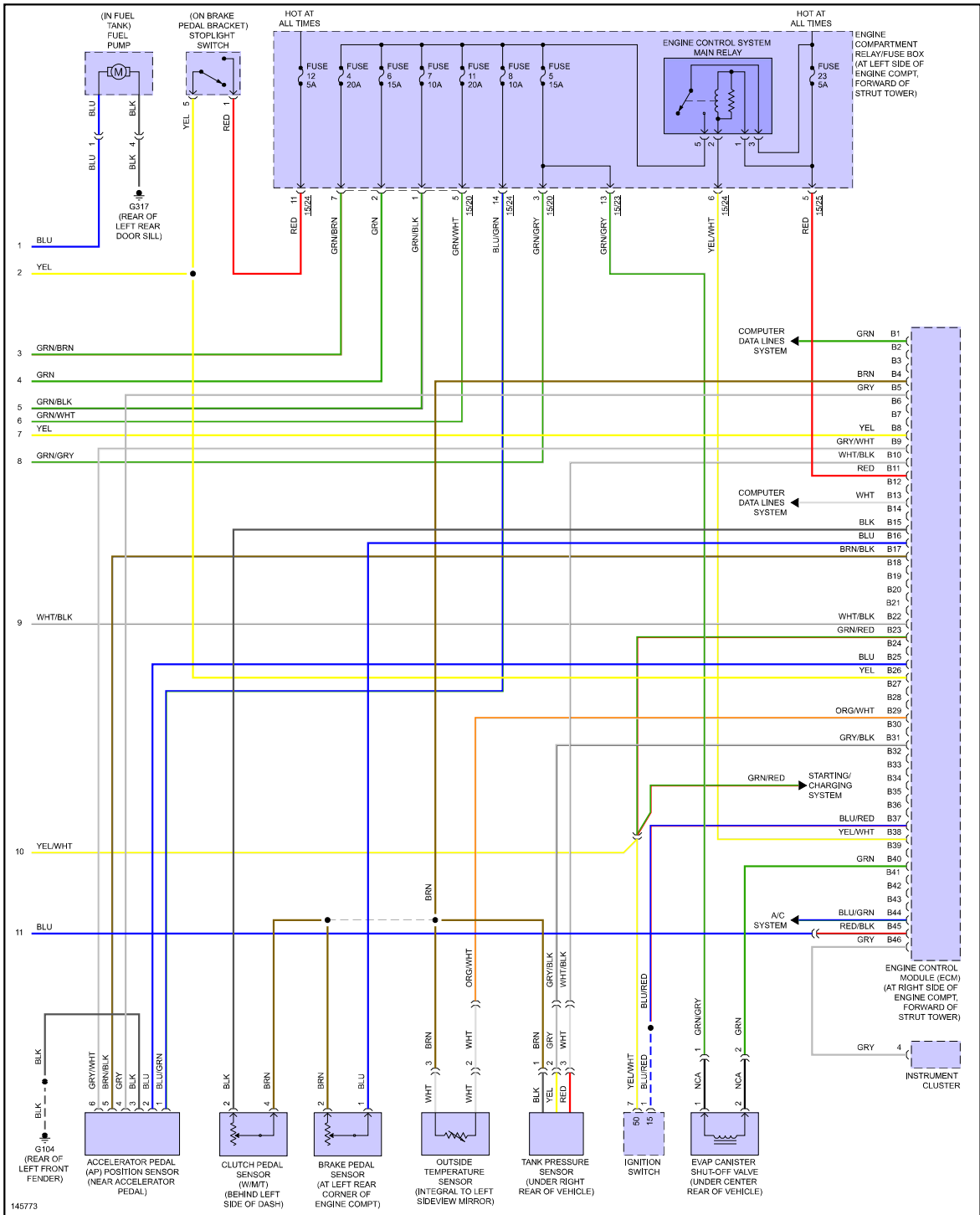
Fig 6: 2.4L, Engine Performance Circuits (3 of 3)
