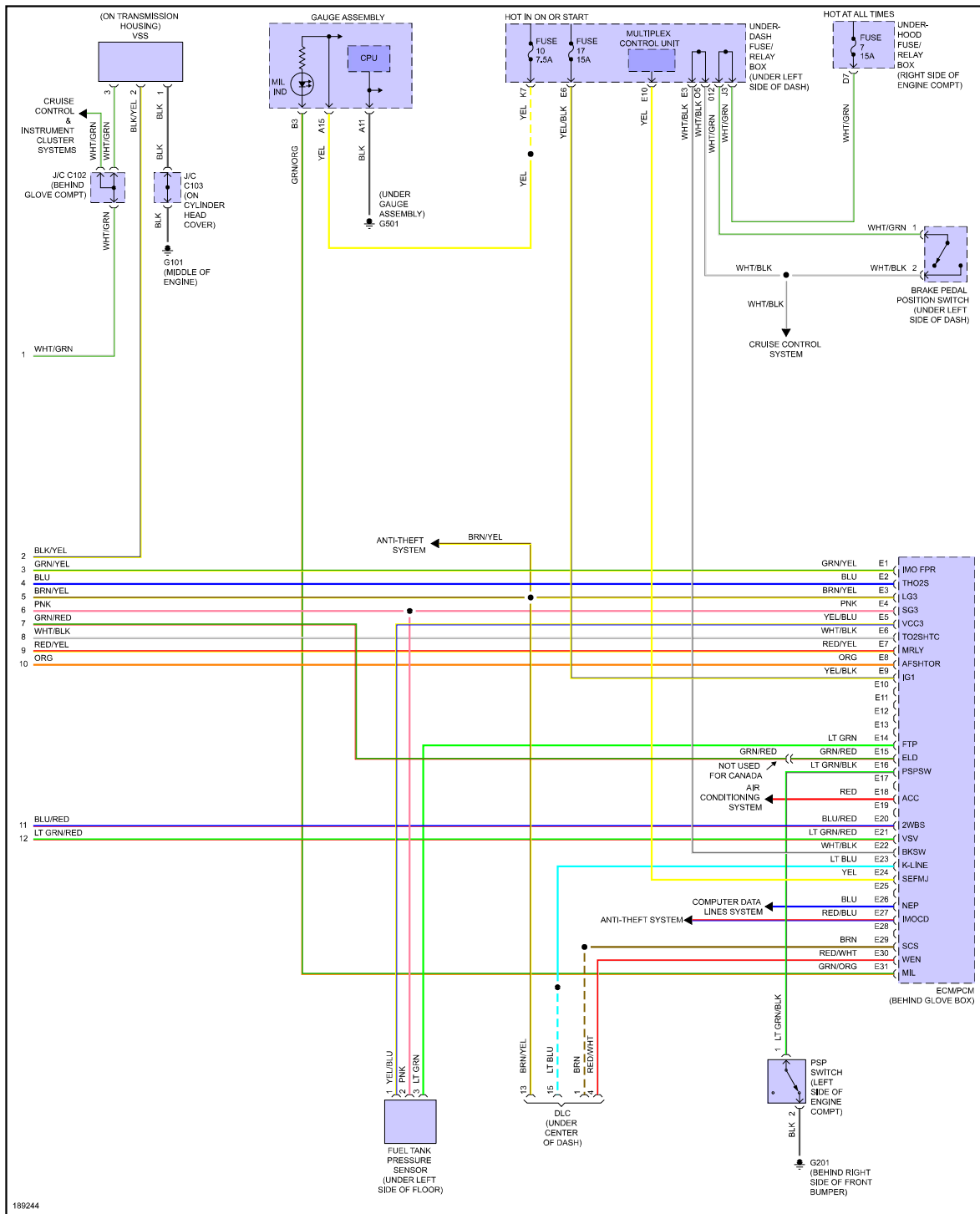
Fig 12: 1.7L, Engine Performance Circuit, HX M/T (3 of 3)
