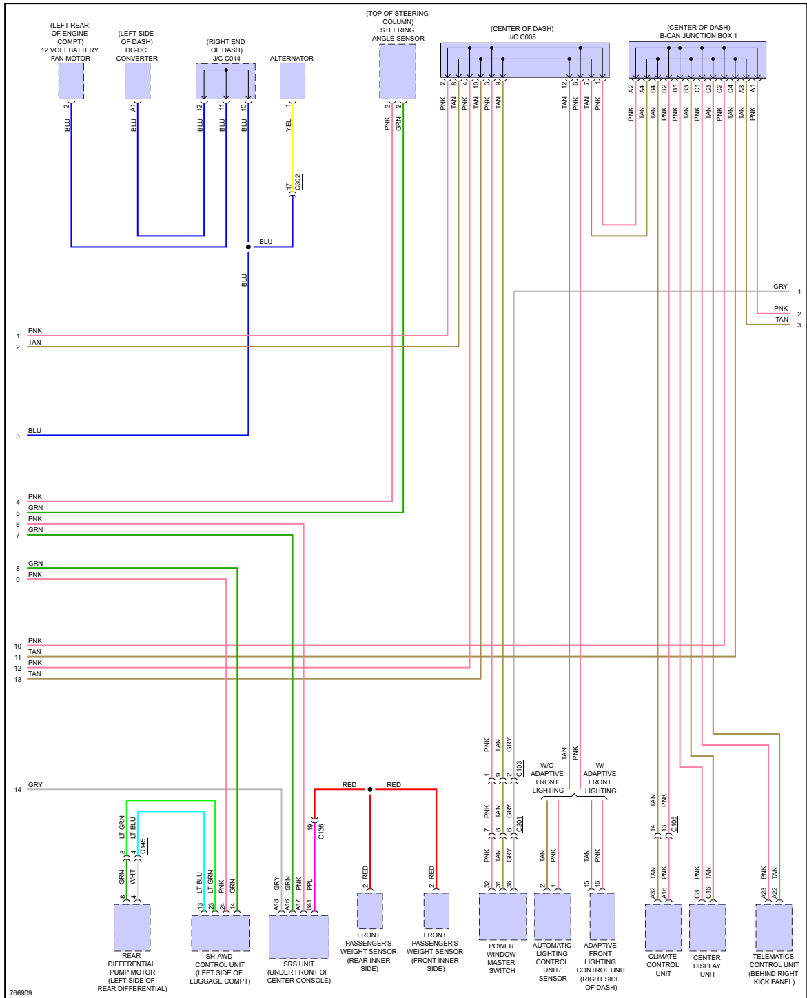
Fig 4: Computer Data Lines Circuit (4 of 5)
