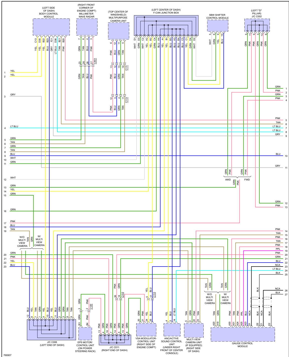
Fig 2: Computer Data Lines Circuit (2 of 5)
