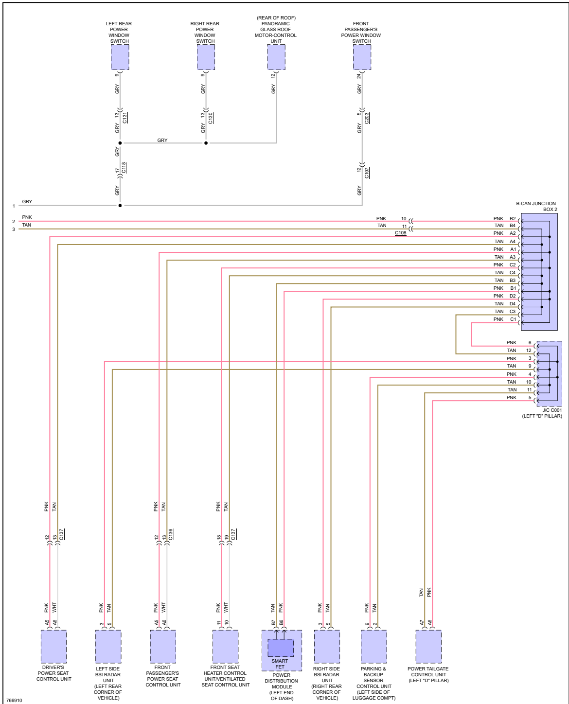
Fig 5: Computer Data Lines Circuit (5 of 5)
