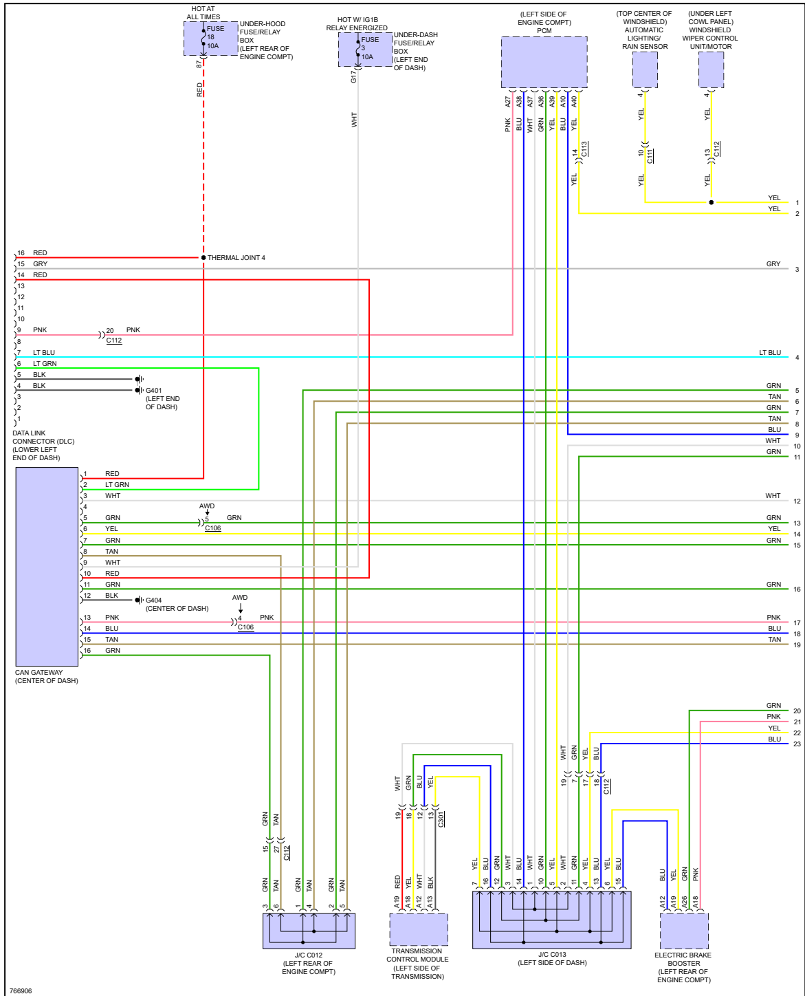
Fig 1: Computer Data Lines Circuit (1 of 5)
