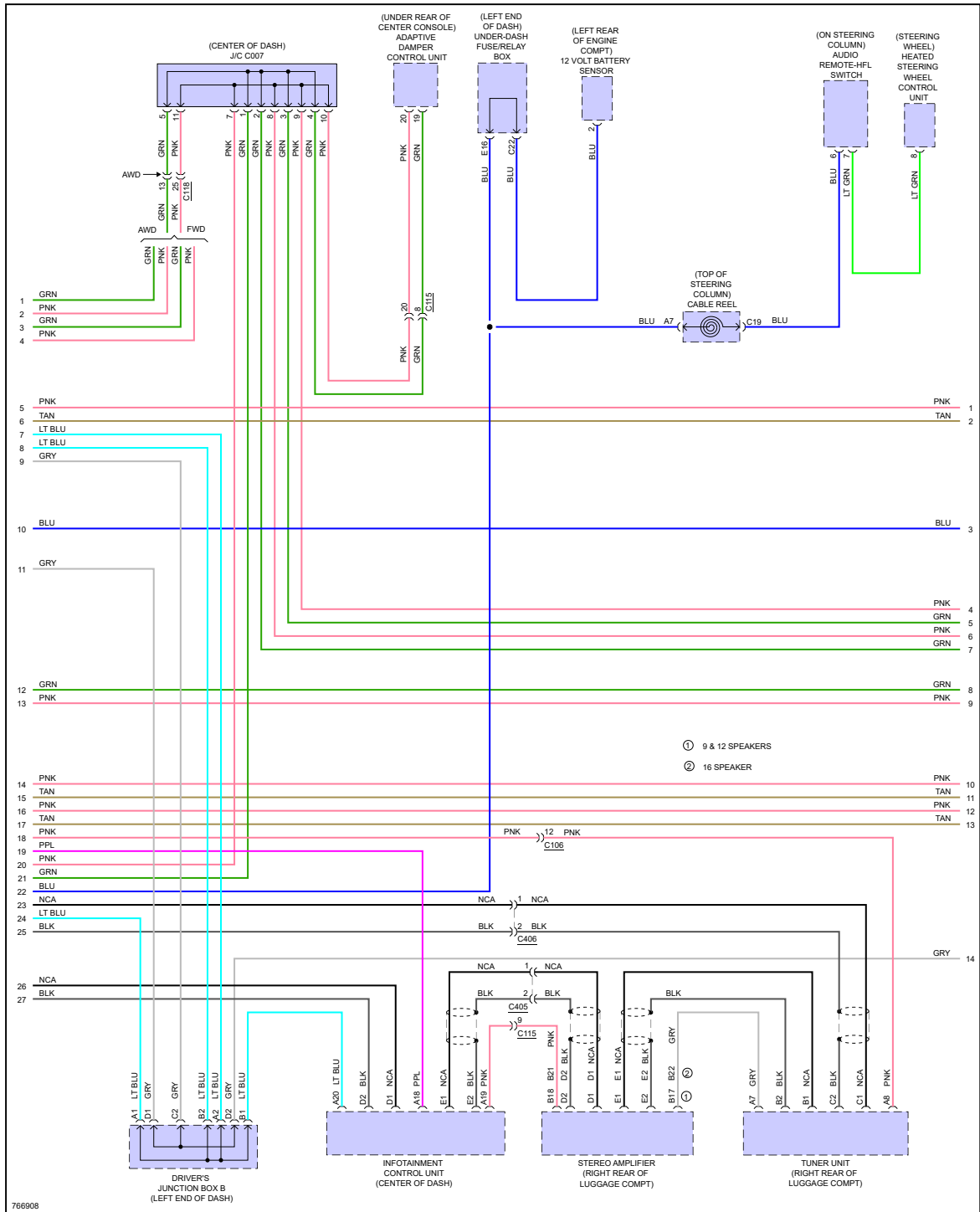
Fig 3: Computer Data Lines Circuit (3 of 5)
