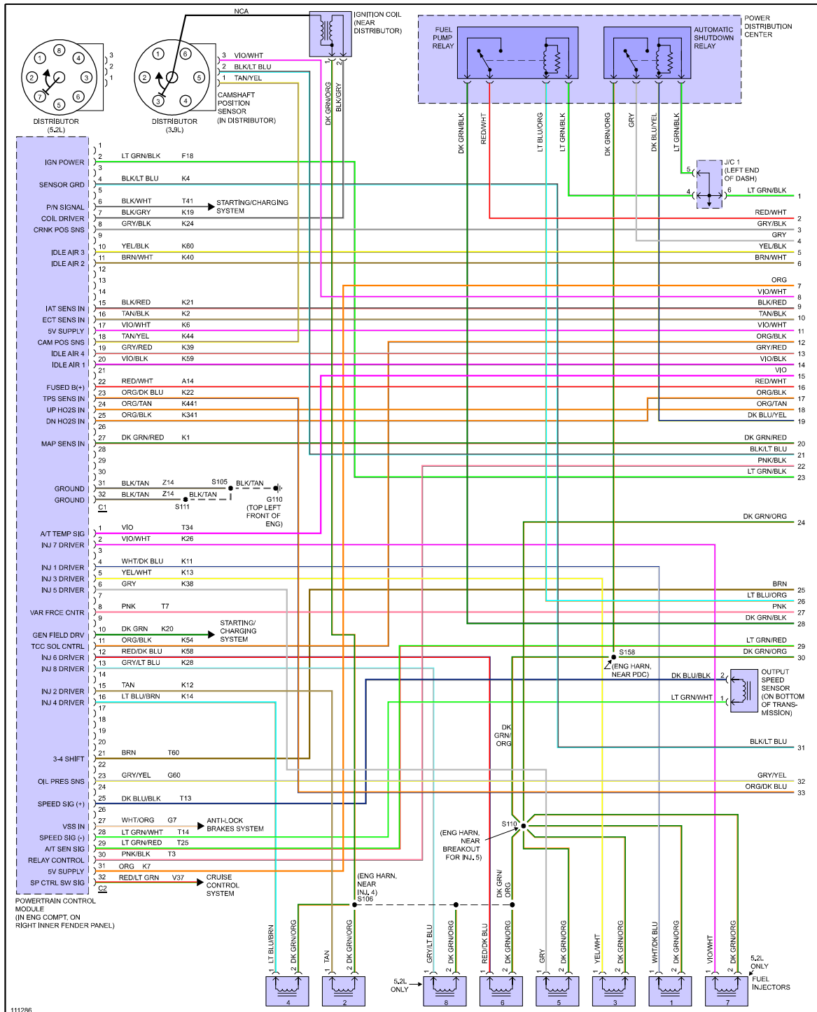
Fig 1: 3.9L, Engine Performance Circuits (1 of 3)
