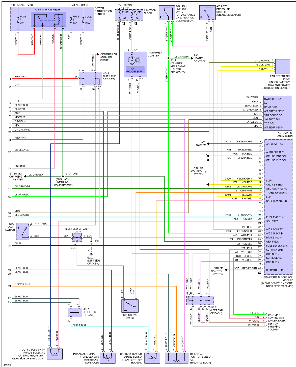
Fig 3: 3.9L, Engine Performance Circuits (3 of 3)
