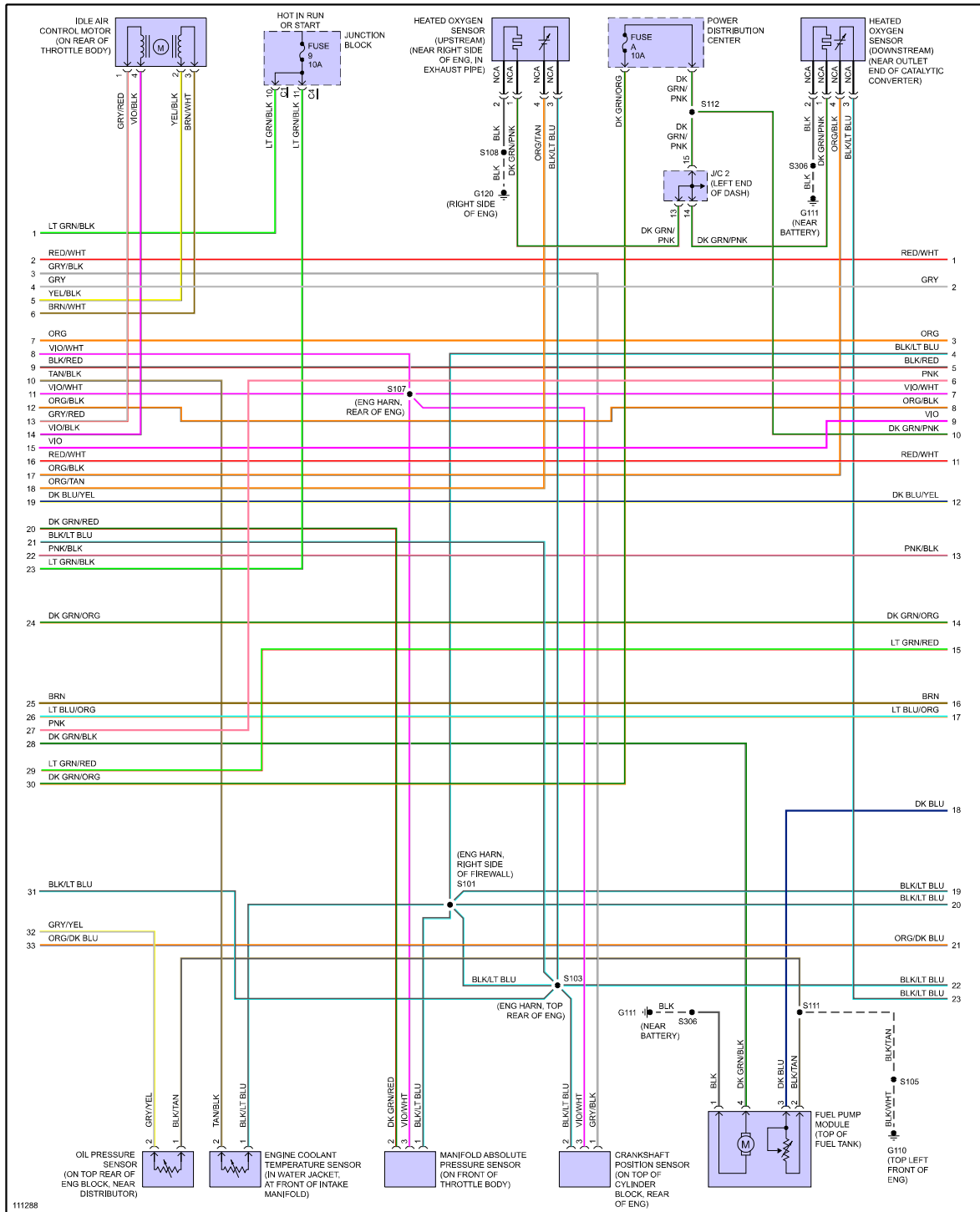
Fig 2: 3.9L, Engine Performance Circuits (2 of 3)
