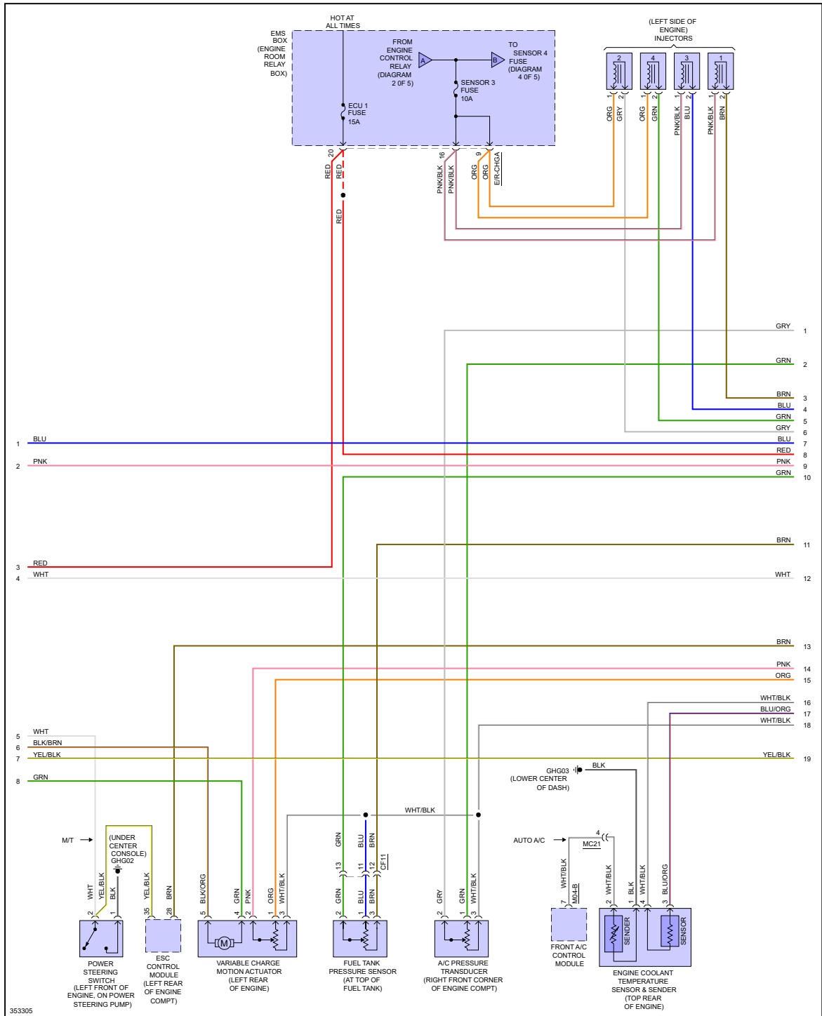
Fig 3: 2.4L, Engine Performance Circuit (3 of 5)
