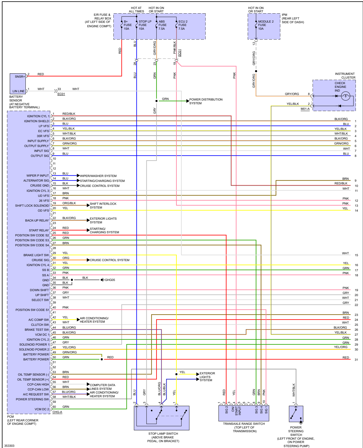
Fig 1: 2.4L, Engine Performance Circuit (1 of 5)
