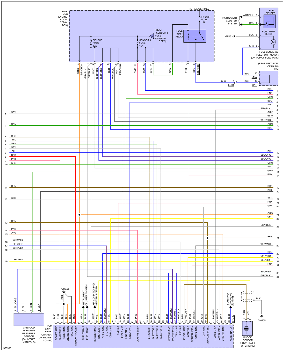
Fig 4: 2.4L, Engine Performance Circuit (4 of 5)
