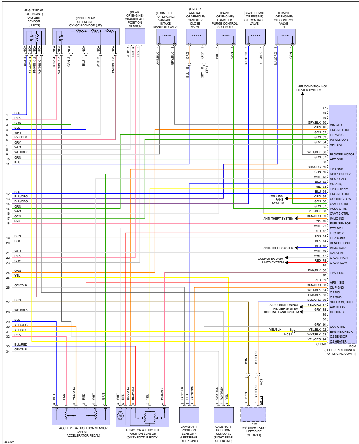
Fig 5: 2.4L, Engine Performance Circuit (5 of 5)
