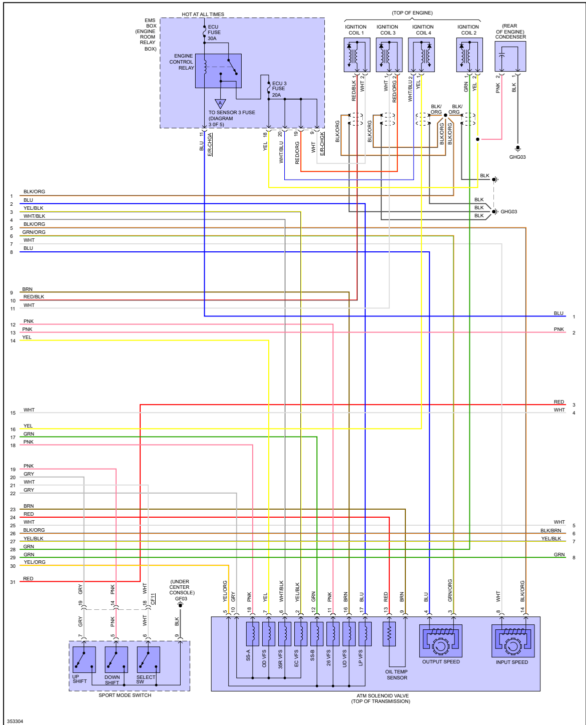
Fig 2: 2.4L, Engine Performance Circuit (2 of 5)
