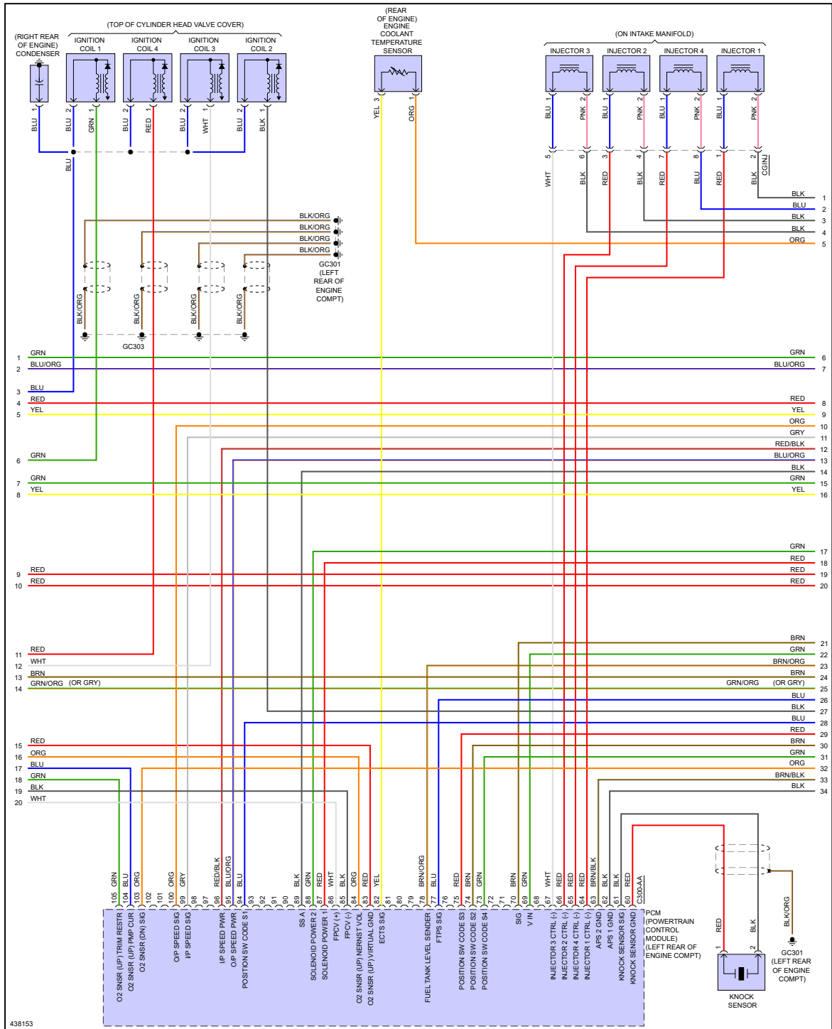
Fig 4: 2.0L, MFI Control Circuit (3 of 7)
