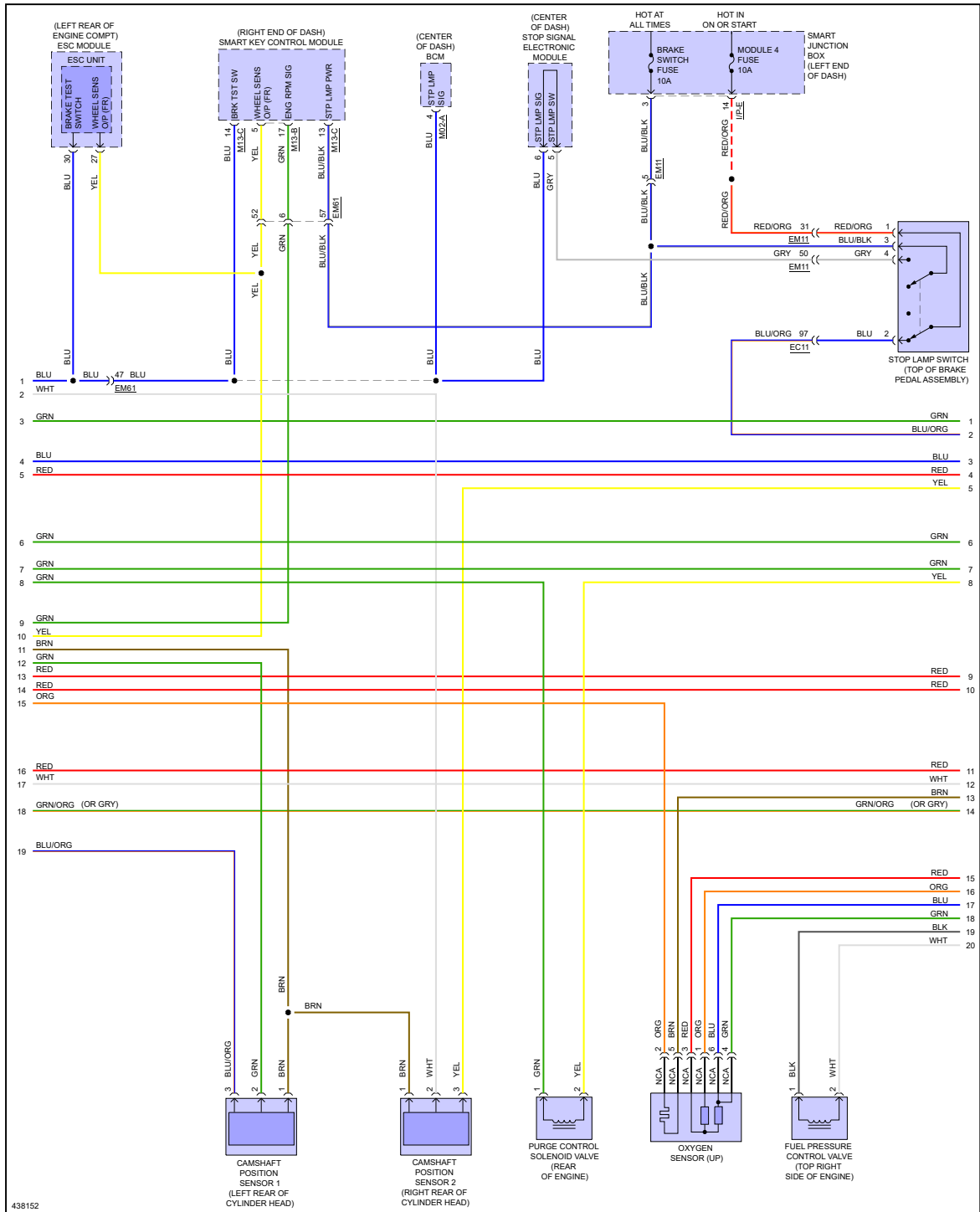
Fig 3: 2.0L, MFI Control Circuit (2 of 7)
