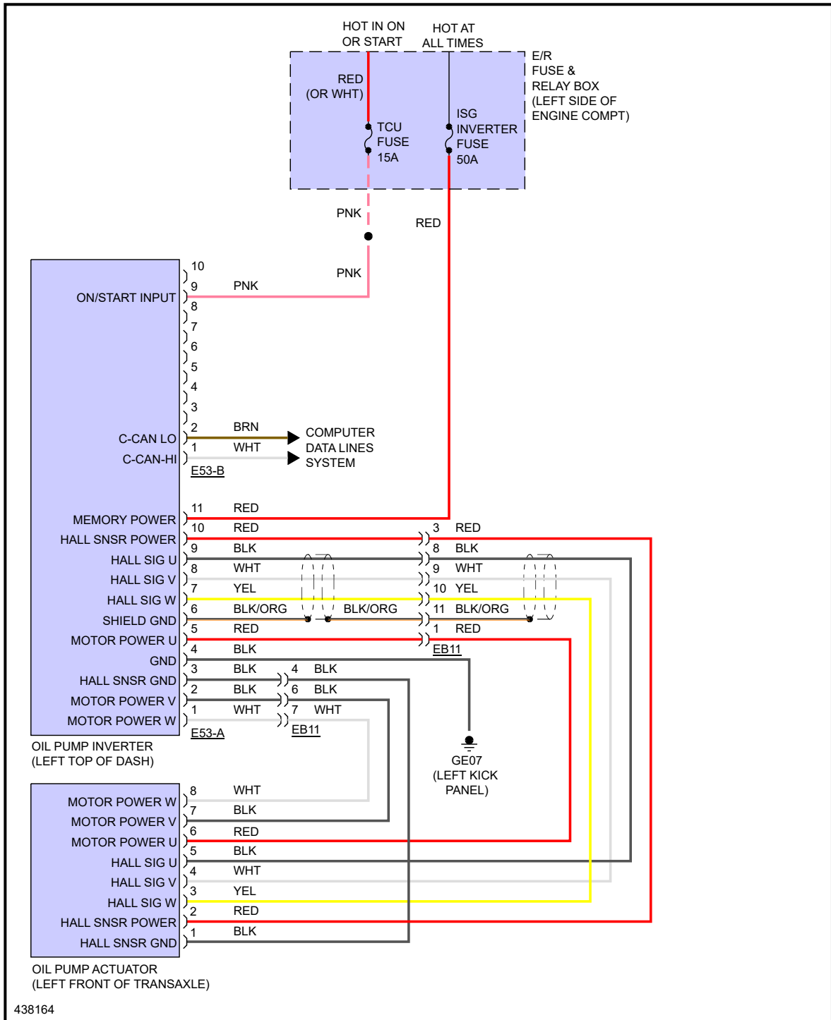
Fig 1: 2.0L, Electric Oil Pump Circuit
