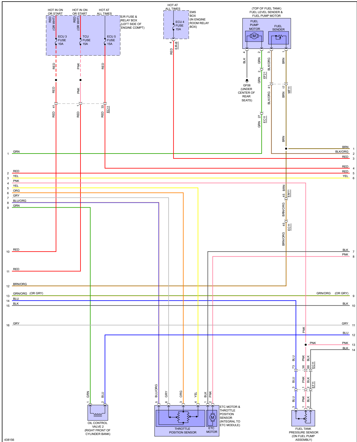
Fig 7: 2.0L, MFI Control Circuit (6 of 7)
