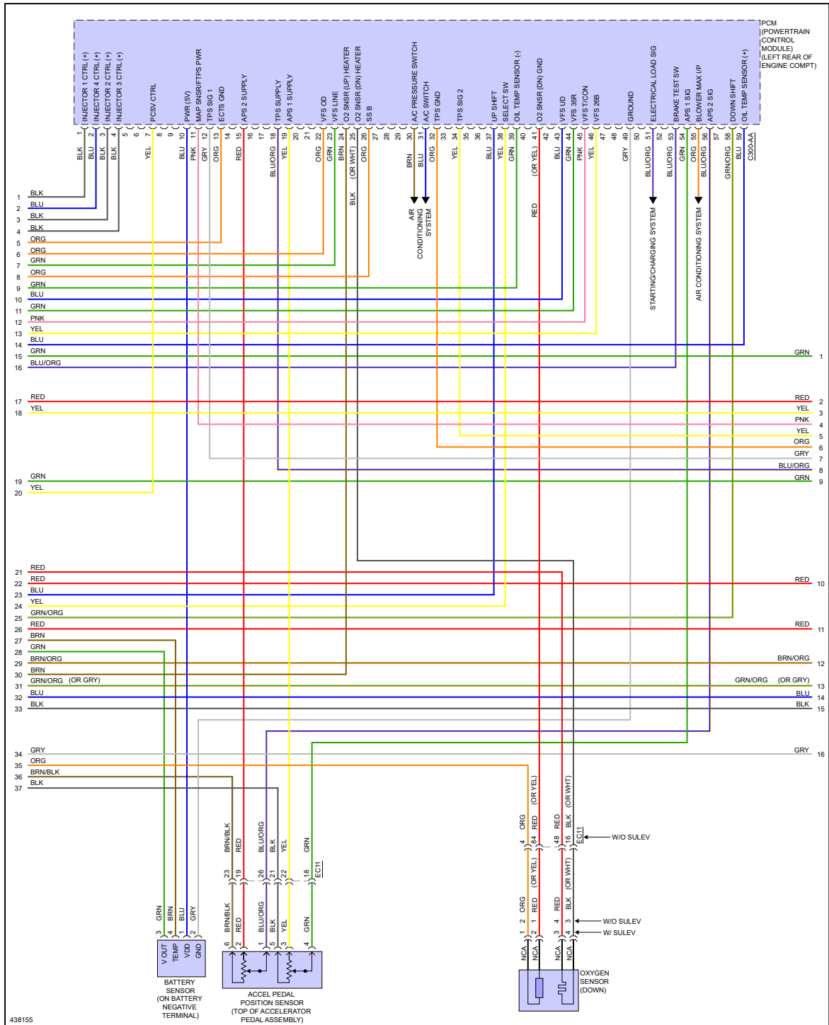
Fig 6: 2.0L, MFI Control Circuit (5 of 7)
