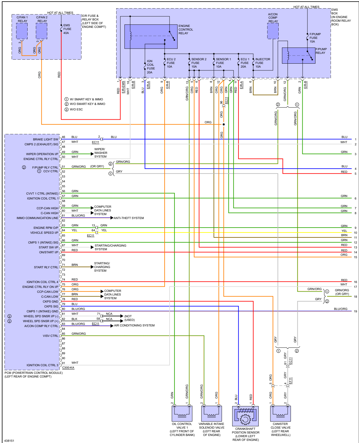
Fig 2: 2.0L, MFI Control Circuit (1 of 7)
