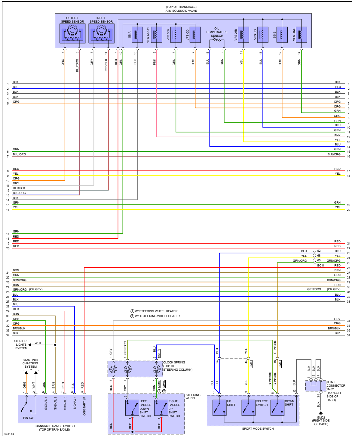
Fig 5: 2.0L, MFI Control Circuit (4 of 7)
