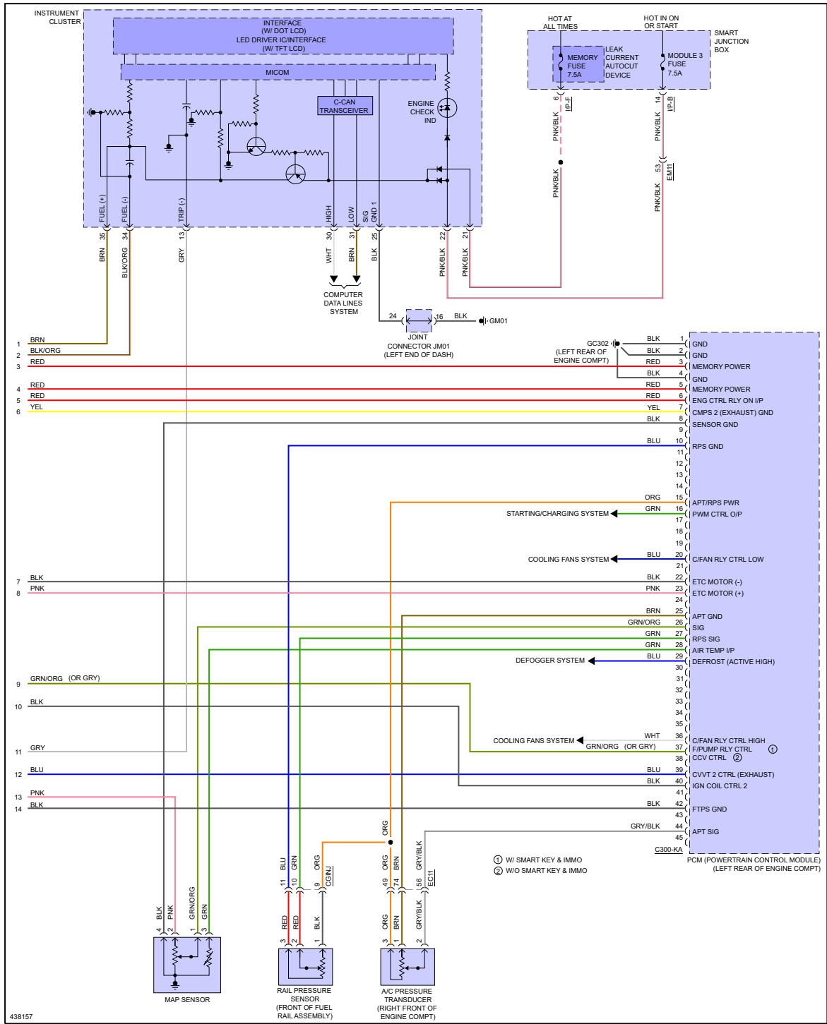
Fig 8: 2.0L, MFI Control Circuit (7 of 7)
