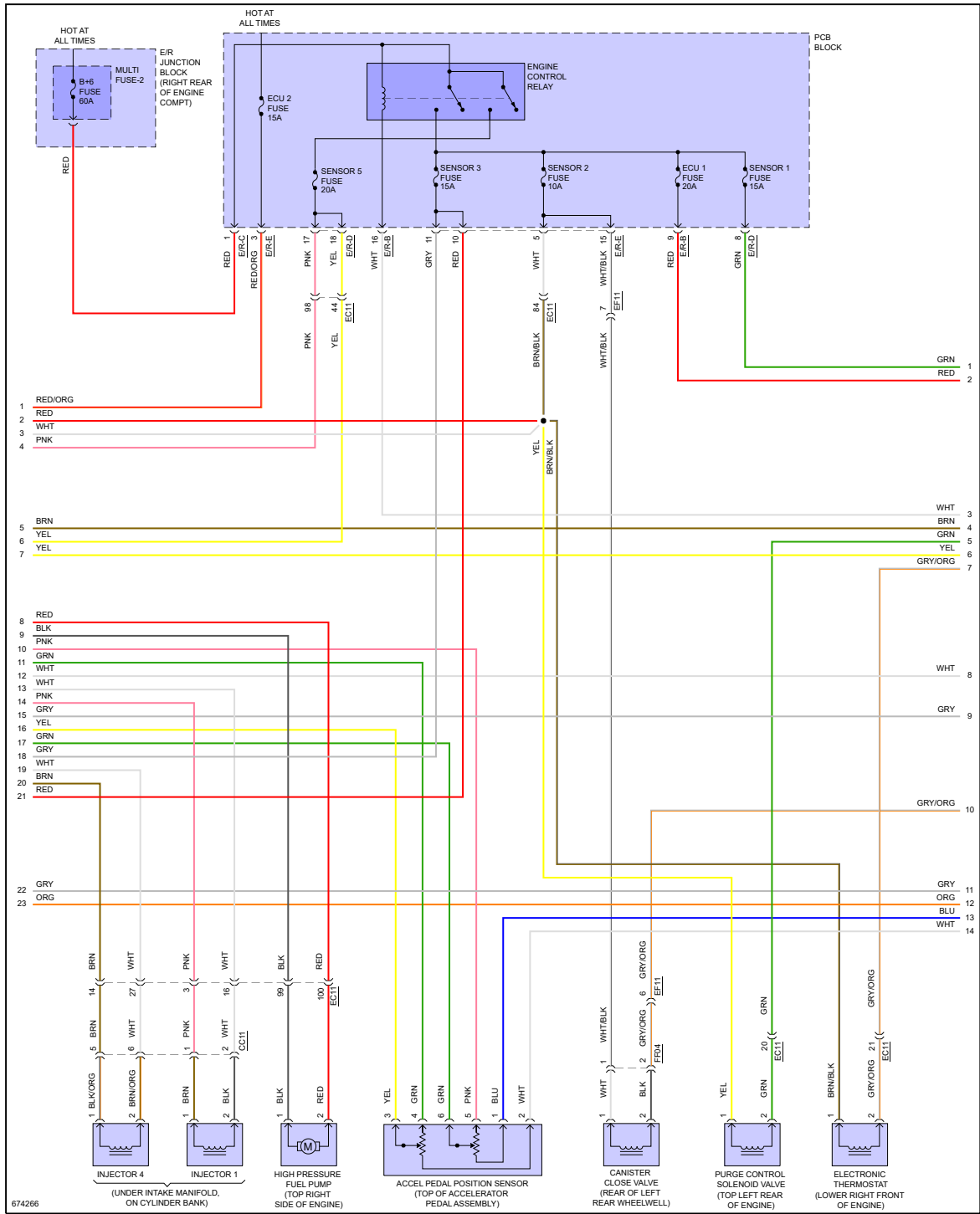
Fig 6: 2.0L Turbo, Engine Controls Circuit (5 of 7)
