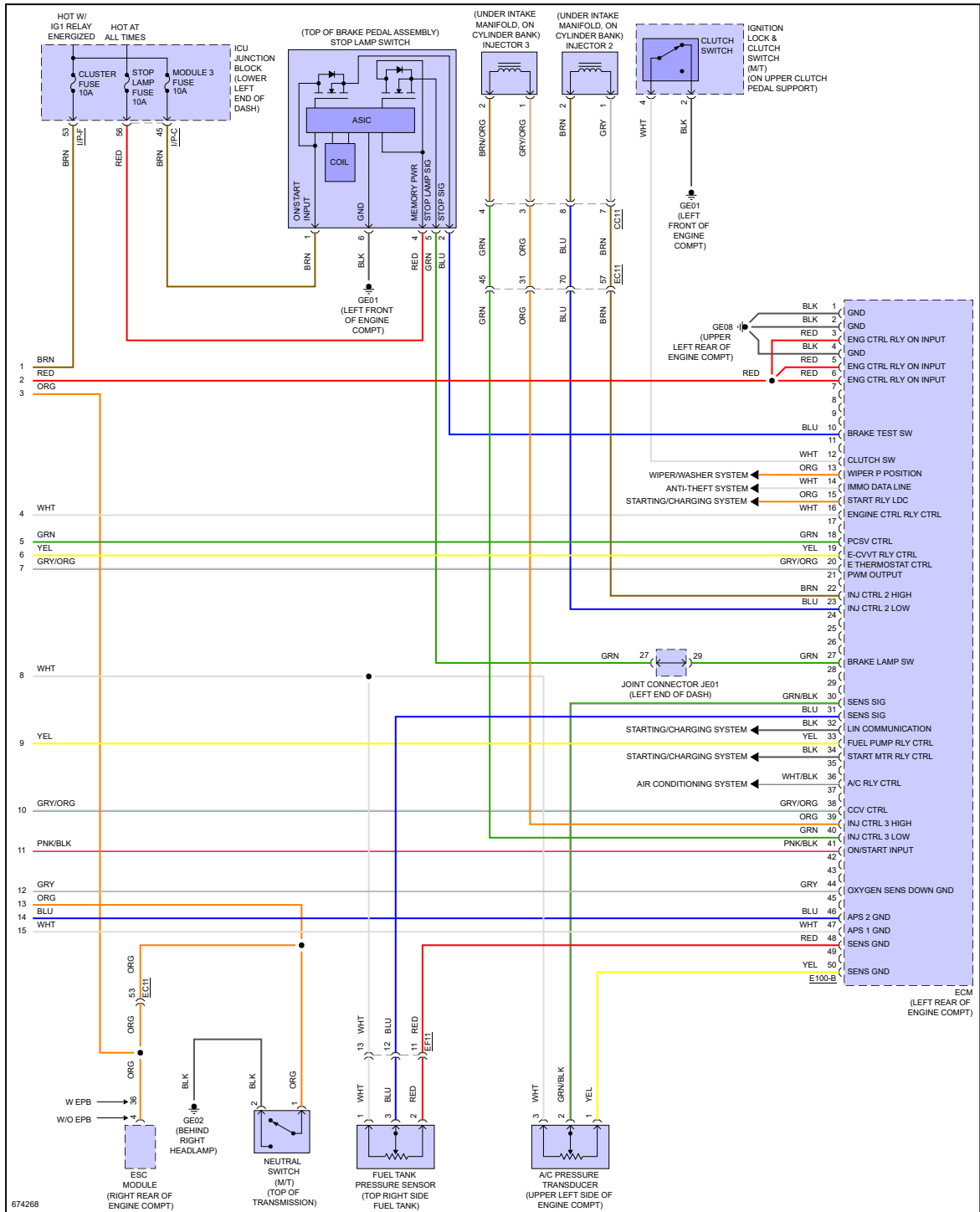
Fig 8: 2.0L Turbo, Engine Controls Circuit (7 of 7)
