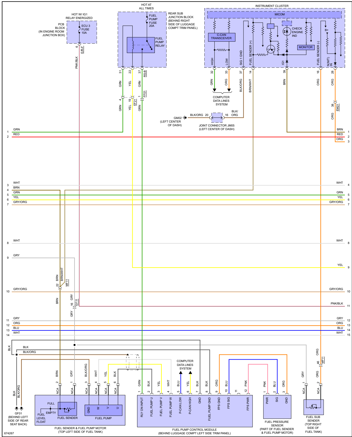
Fig 7: 2.0L Turbo, Engine Controls Circuit (6 of 7)
