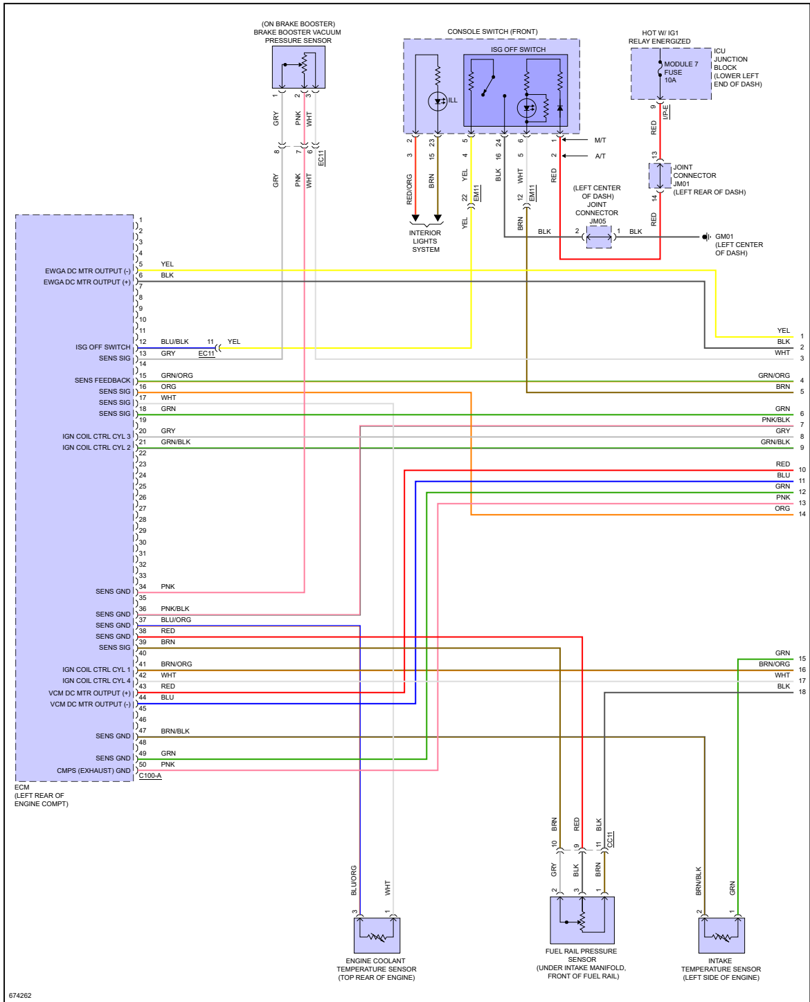
Fig 2: 2.0L Turbo, Engine Controls Circuit (1 of 7)
