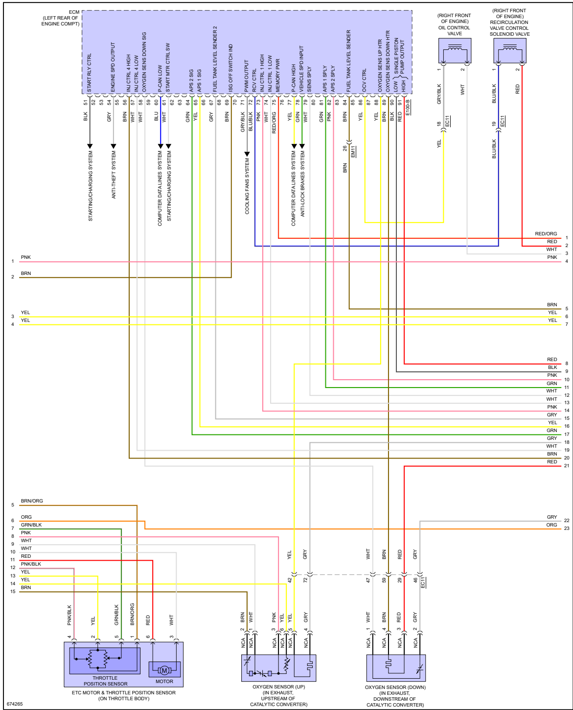
Fig 5: 2.0L Turbo, Engine Controls Circuit (4 of 7)
