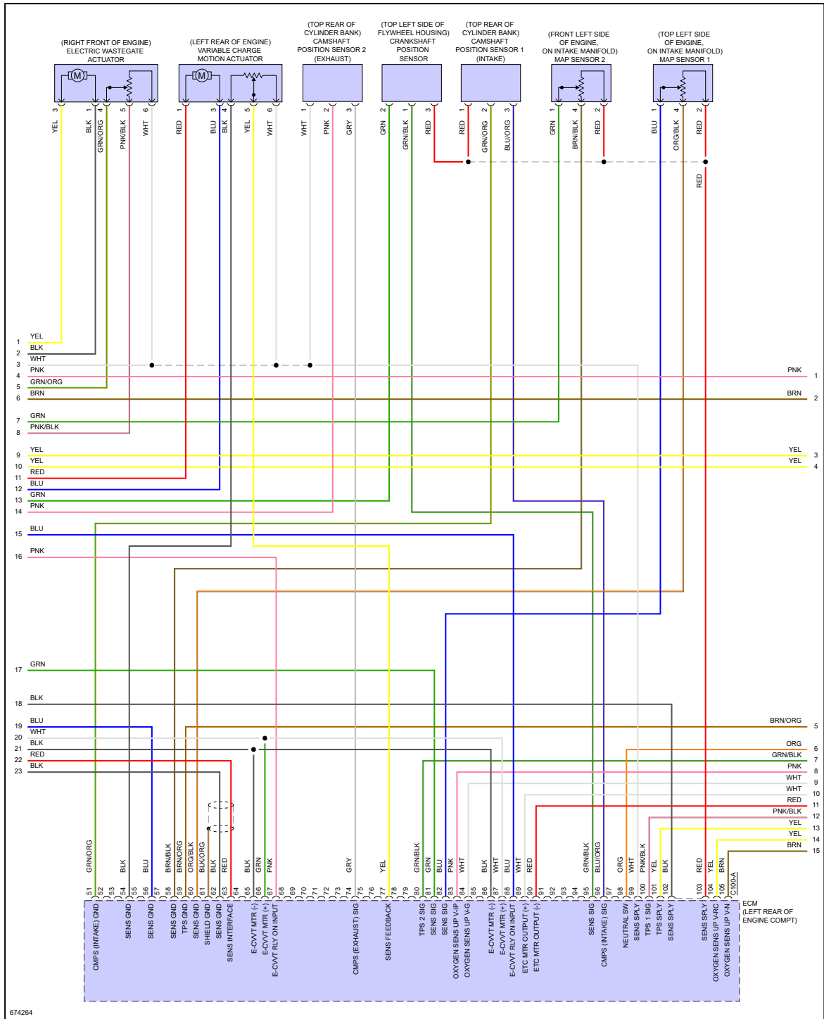
Fig 4: 2.0L Turbo, Engine Controls Circuit (3 of 7)
