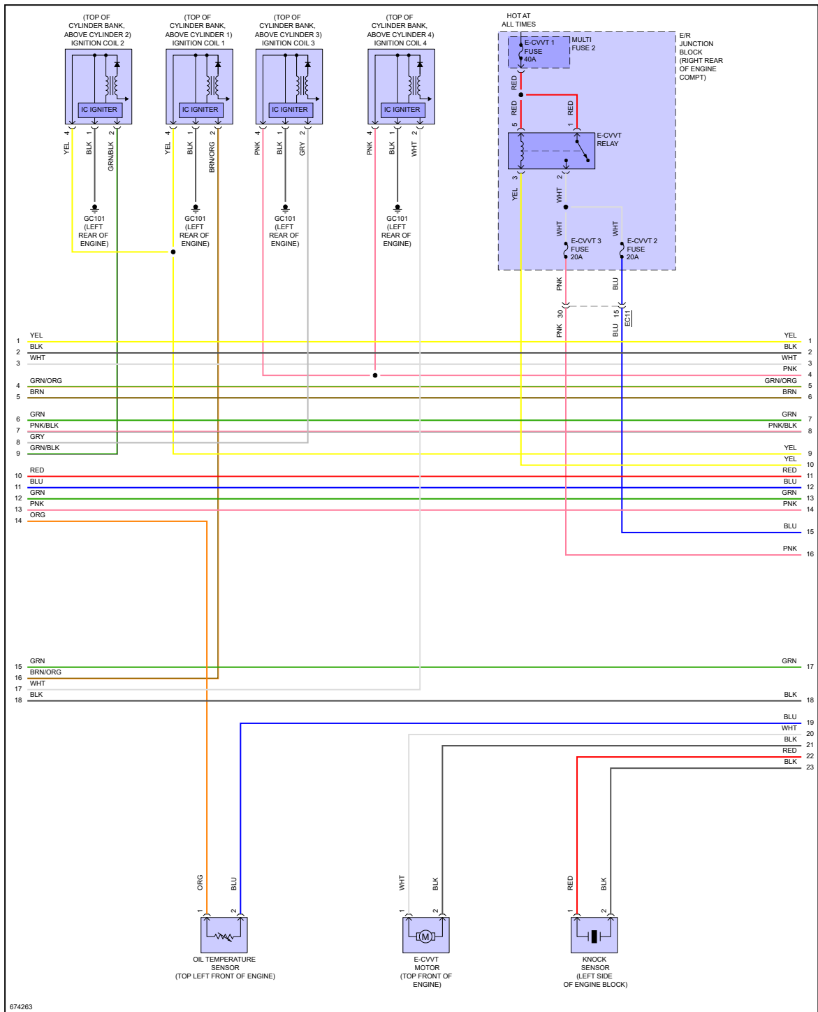
Fig 3: 2.0L Turbo, Engine Controls Circuit (2 of 7)
