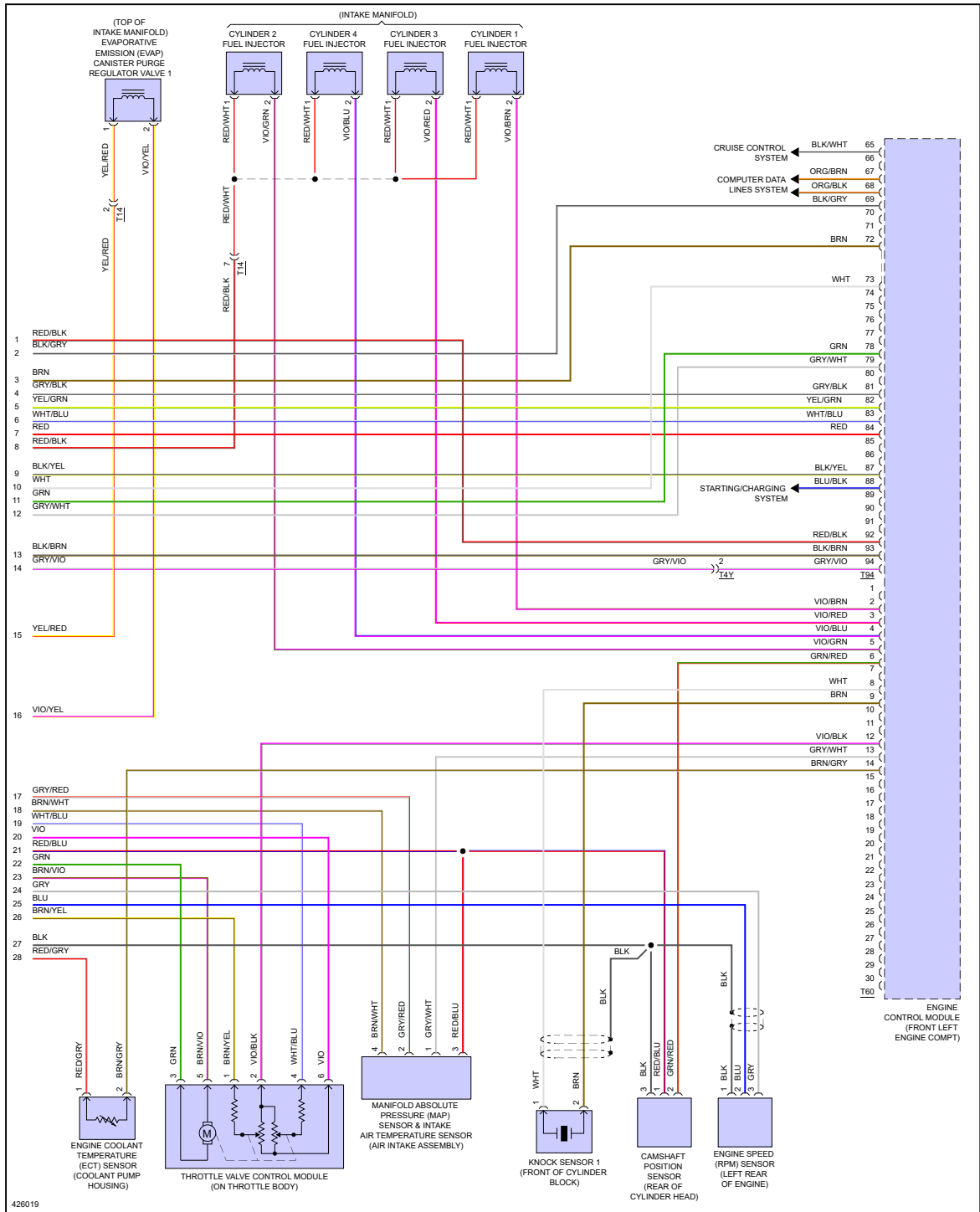
Fig 4: 2.0L, Engine Performance Circuit (4 of 4)
