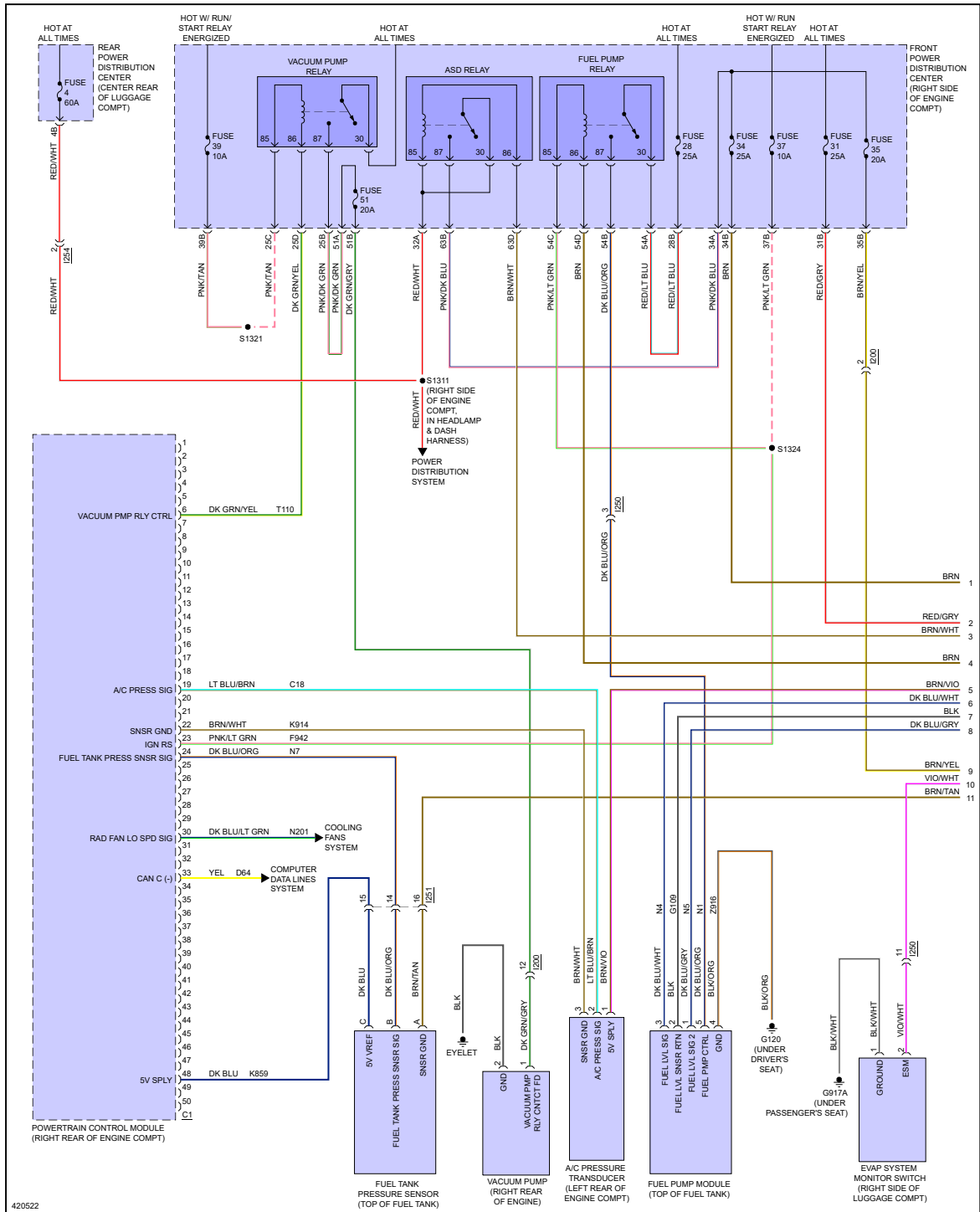
Fig 1: 3.6L, Engine Performance Circuit (1 of 5)
