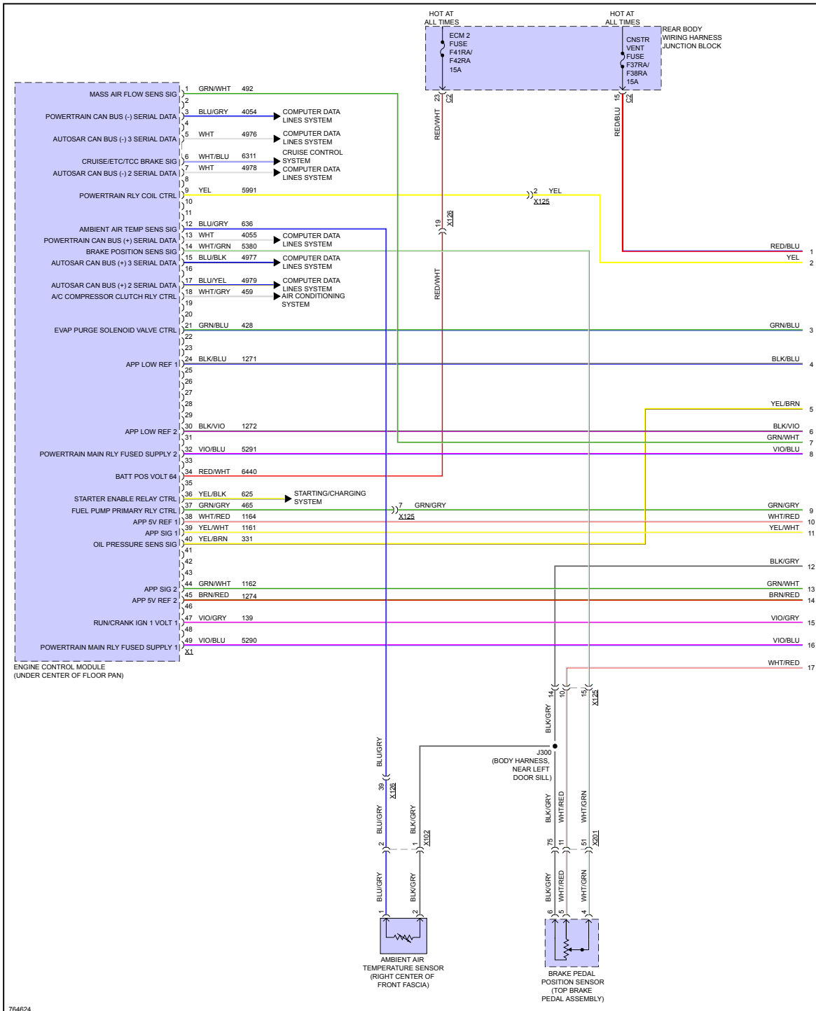
Fig 1: 6.2L VIN 4, Engine Performance Circuit (1 of 10)
