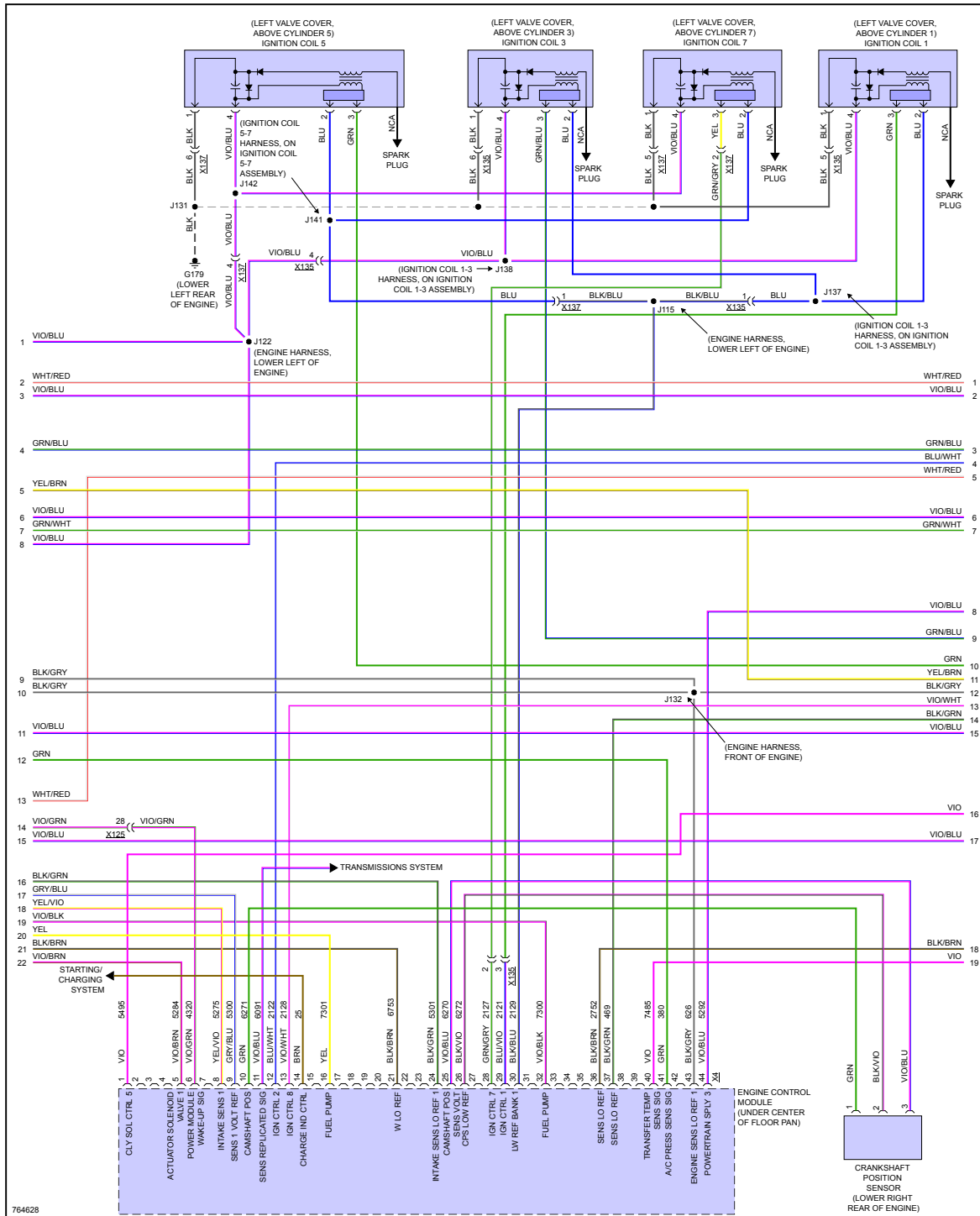
Fig 5: 6.2L VIN 4, Engine Performance Circuit (5 of 10)
