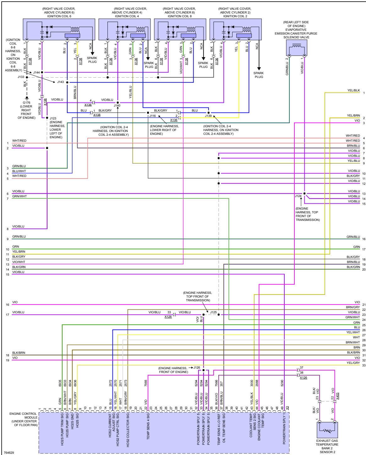
Fig 6: 6.2L VIN 4, Engine Performance Circuit (6 of 10)
