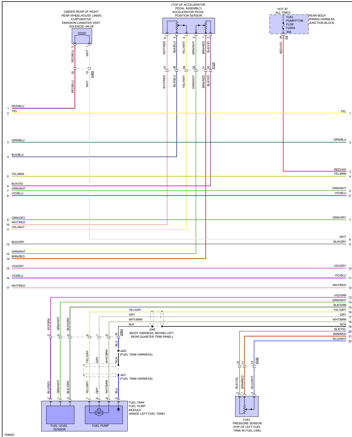
Fig 2: 6.2L VIN 4, Engine Performance Circuit (2 of 10)
