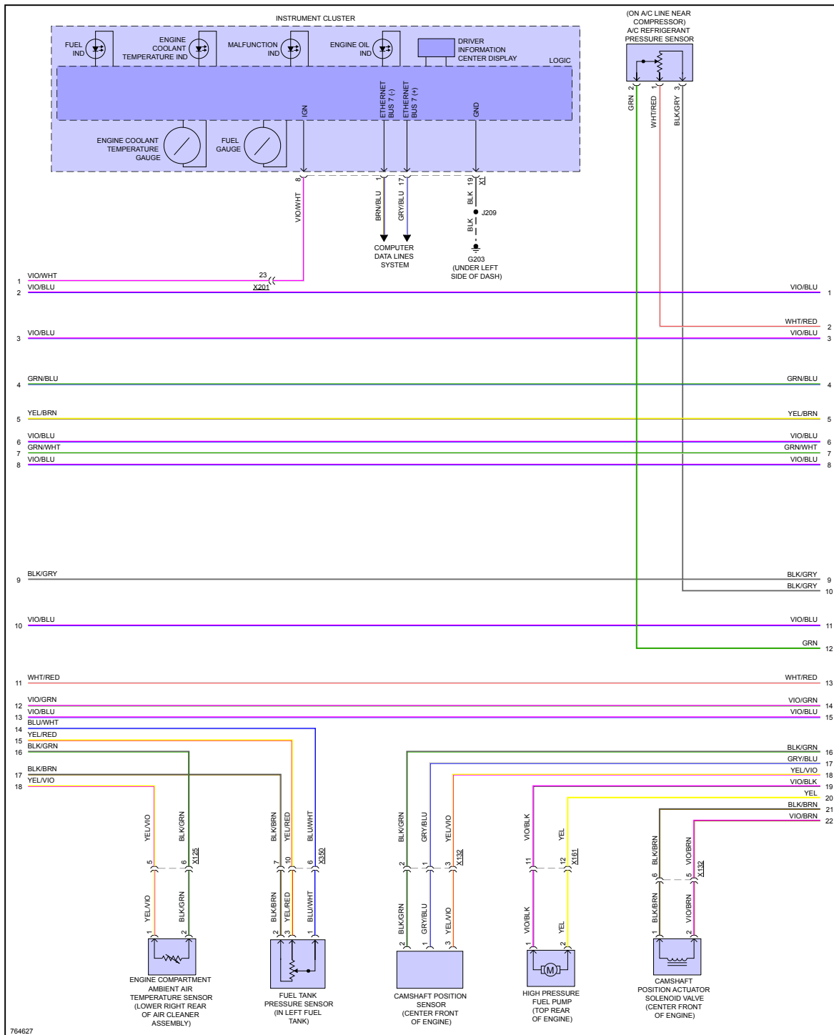
Fig 4: 6.2L VIN 4, Engine Performance Circuit (4 of 10)
