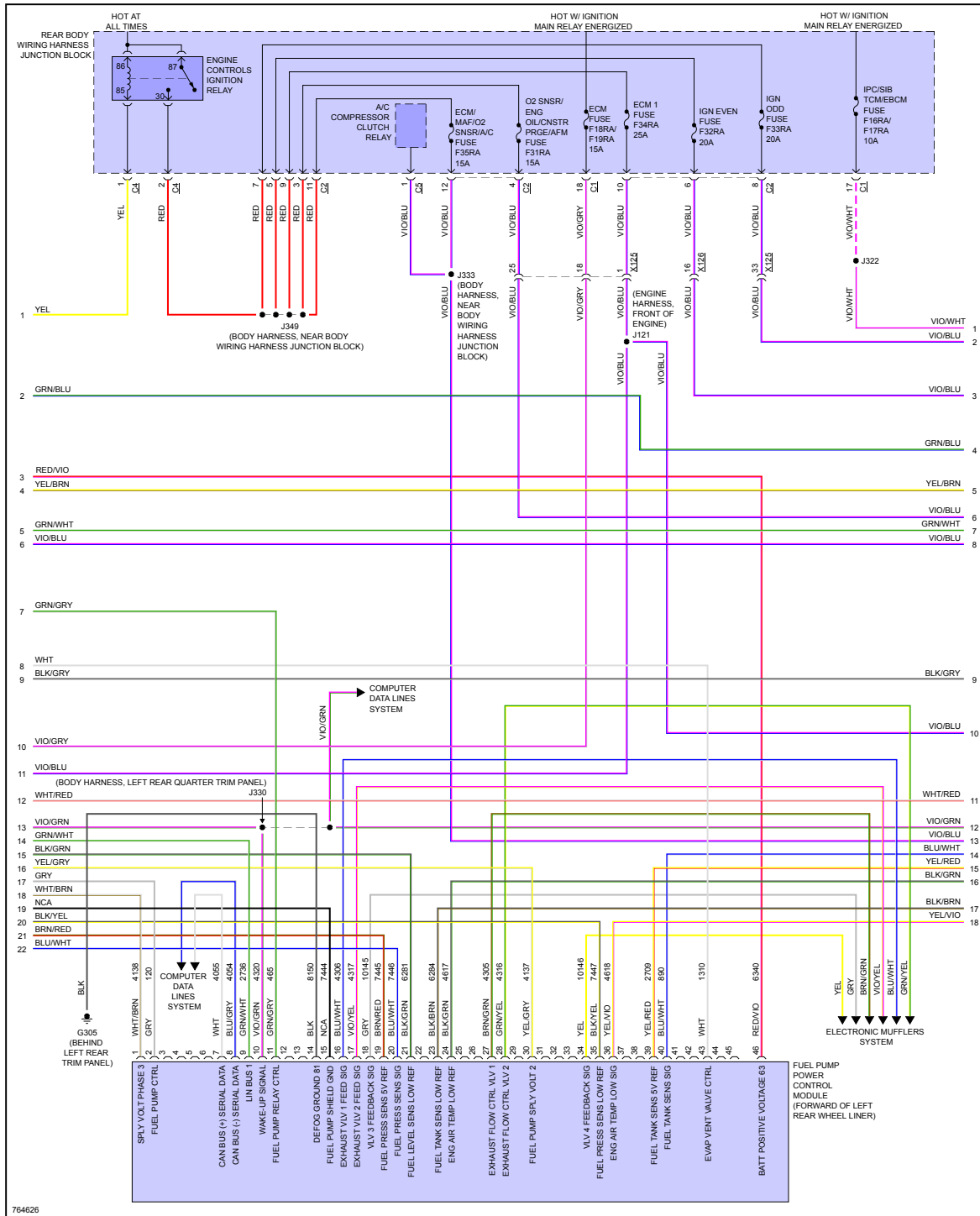
Fig 3: 6.2L VIN 4, Engine Performance Circuit (3 of 10)
