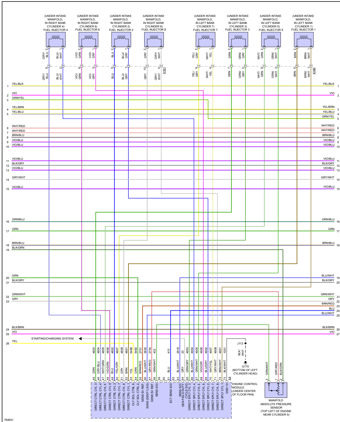
Fig 8: 6.2L VIN 4, Engine Performance Circuit (8 of 10)
