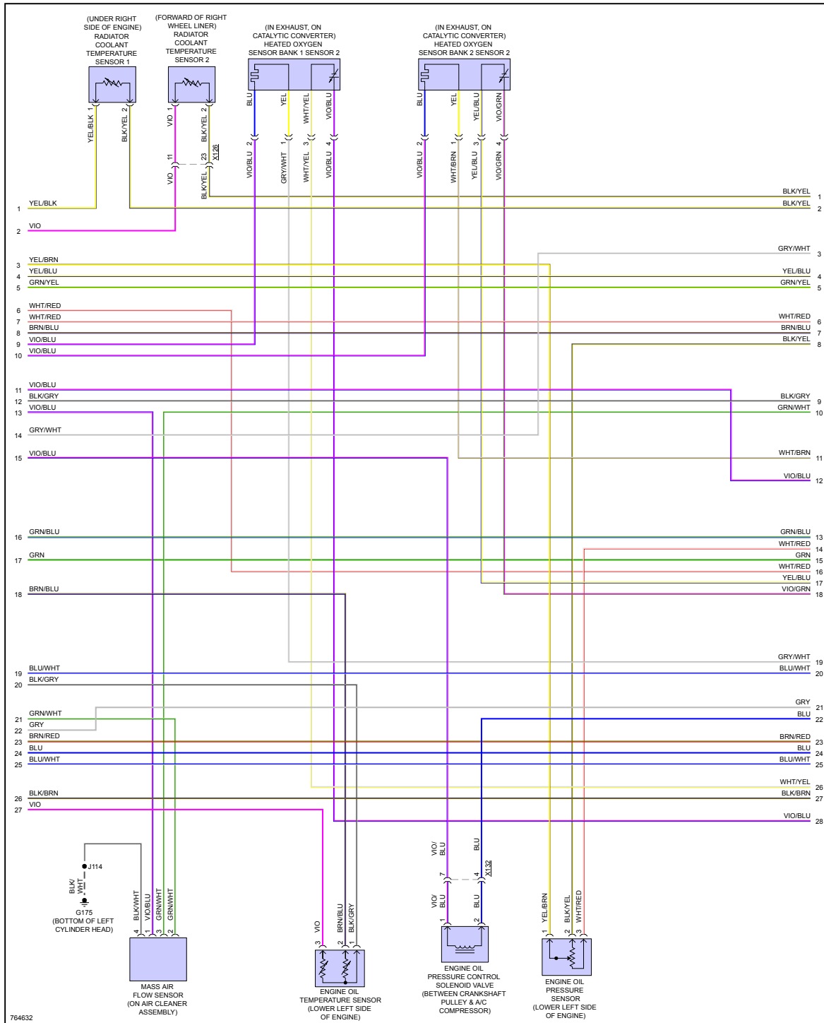
Fig 9: 6.2L VIN 4, Engine Performance Circuit (9 of 10)
