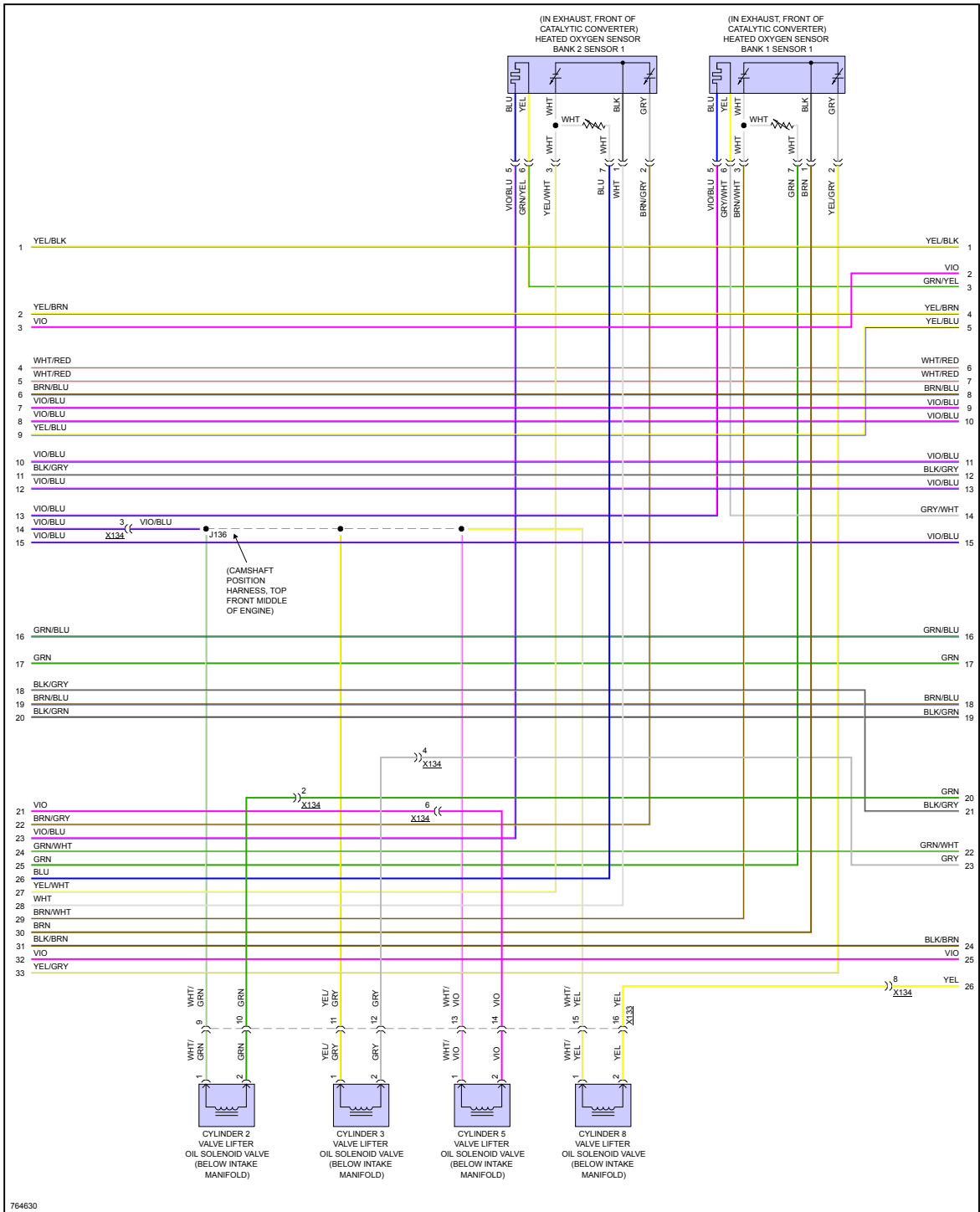
Fig 7: 6.2L VIN 4, Engine Performance Circuit (7 of 10)
