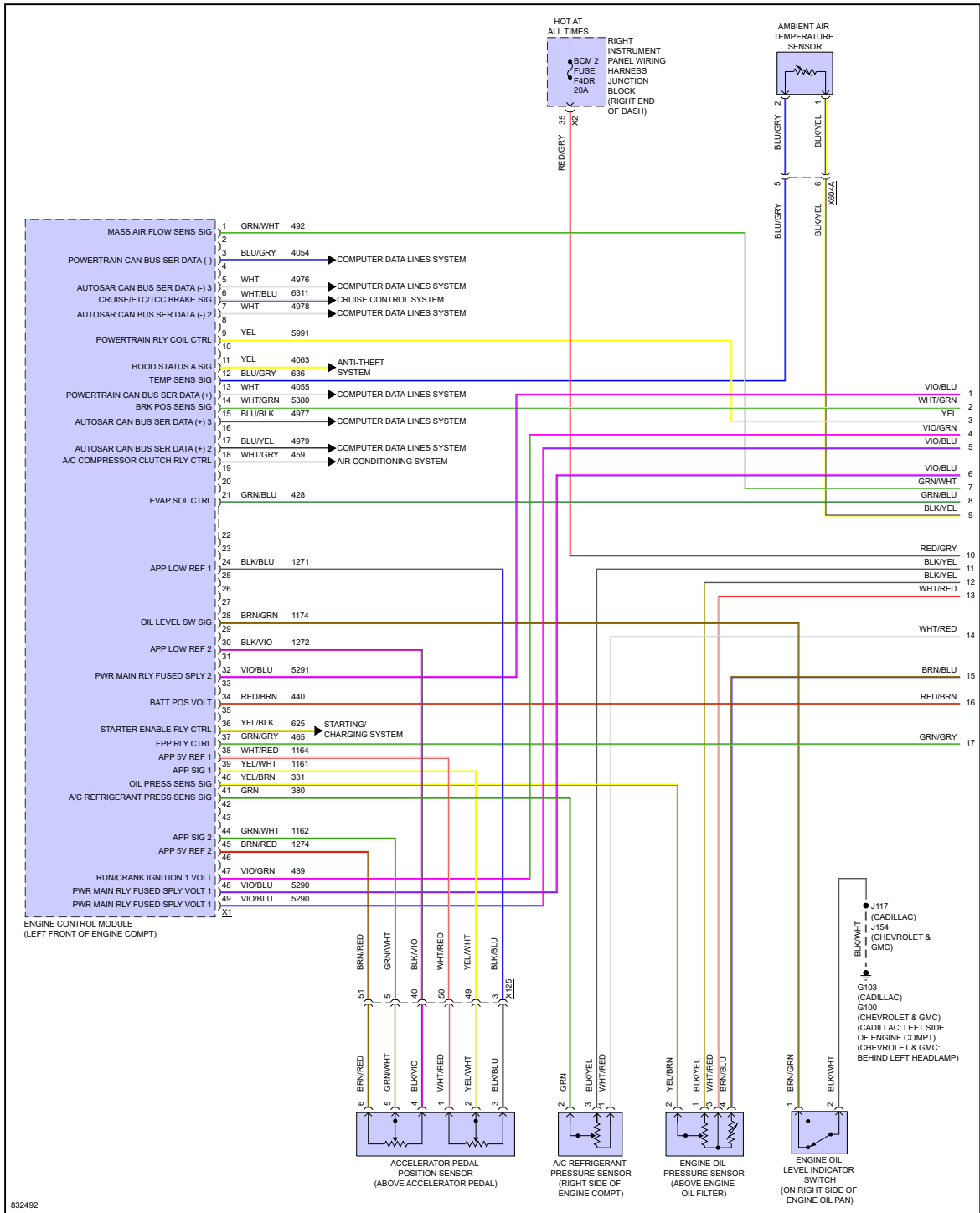
Fig 1: 5.3L VIN D, Engine Performance Circuit (1 of 7)
