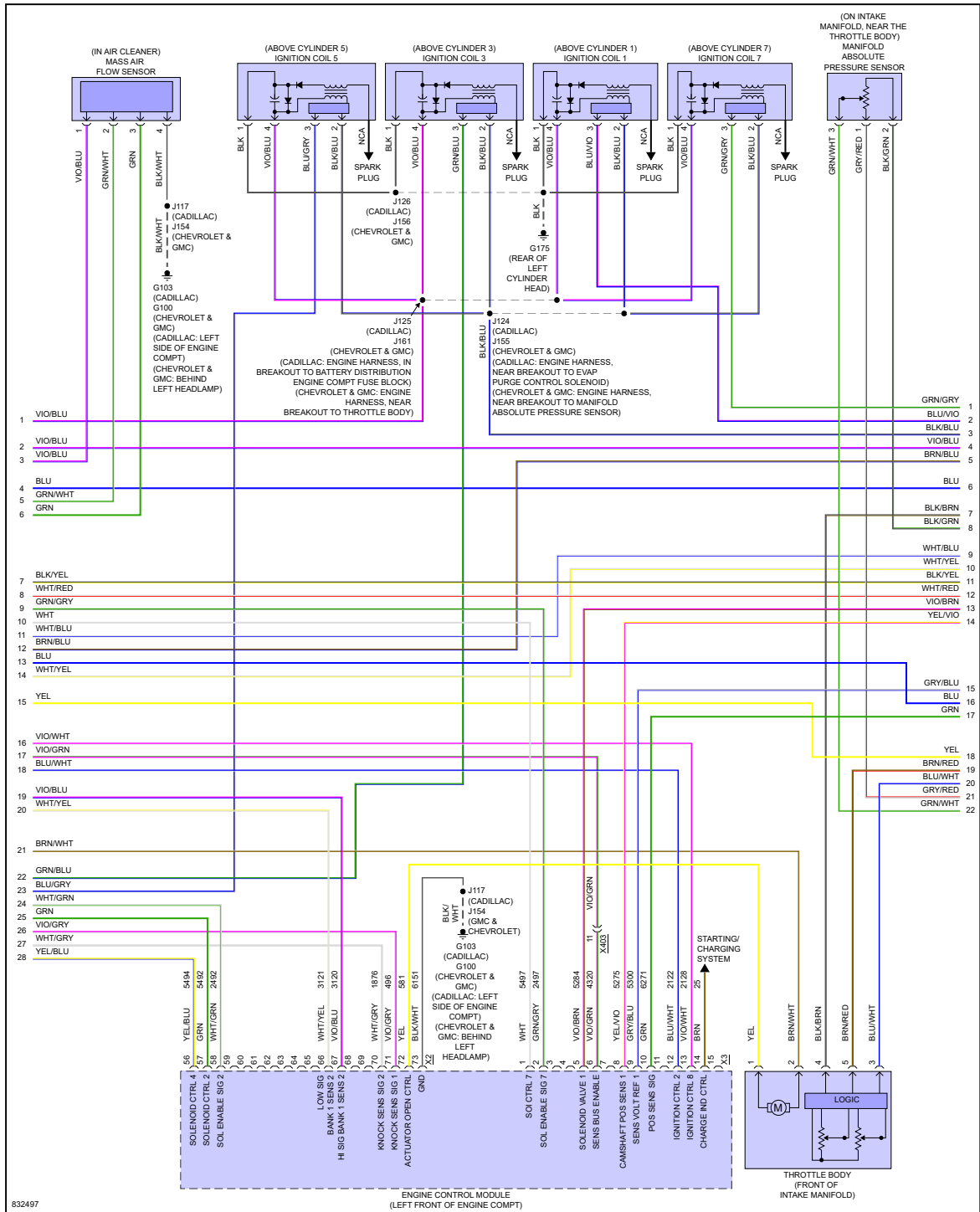
Fig 6: 5.3L VIN D, Engine Performance Circuit (6 of 7)
