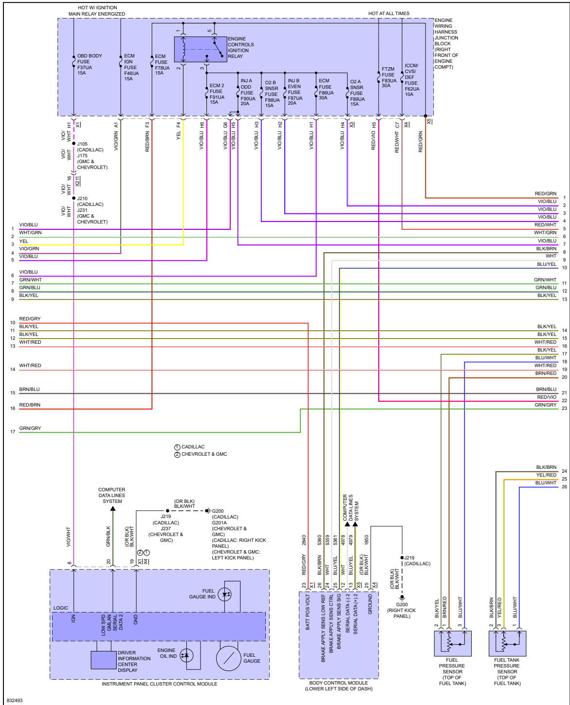
Fig 2: 5.3L VIN D, Engine Performance Circuit (2 of 7)
