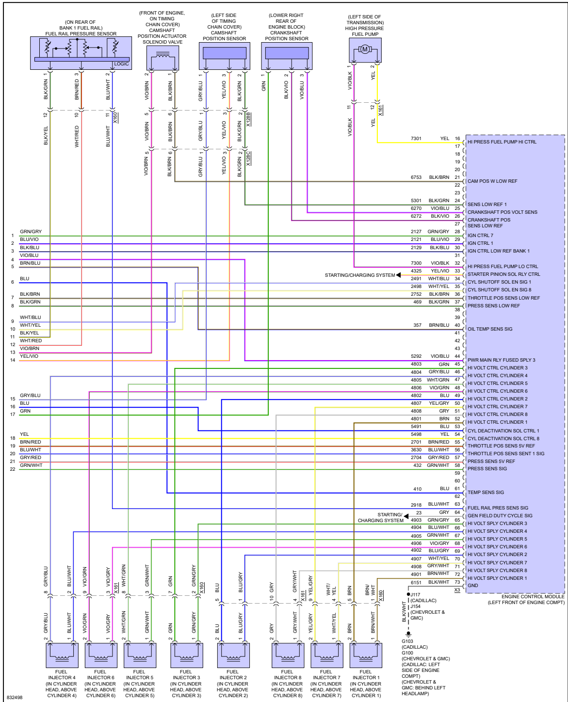
Fig 7: 5.3L VIN D, Engine Performance Circuit (7 of 7)
