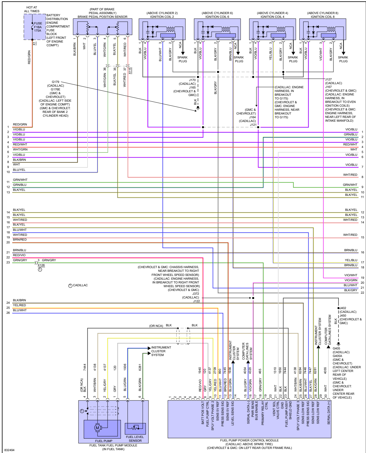
Fig 3: 5.3L VIN D, Engine Performance Circuit (3 of 7)
