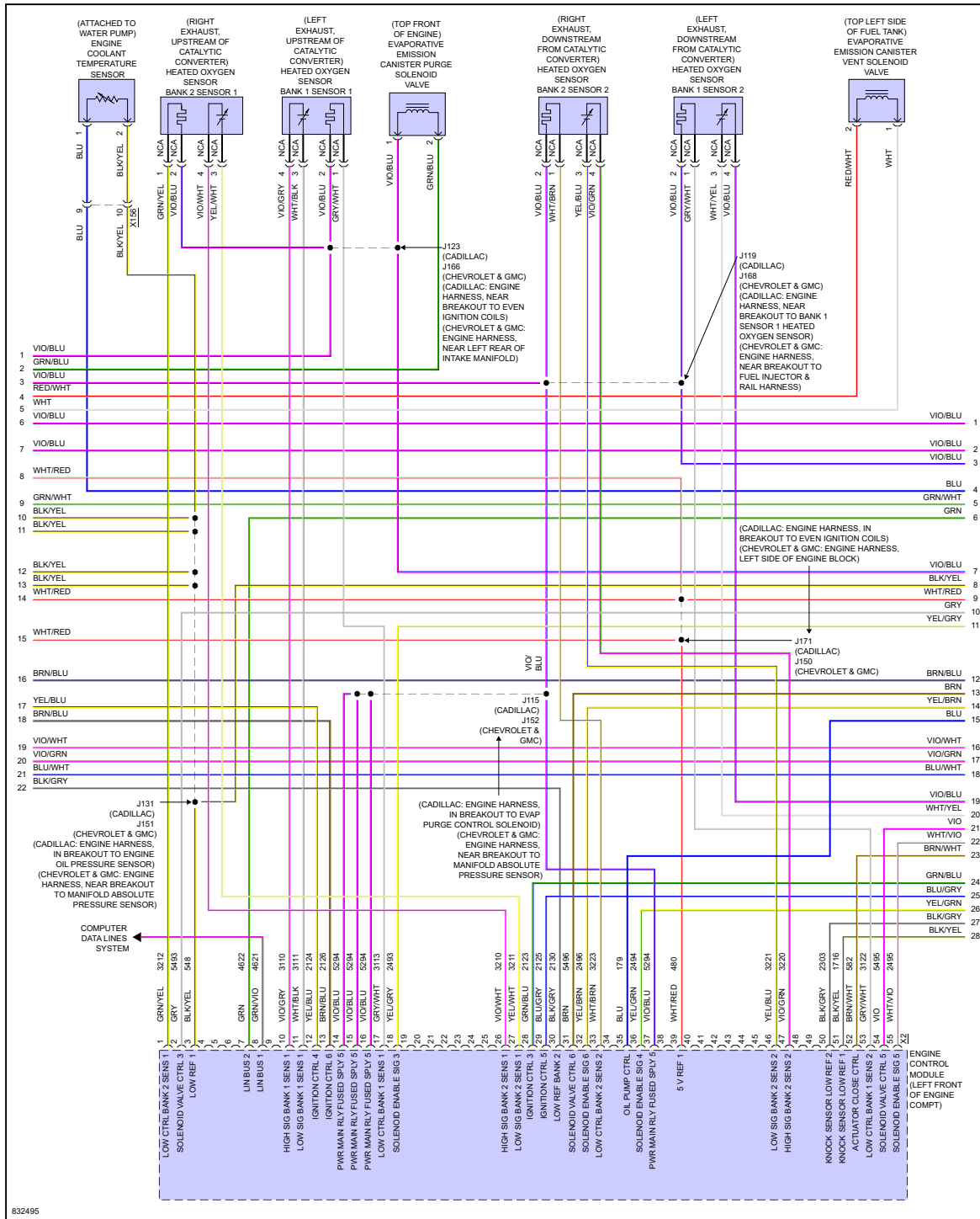
Fig 4: 5.3L VIN D, Engine Performance Circuit (4 of 7)
