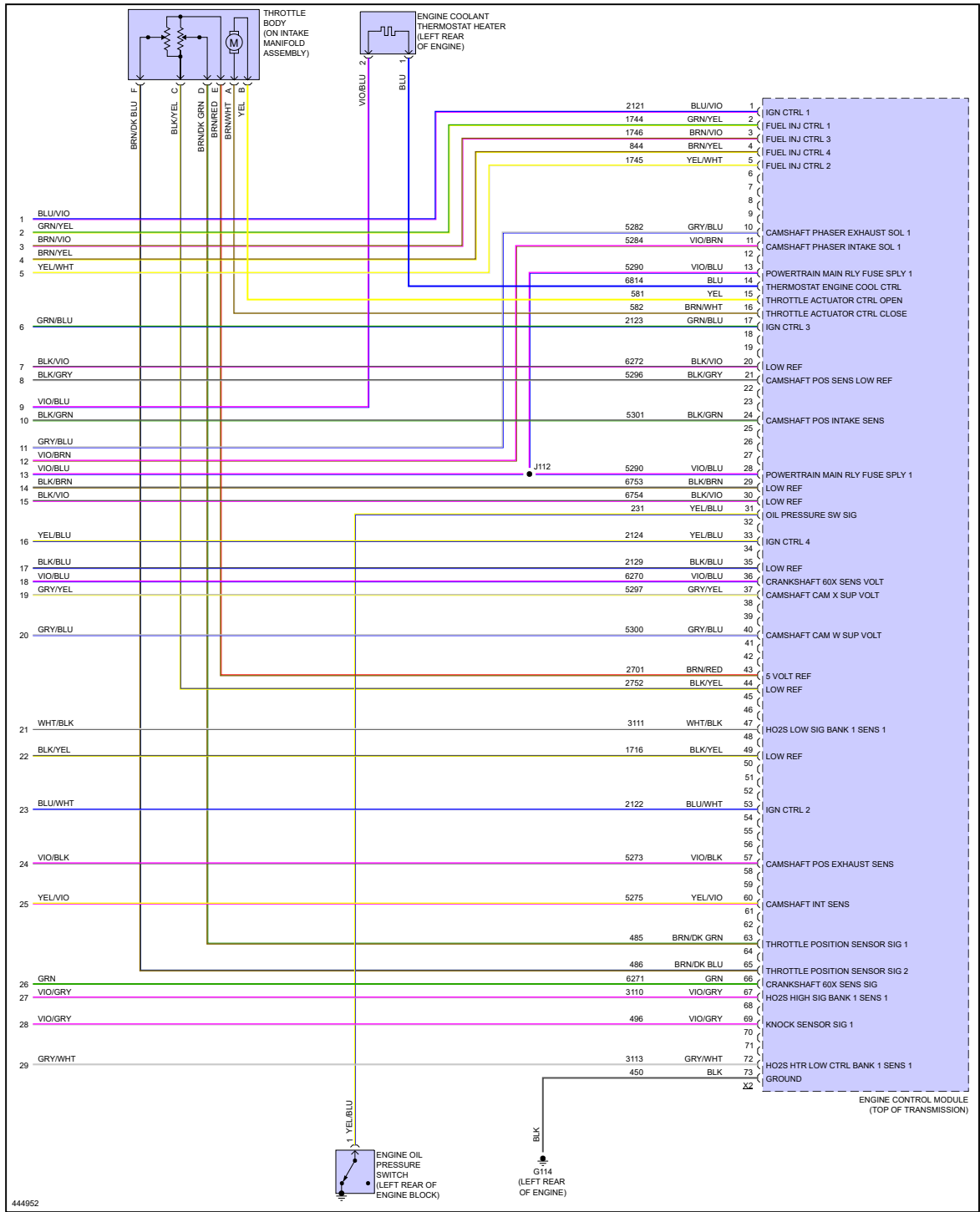
Fig 7: 1.8L VIN H, Engine Performance Circuit (7 of 7)
