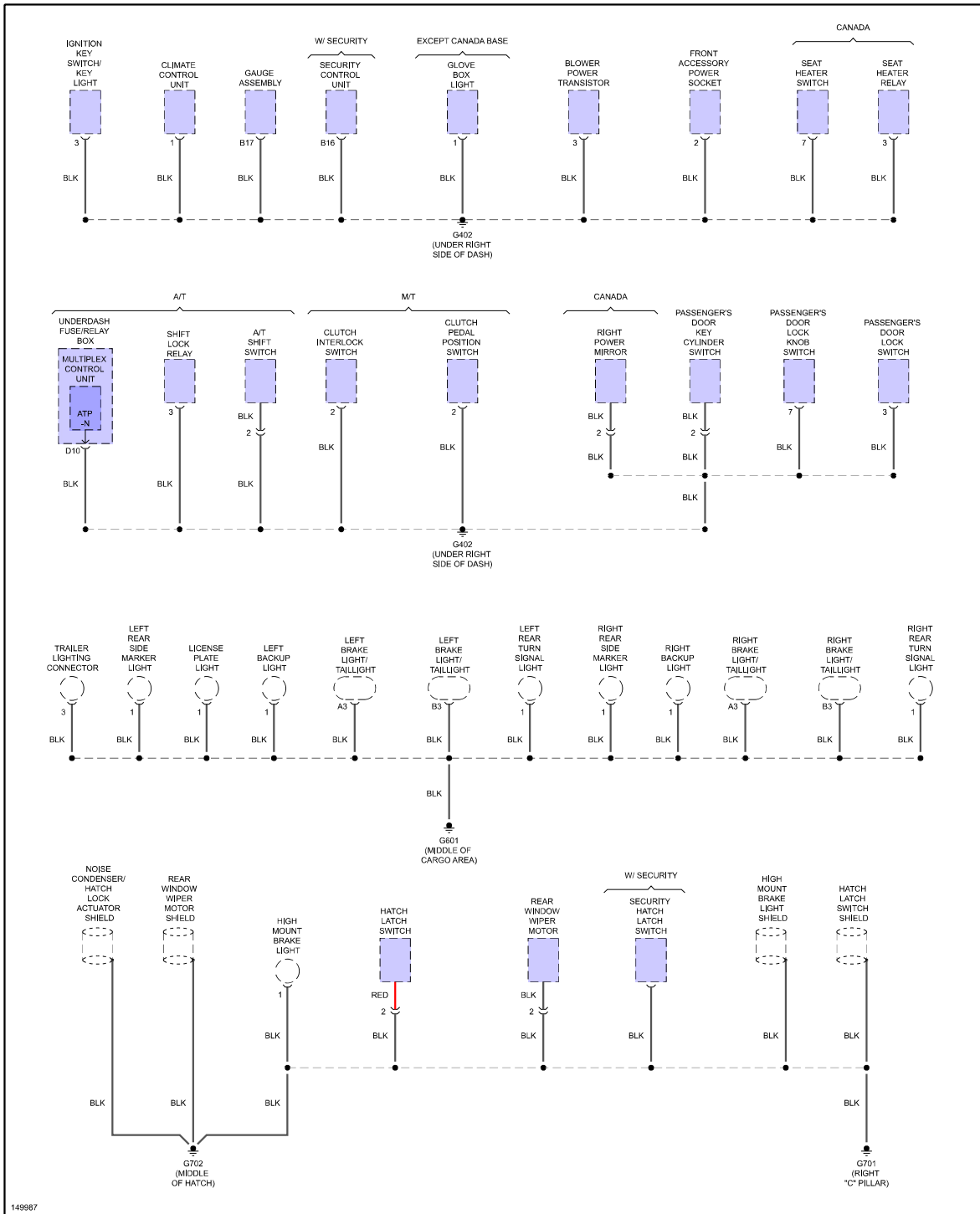
Fig 3: Ground Distribution Circuit (3 of 3)
