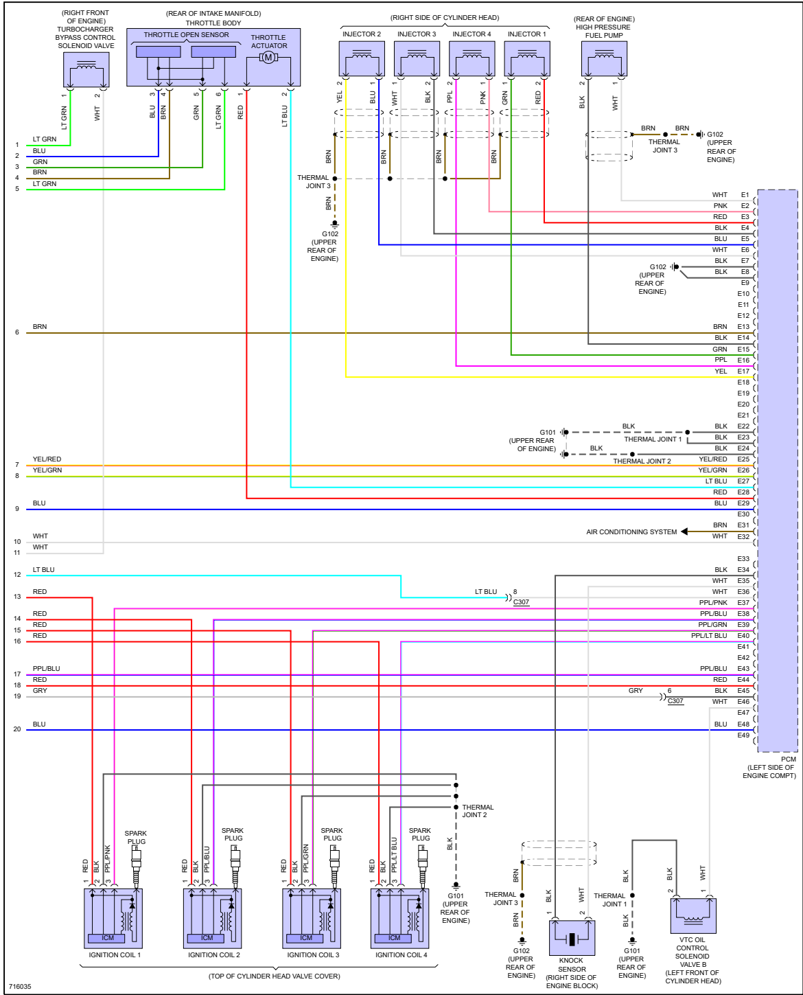
Fig 6: 1.5L Turbo, Engine Performance Circuit (6 of 6)
