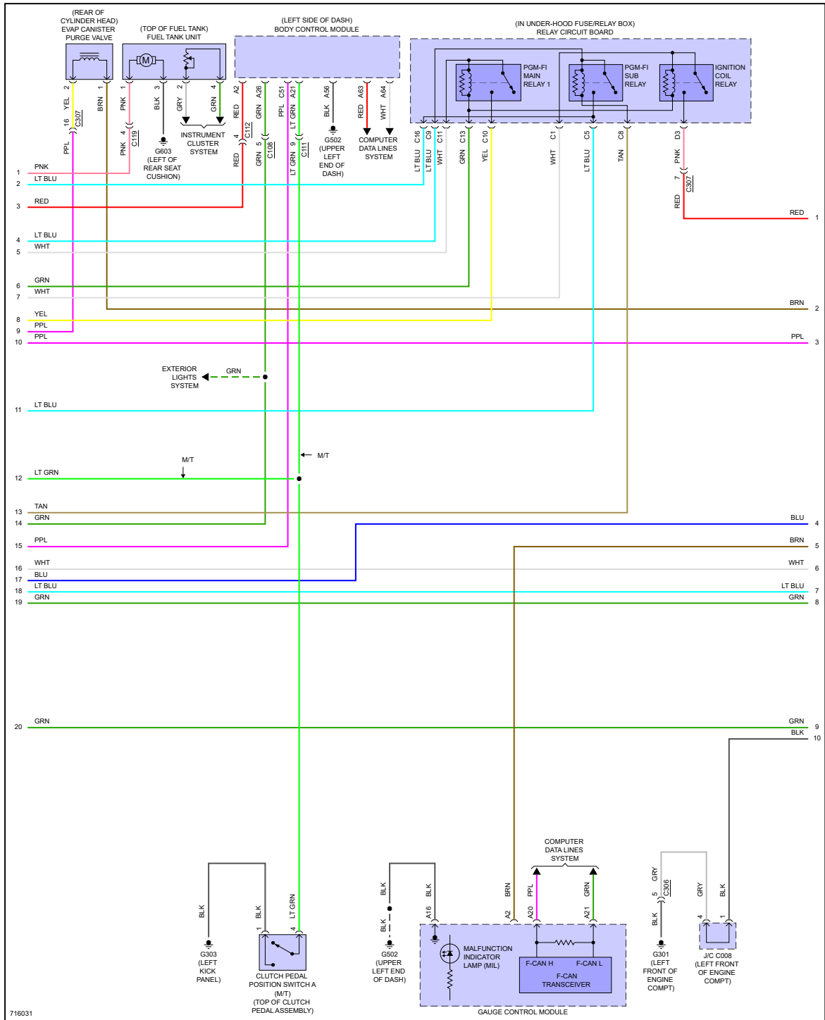
Fig 2: 1.5L Turbo, Engine Performance Circuit (2 of 6)
