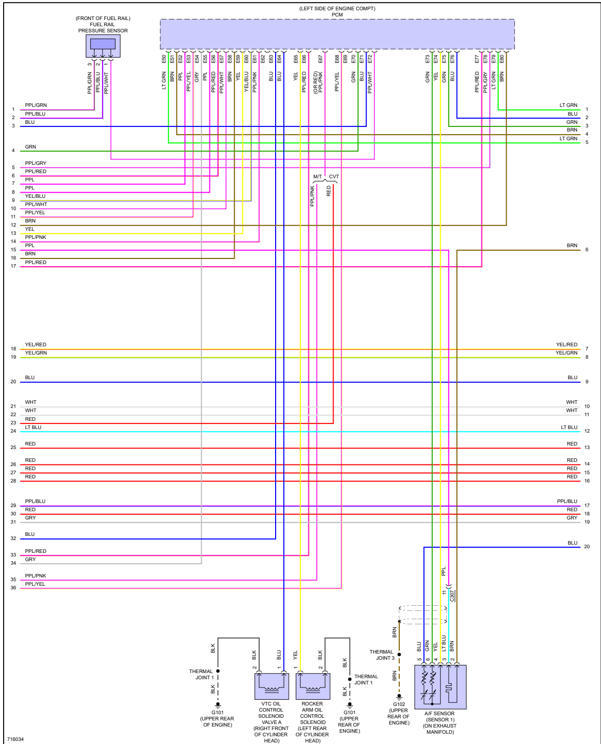
Fig 5: 1.5L Turbo, Engine Performance Circuit (5 of 6)
