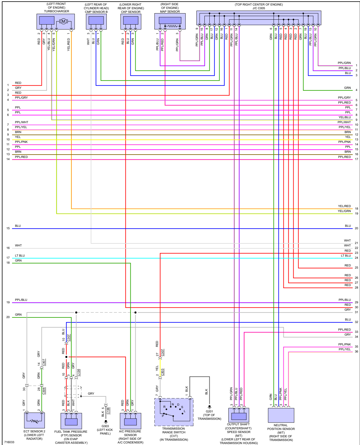
Fig 4: 1.5L Turbo, Engine Performance Circuit (4 of 6)
