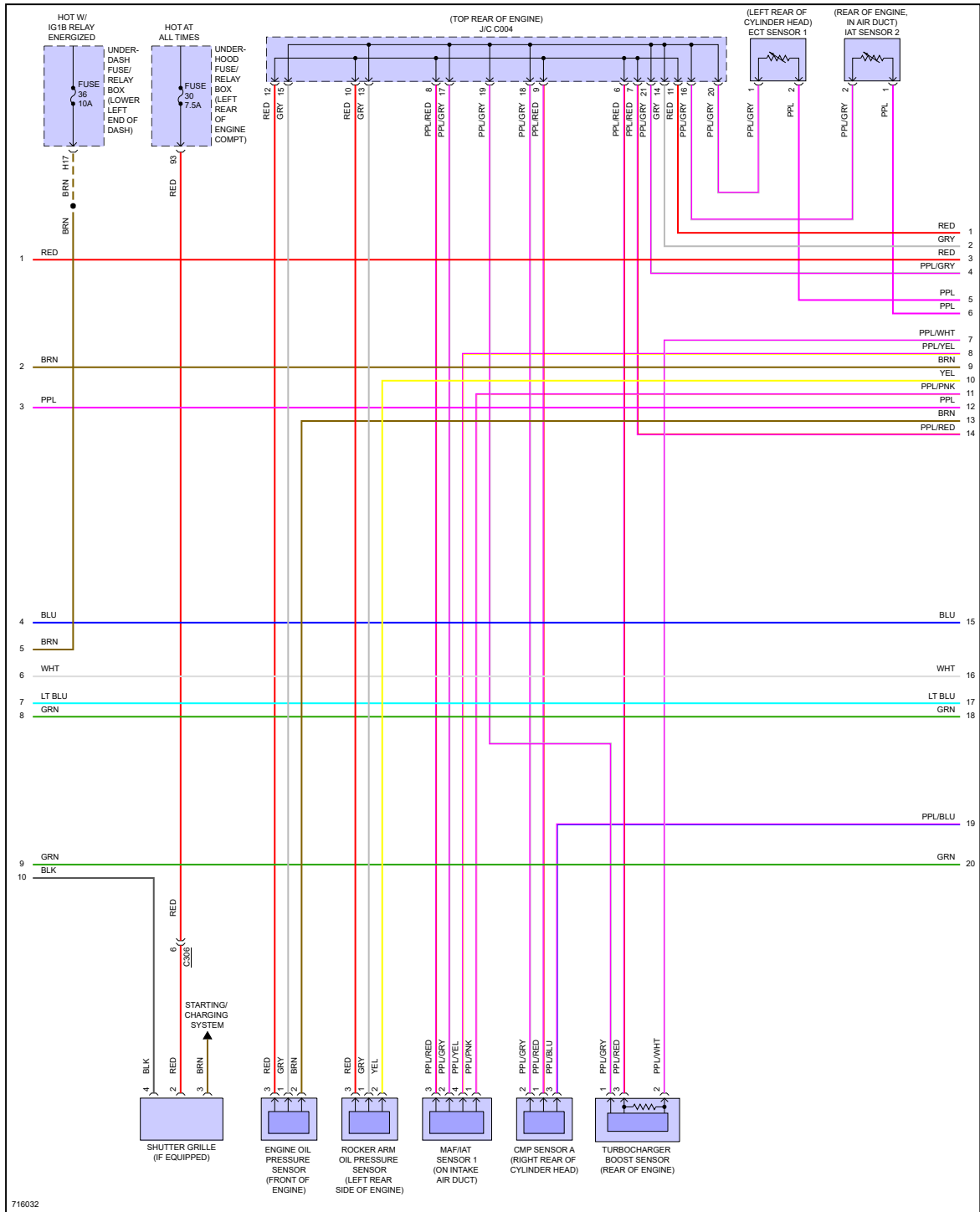
Fig 3: 1.5L Turbo, Engine Performance Circuit (3 of 6)
