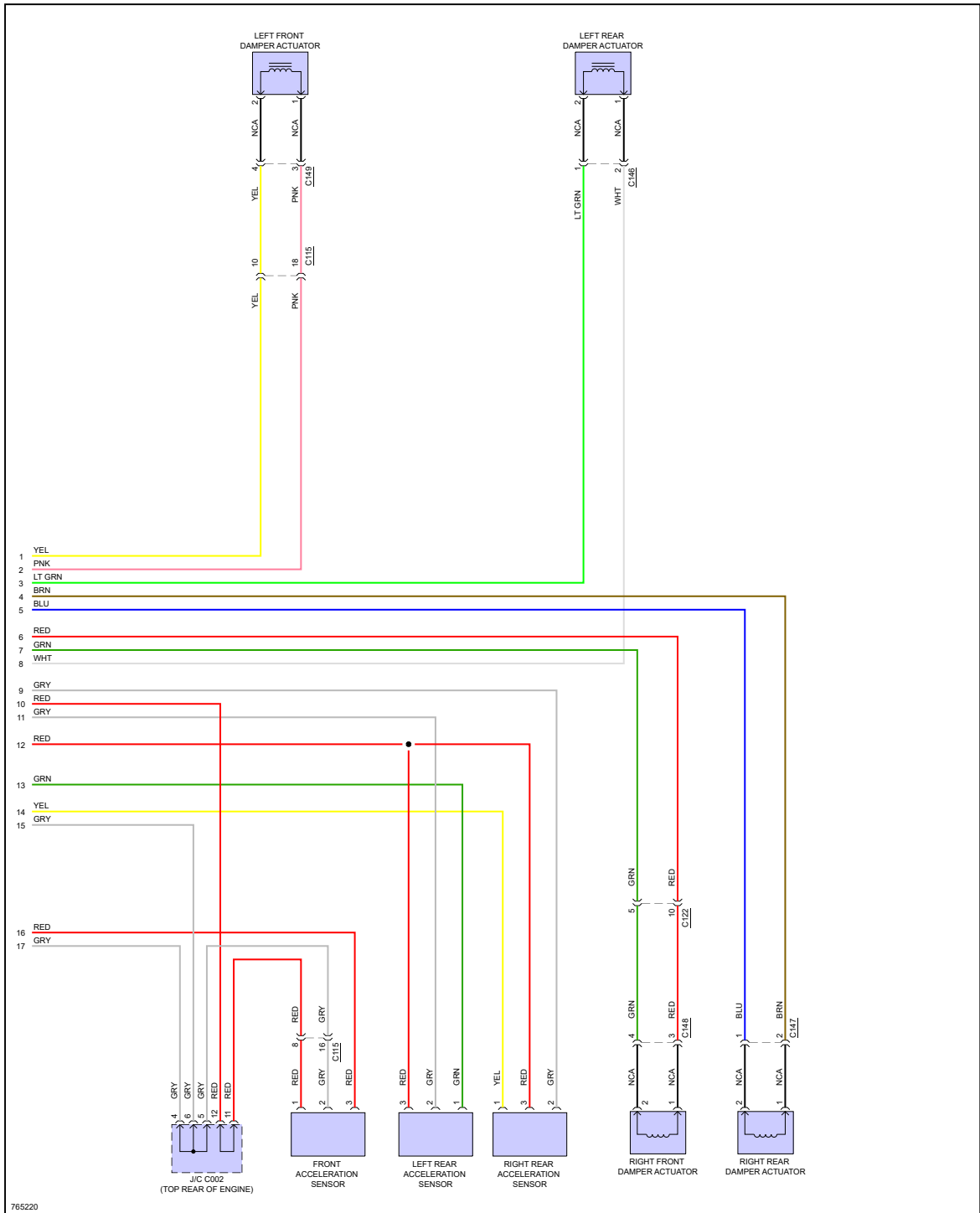
Fig 2: Electronic Suspension Circuit (2 of 2)
