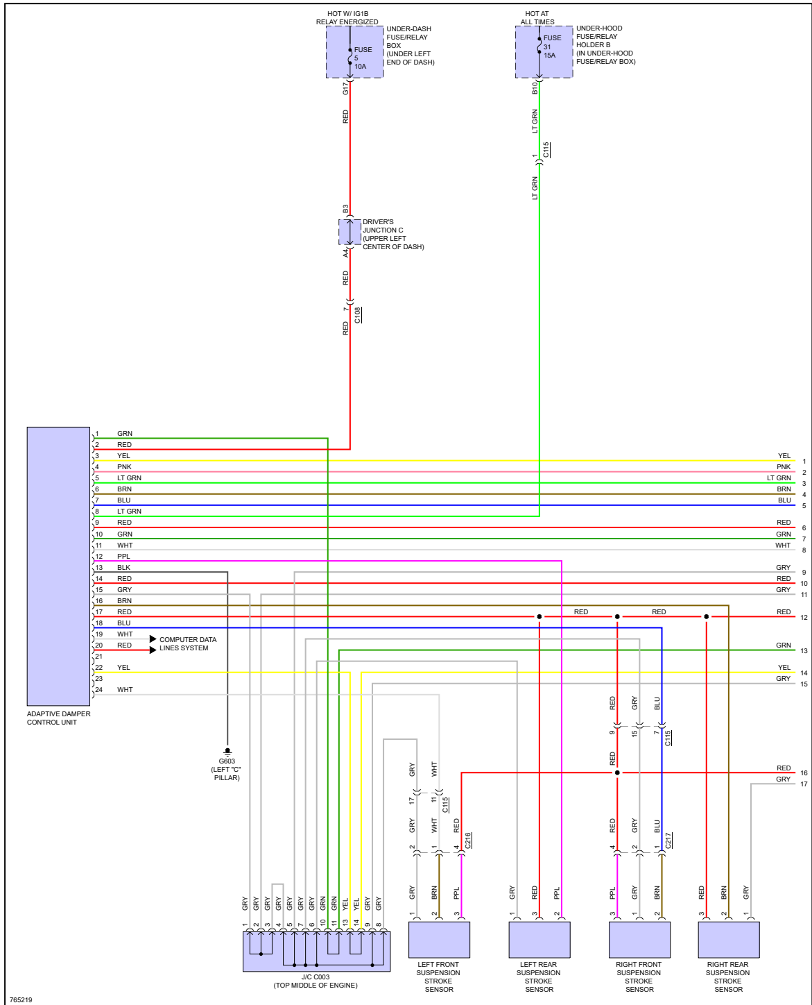
Fig 1: Electronic Suspension Circuit (1 of 2)
