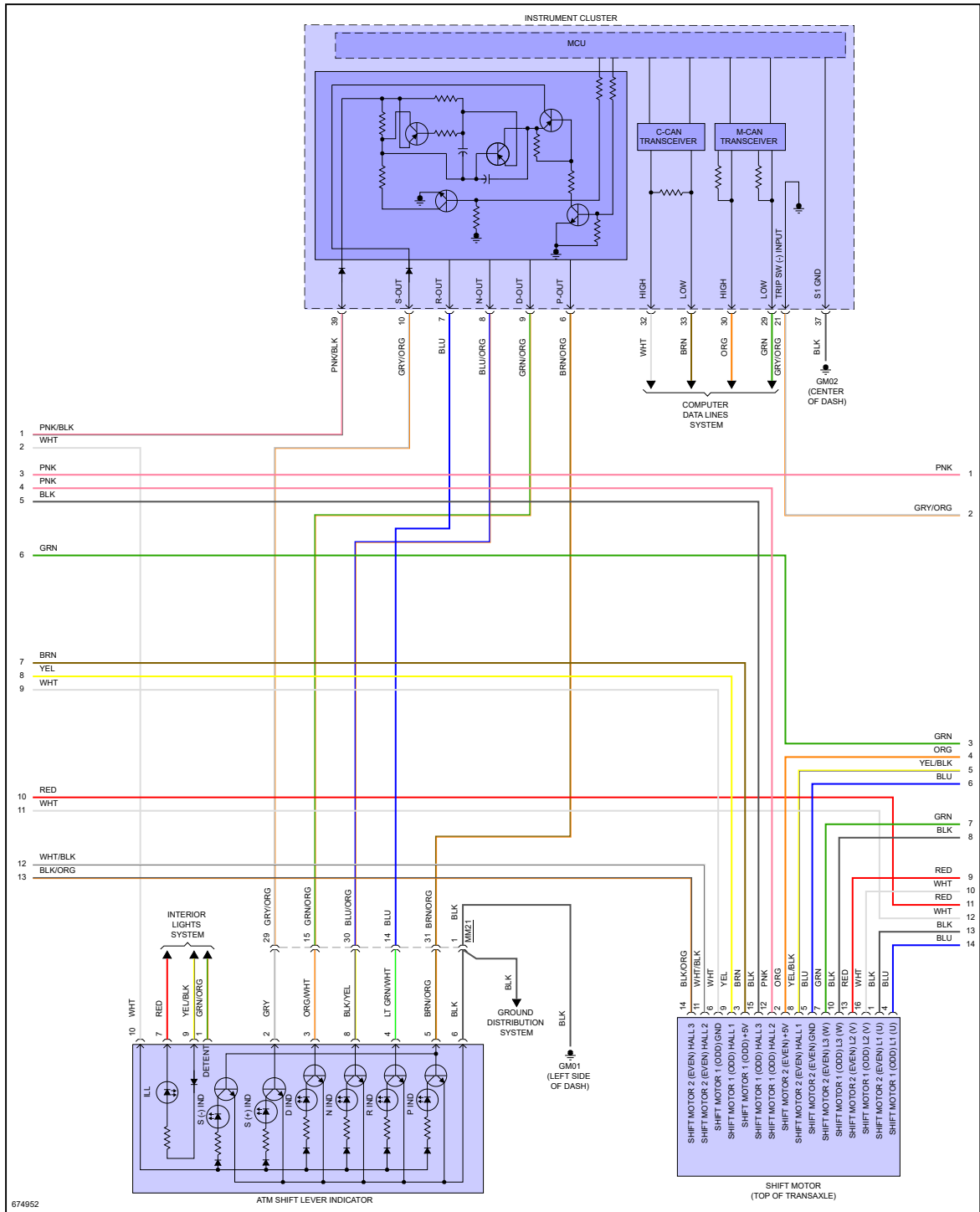
Fig 2: 1.6L Turbo, A/T Circuit (2 of 3)
