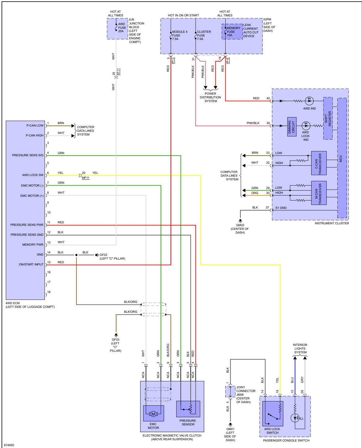
Fig 4: 1.6L Turbo, Transfer Case Circuit
