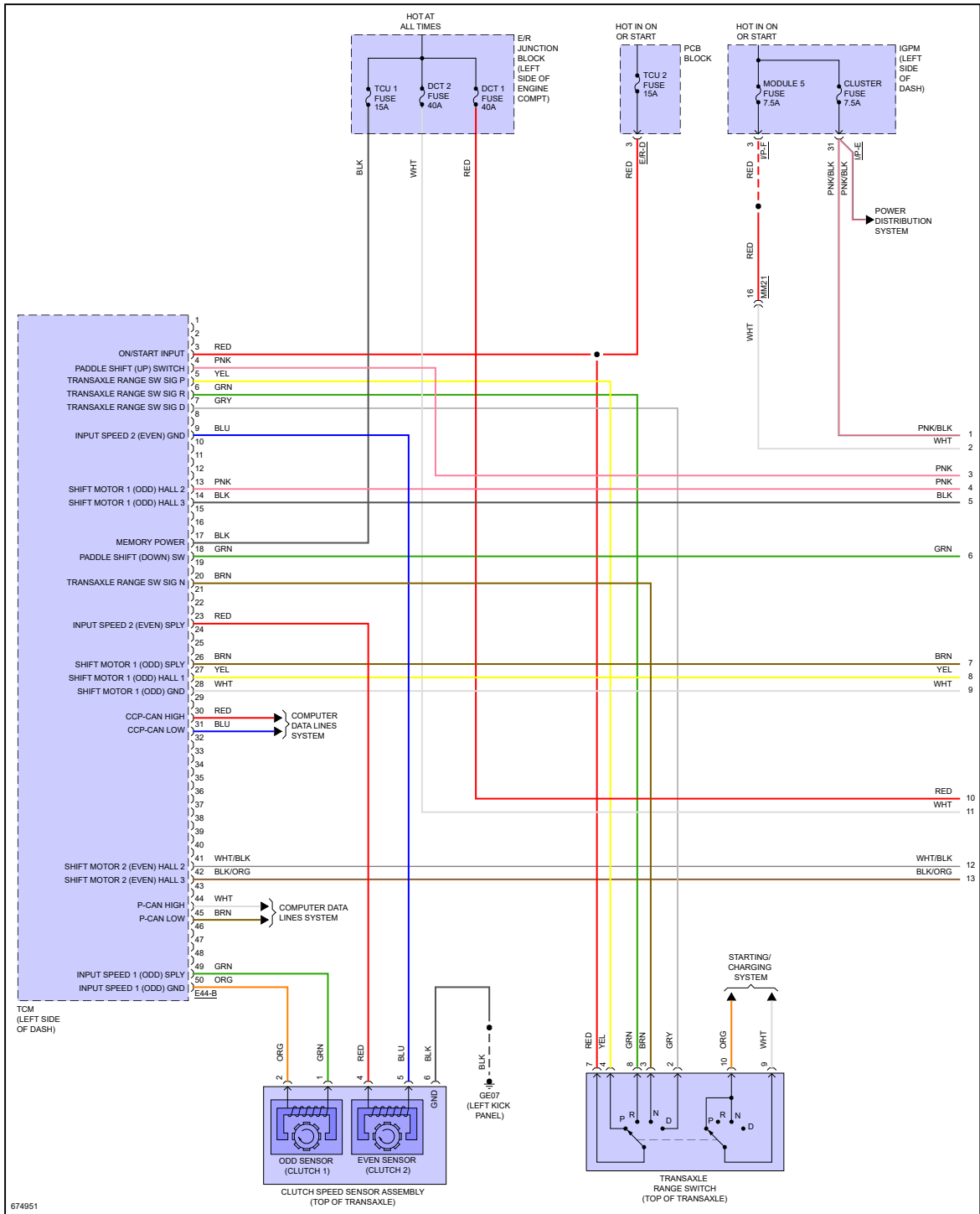
Fig 1: 1.6L Turbo, A/T Circuit (1 of 3)
