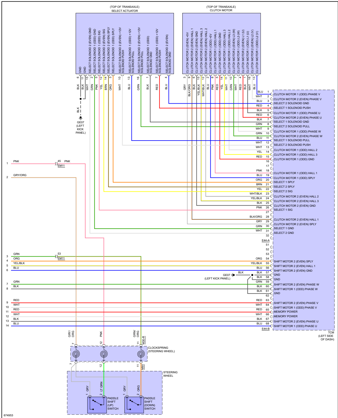
Fig 3: 1.6L Turbo, A/T Circuit (3 of 3)
