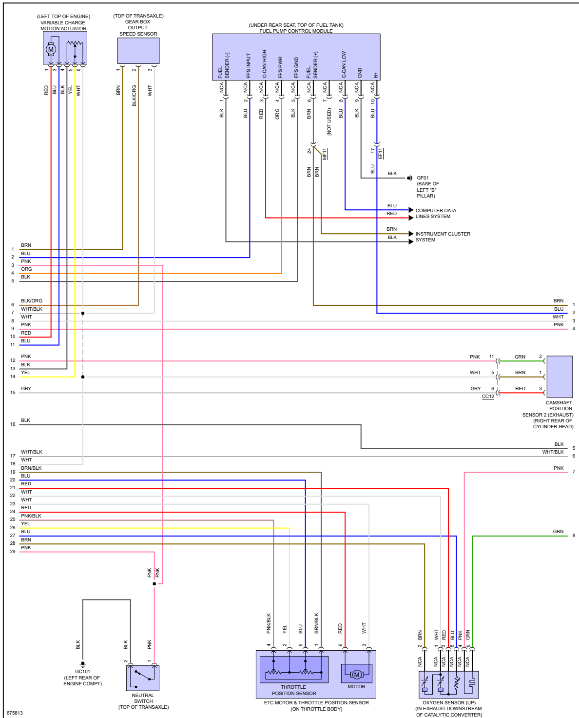
Fig 4: 2.0L Turbo, MFI Control Circuit (4 of 7)
