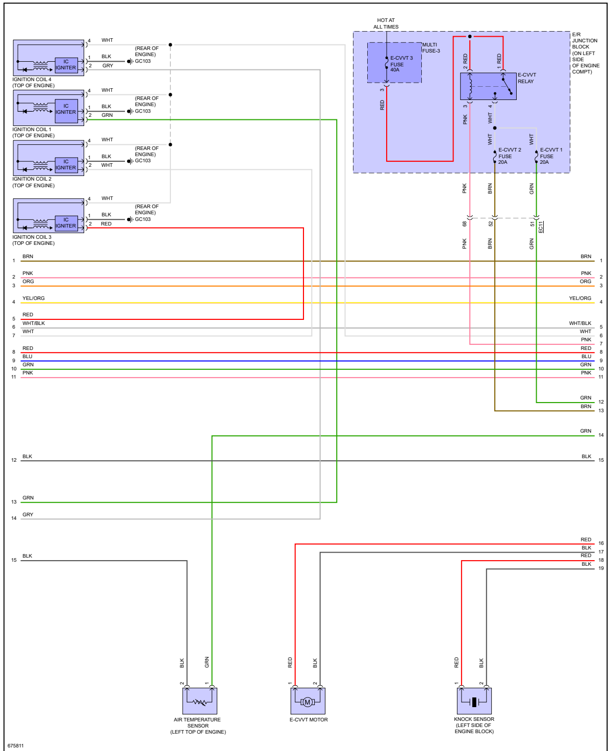
Fig 2: 2.0L Turbo, MFI Control Circuit (2 of 7)
