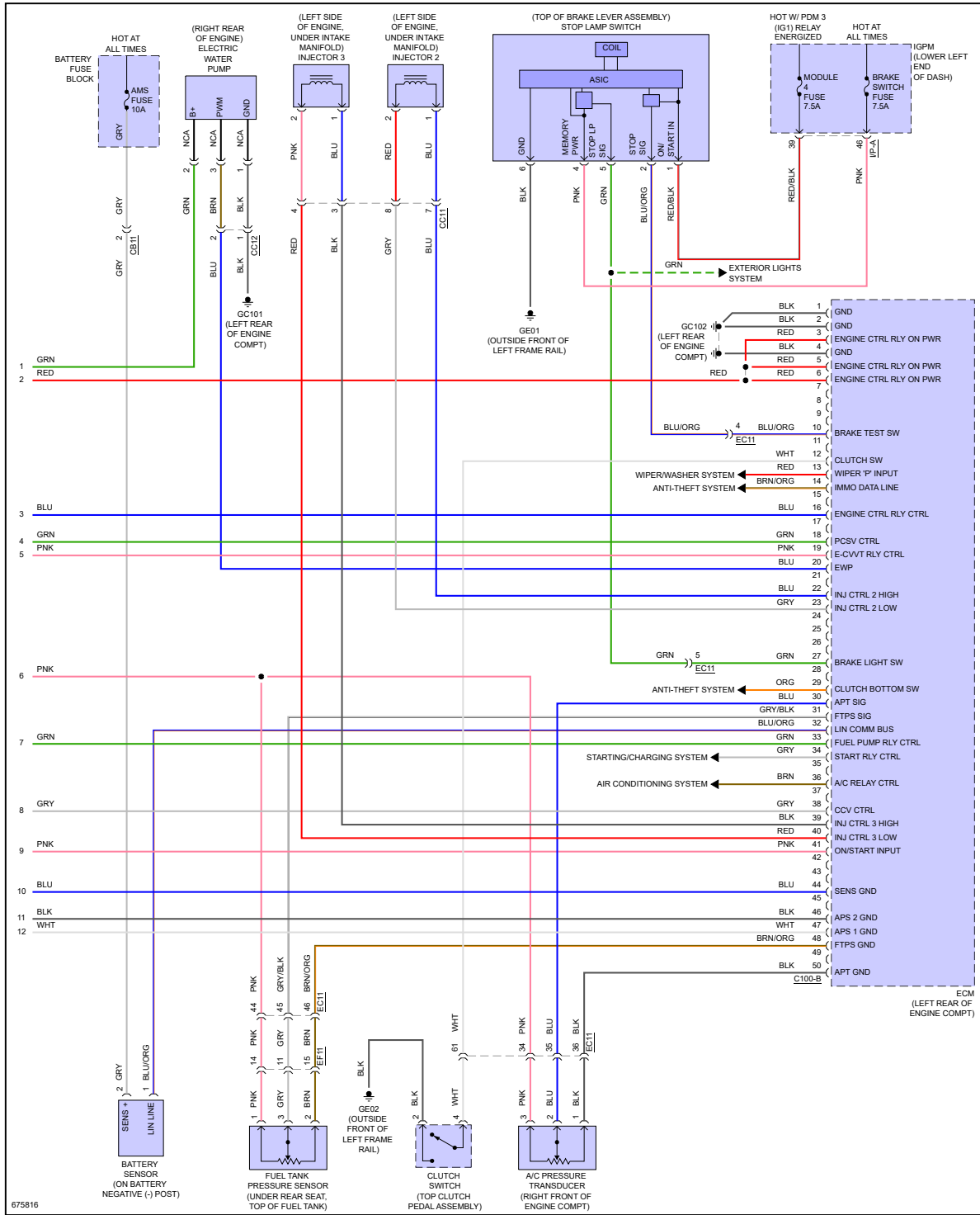
Fig 7: 2.0L Turbo, MFI Control Circuit (7 of 7)
