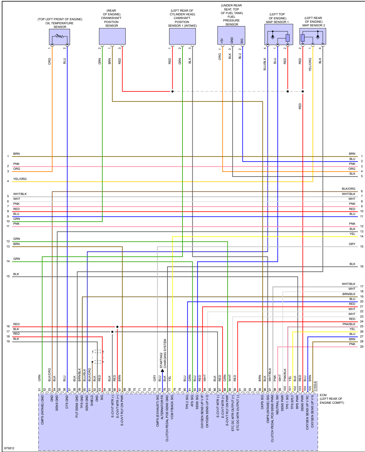
Fig 3: 2.0L Turbo, MFI Control Circuit (3 of 7)
