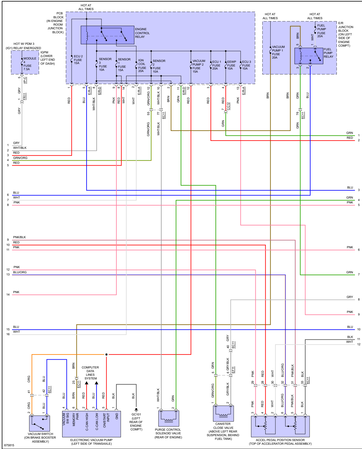
Fig 6: 2.0L Turbo, MFI Control Circuit (6 of 7)
