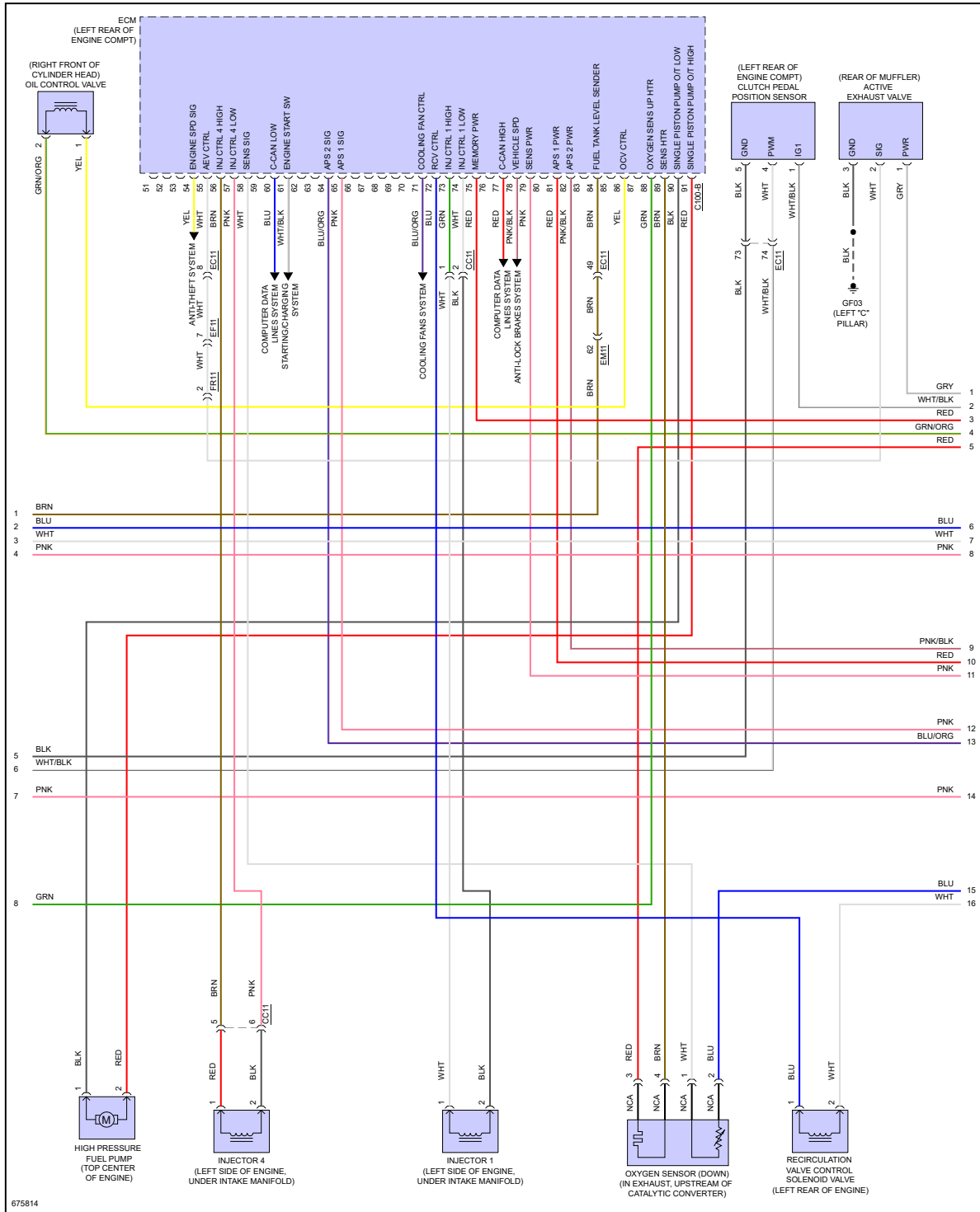
Fig 5: 2.0L Turbo, MFI Control Circuit (5 of 7)
