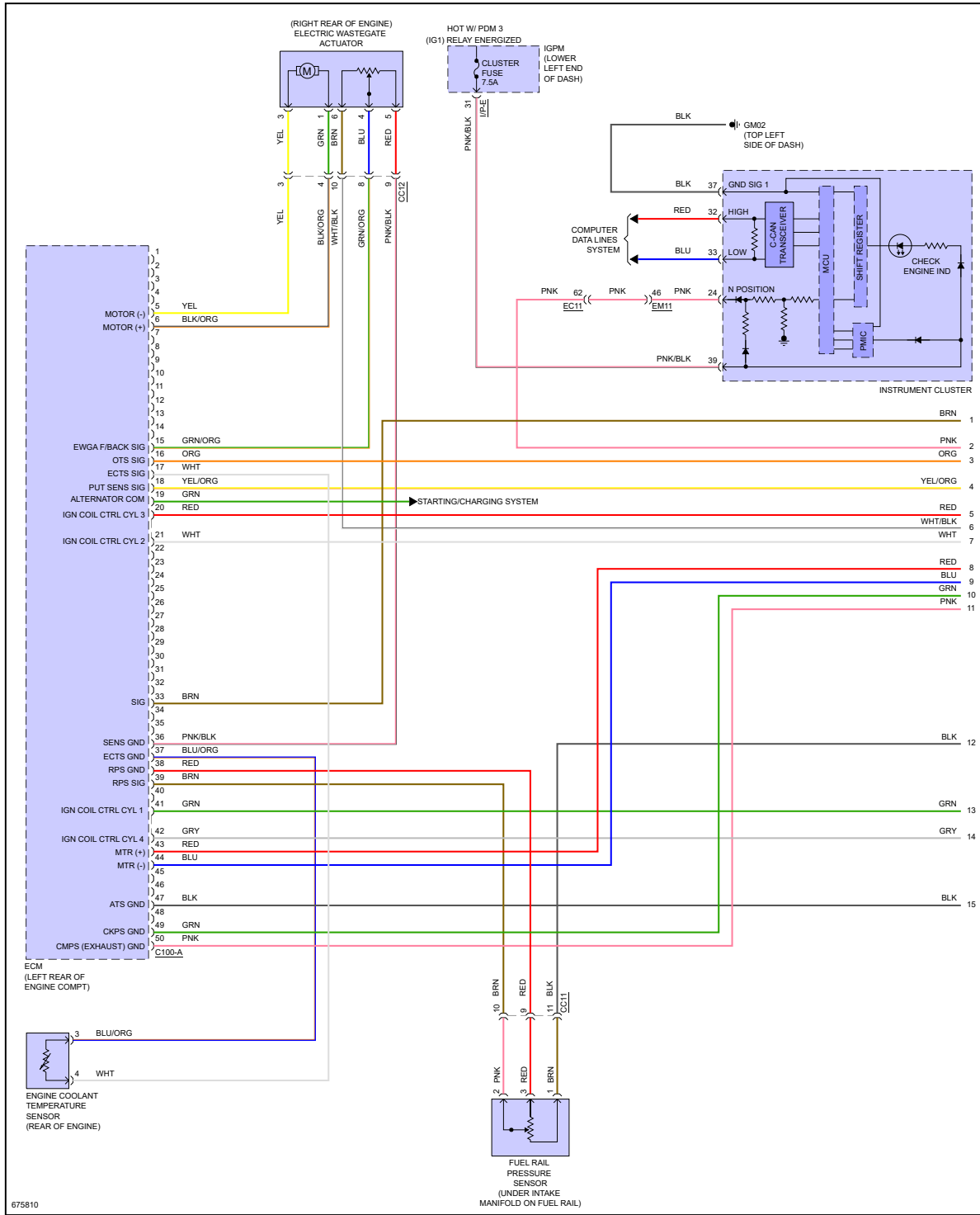
Fig 1: 2.0L Turbo, MFI Control Circuit (1 of 7)
