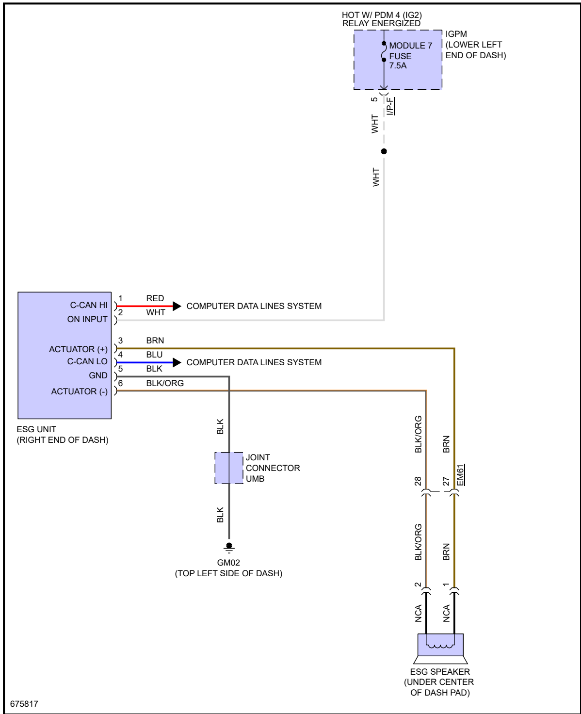
Fig 8: 2.0L Turbo, Virtual Engine Sound System Circuit
