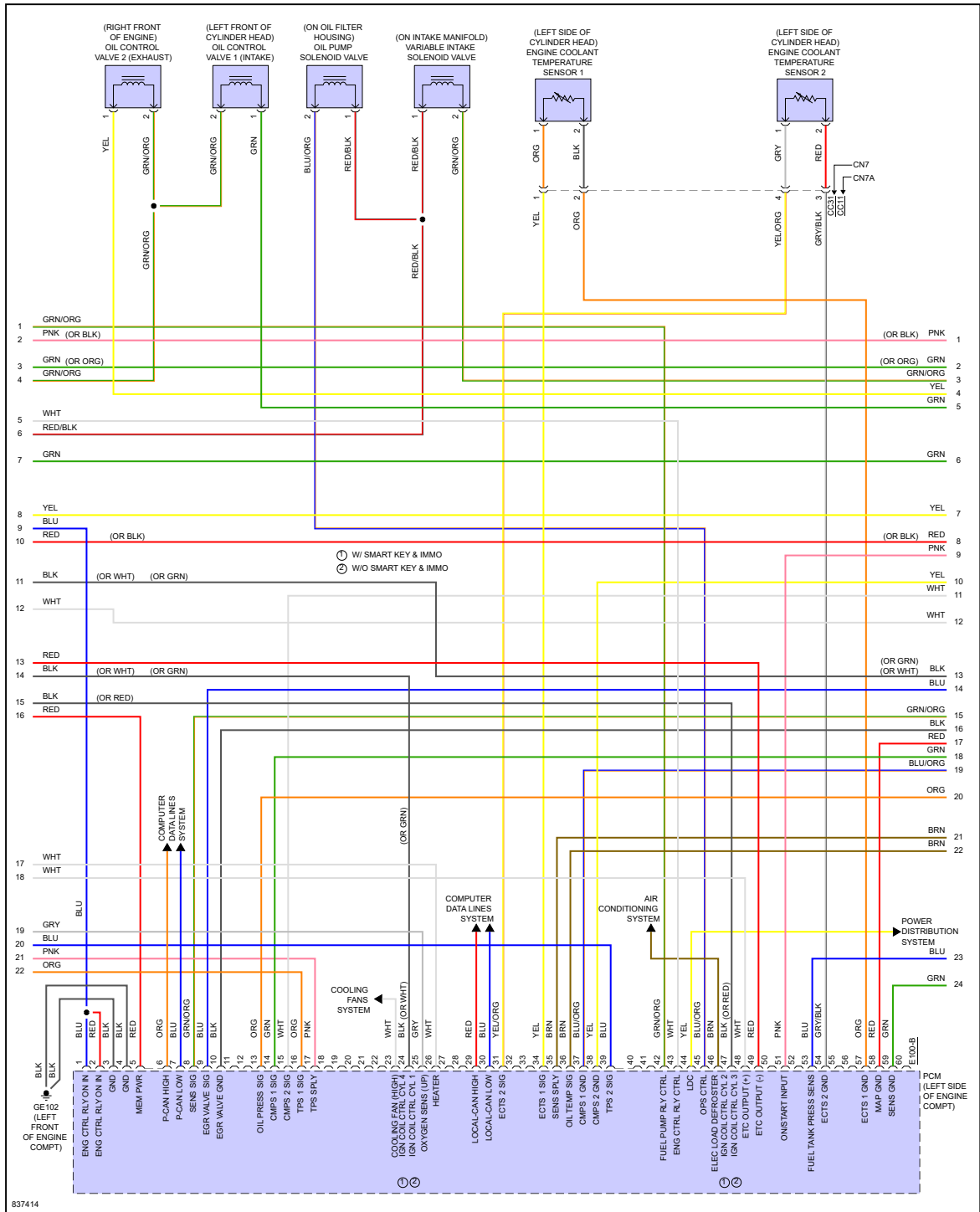
Fig 5: 2.0L, Engine Performance Circuit (5 of 8)
