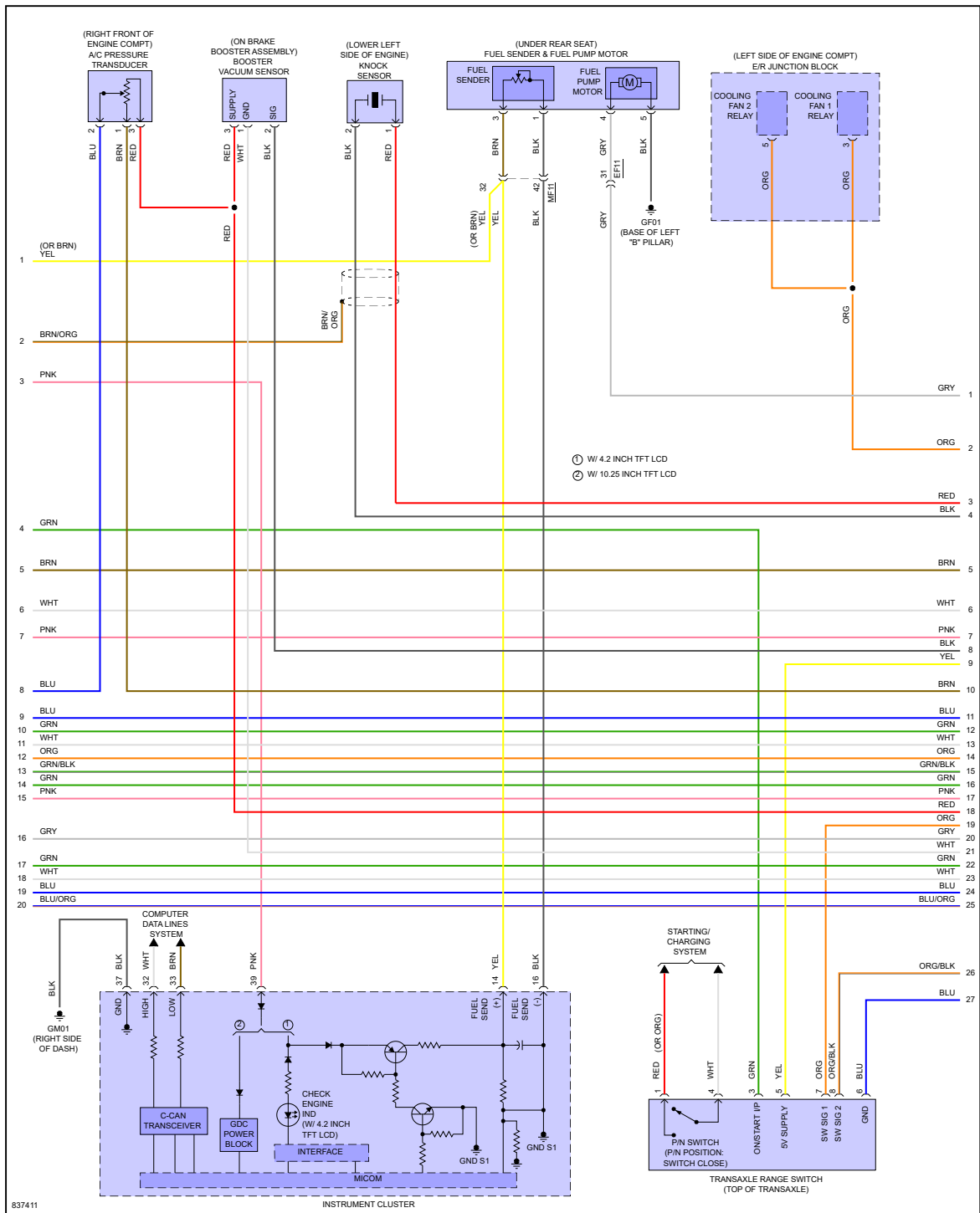
Fig 2: 2.0L, Engine Performance Circuit (2 of 8)
