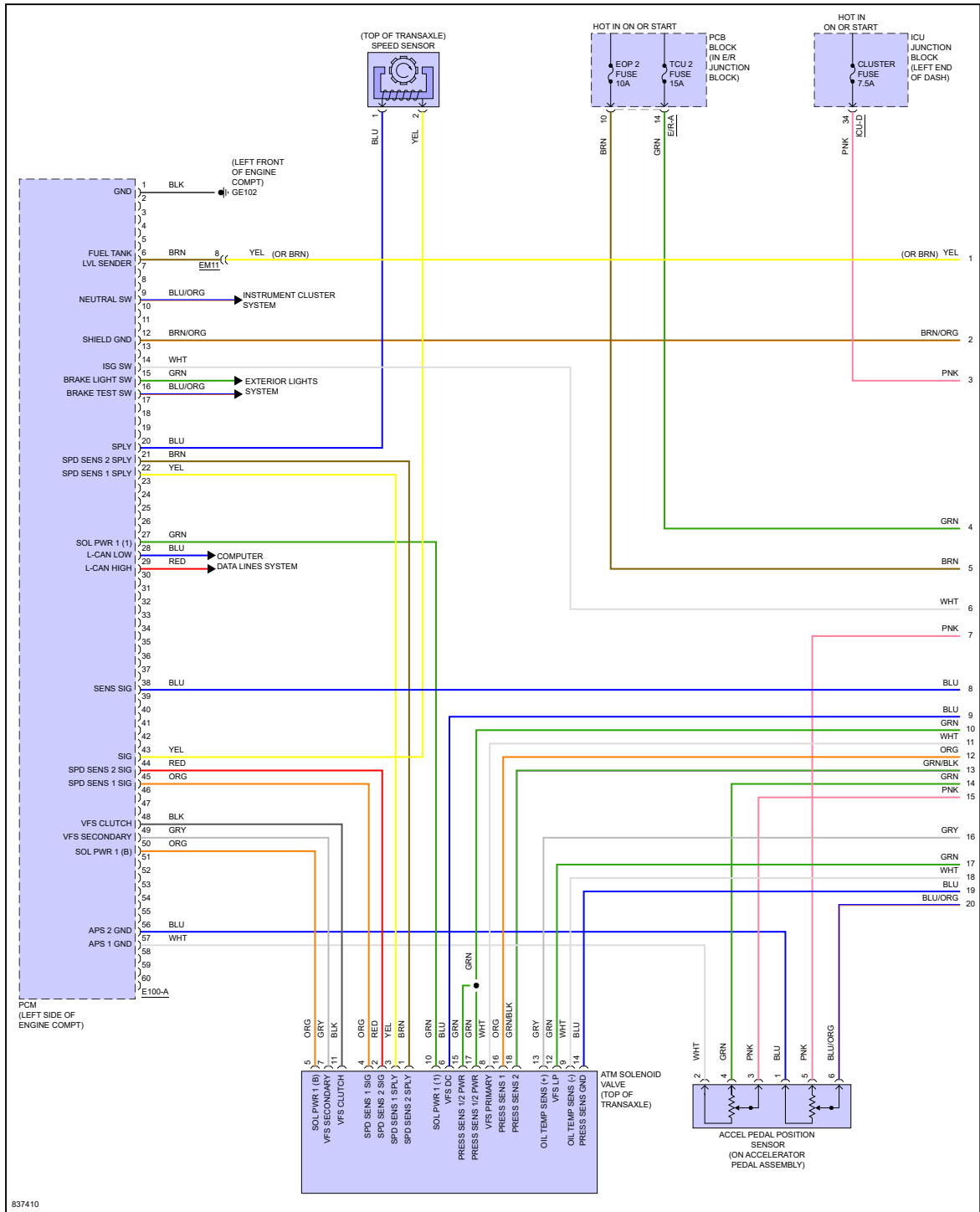
Fig 1: 2.0L, Engine Performance Circuit (1 of 8)
