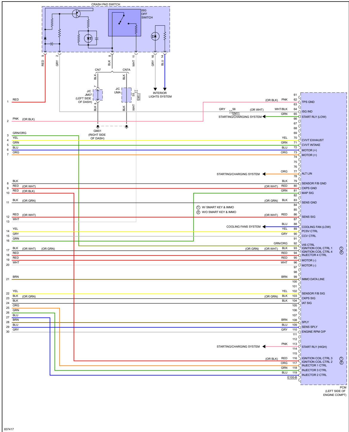
Fig 8: 2.0L, Engine Performance Circuit (8 of 8)
