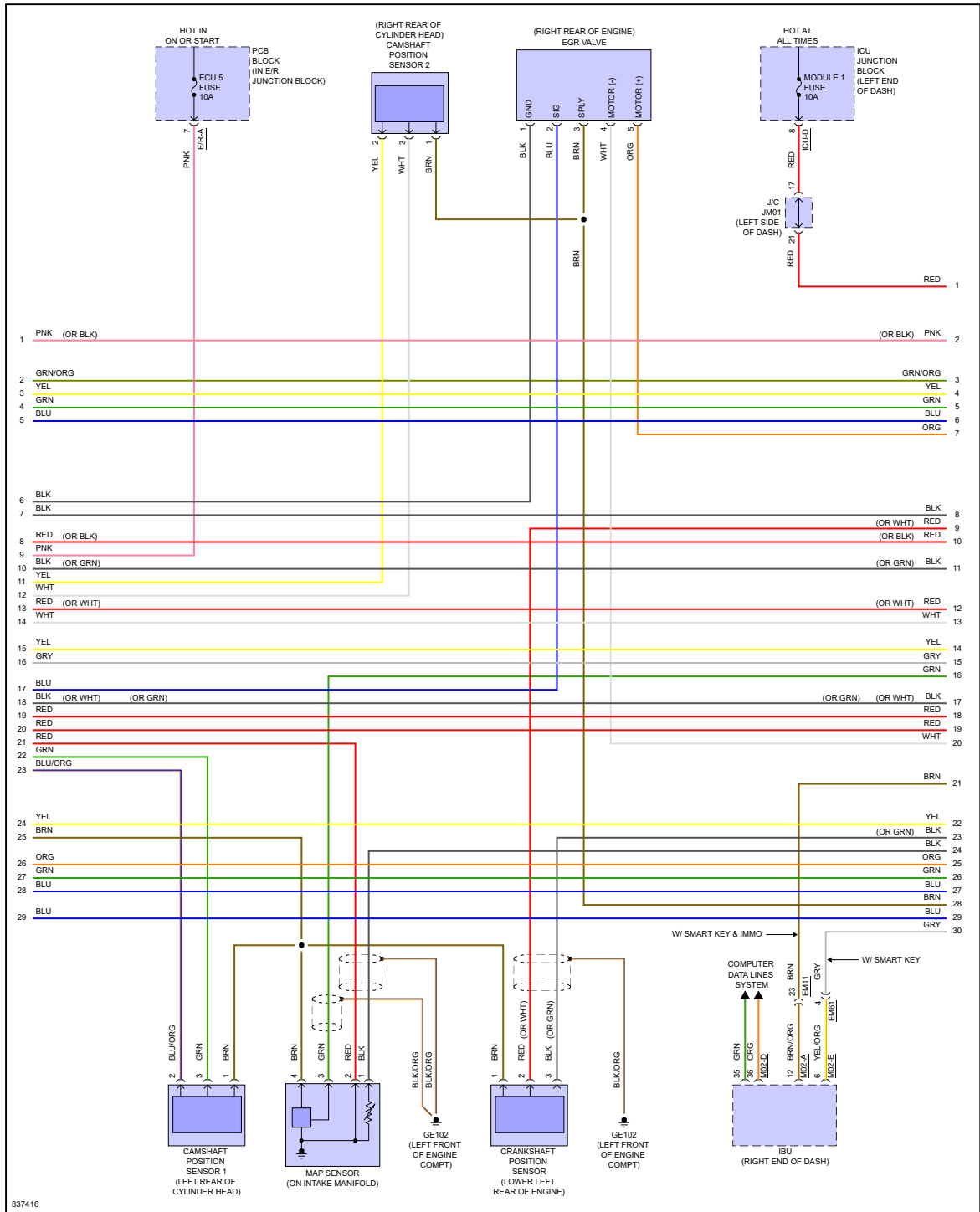
Fig 7: 2.0L, Engine Performance Circuit (7 of 8)
