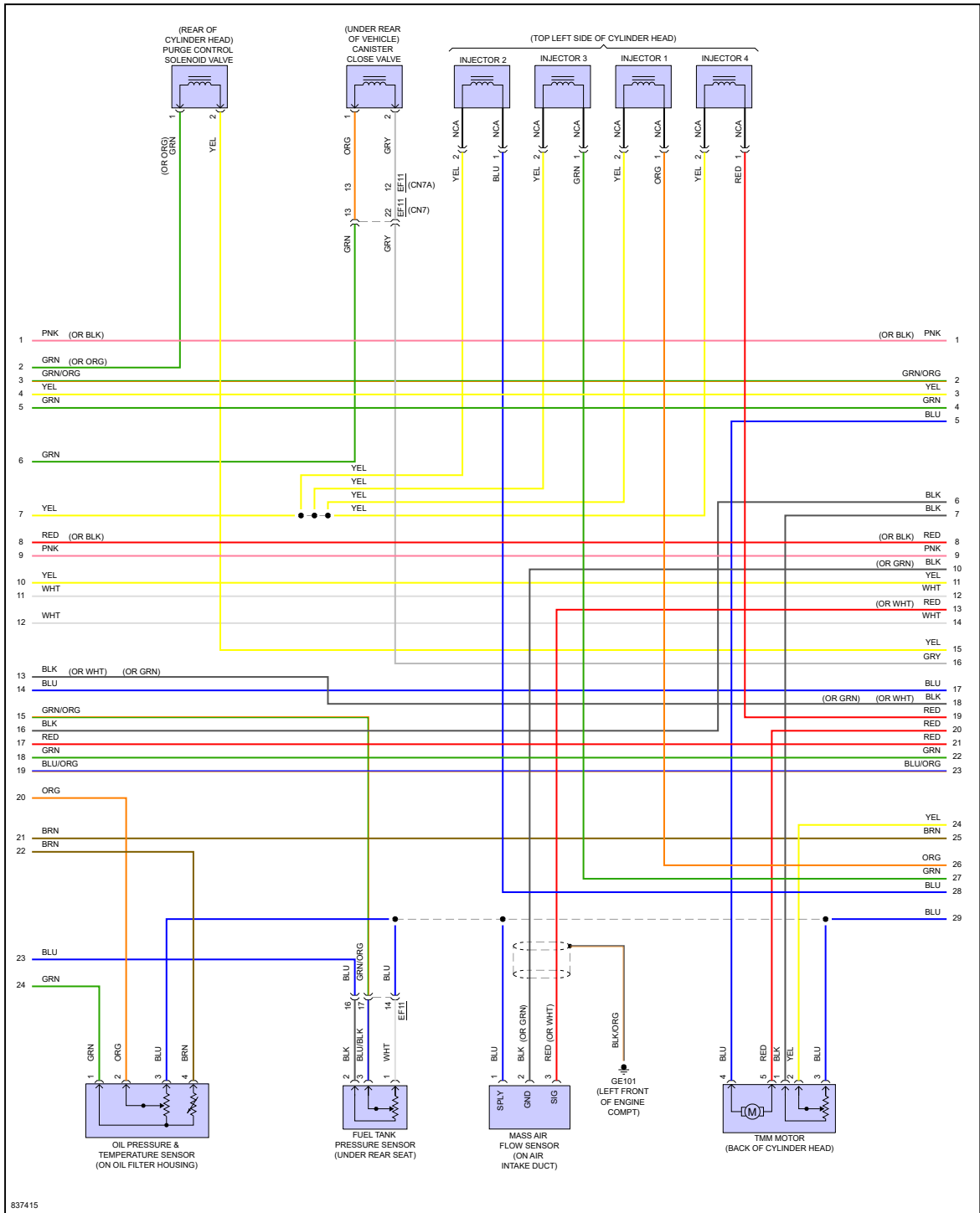
Fig 6: 2.0L, Engine Performance Circuit (6 of 8)
