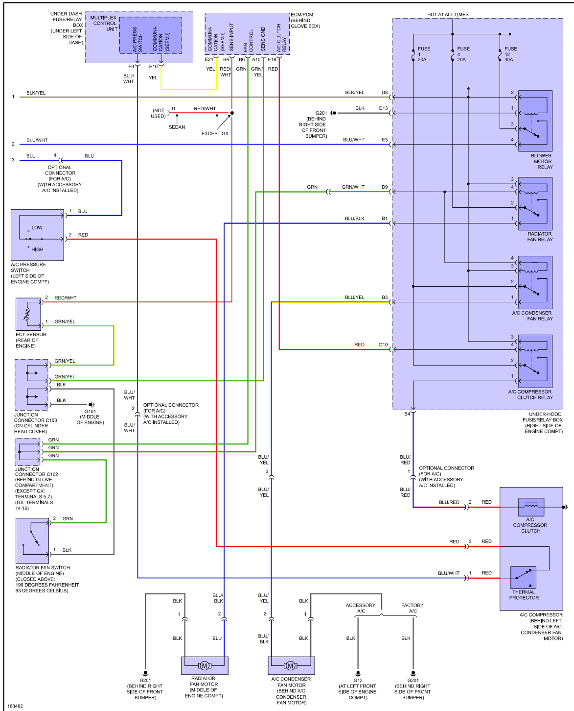
Fig 7: Manual A/C Circuit, Except Hatchback & Hybrid (2 of 2)
