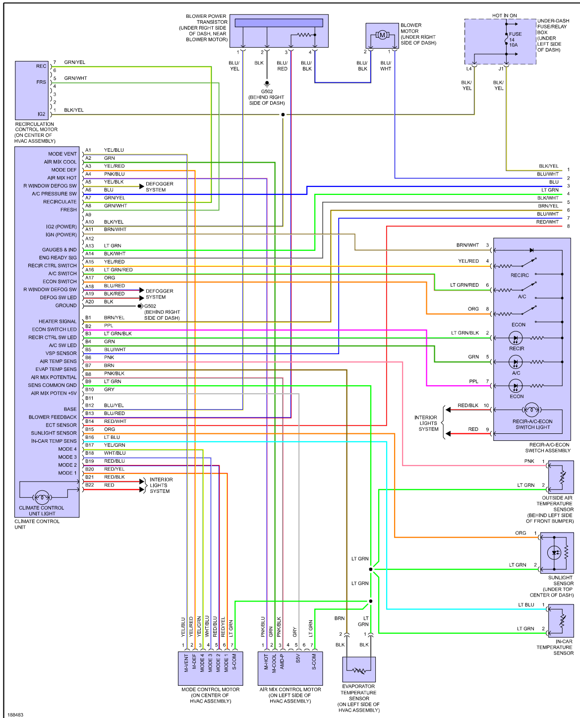
Fig 1: Automatic A/C Circuit, Hybrid (1 of 2)
