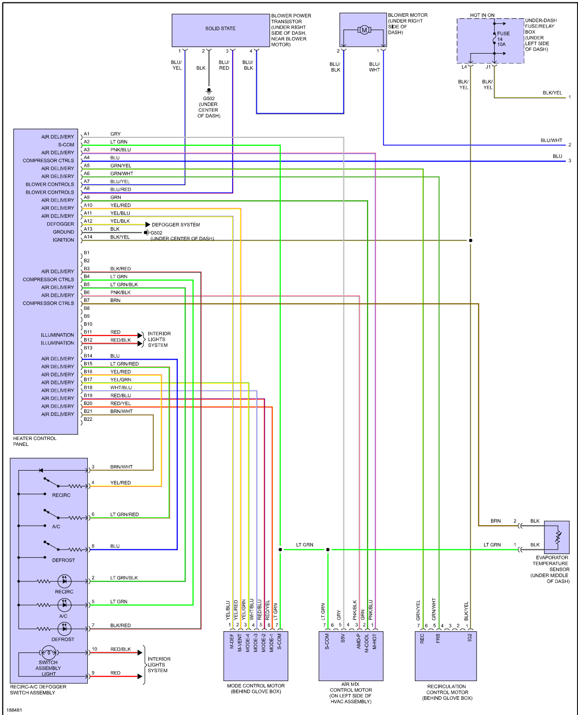
Fig 6: Manual A/C Circuit, Except Hatchback & Hybrid (1 of 2)
