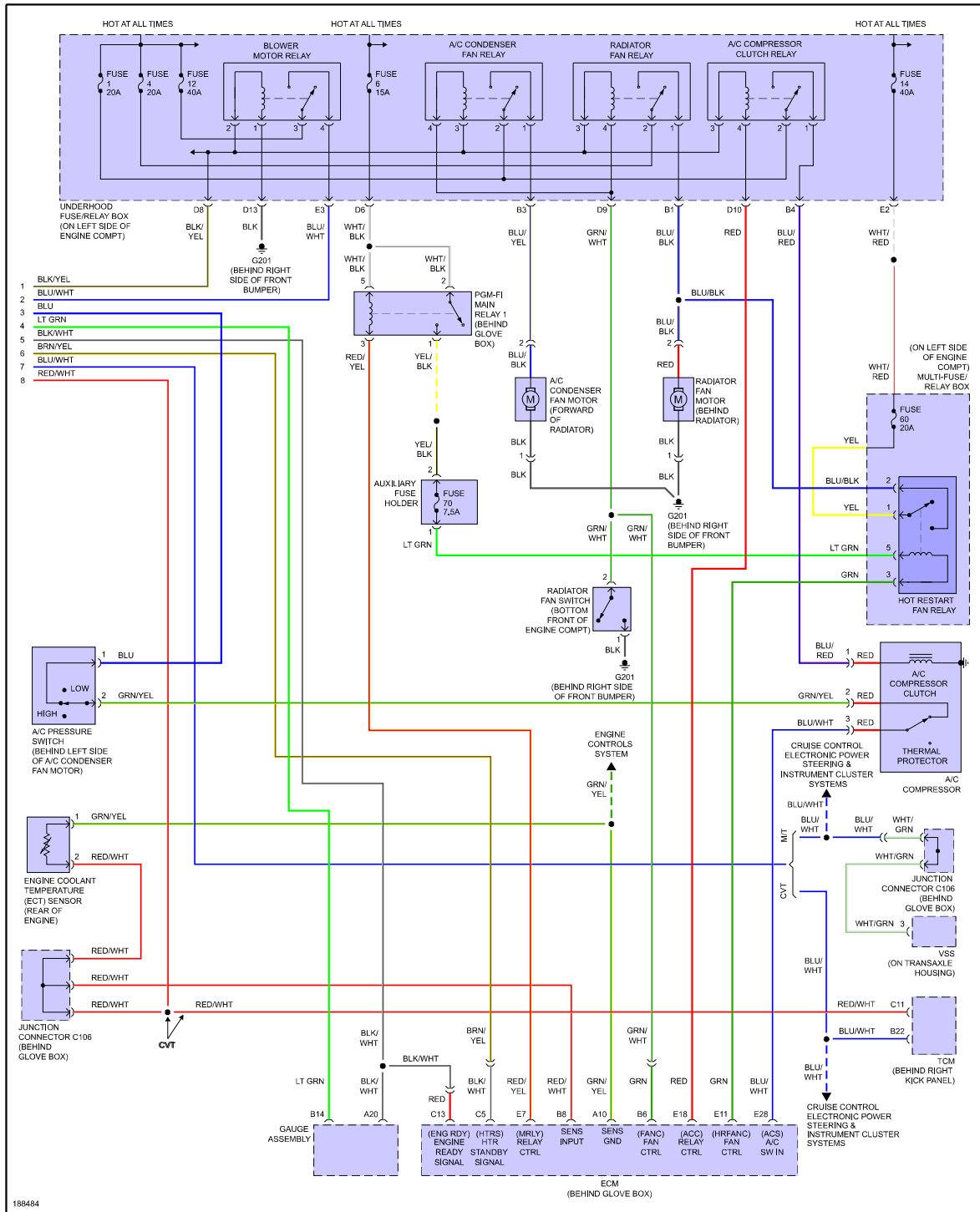
Fig 2: Automatic A/C Circuit, Hybrid (2 of 2)
