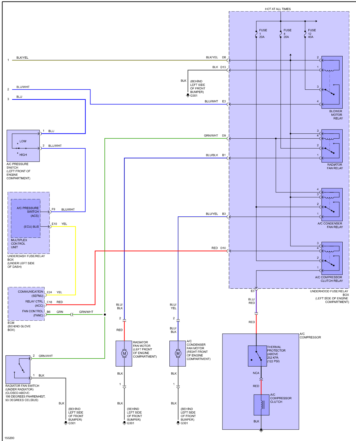
Fig 9: Manual A/C Circuit, Hatchback (2 of 2)
