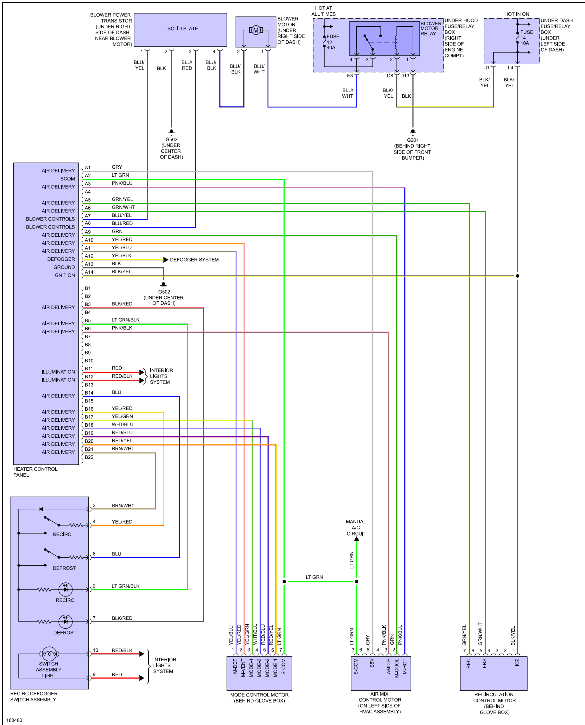
Fig 3: Heater Circuit, Except Hatchback & Hybrid
