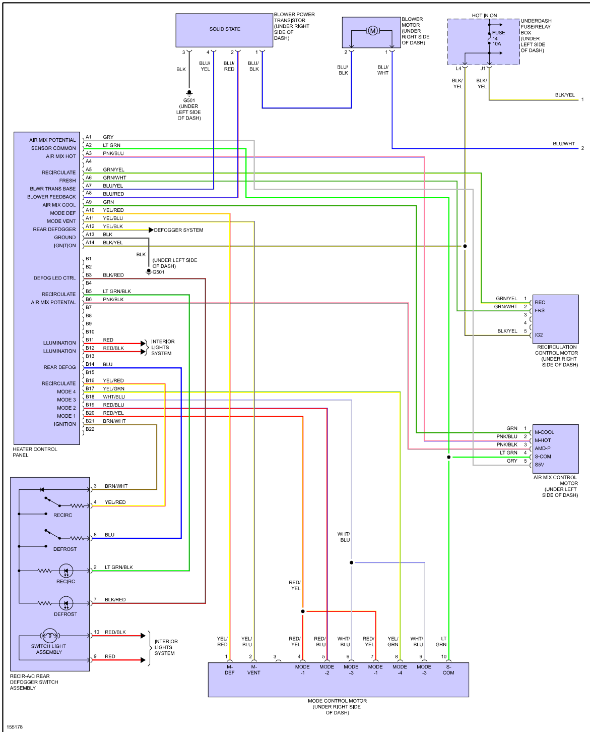
Fig 4: Heater Circuit, Hatchback (1 of 2)
