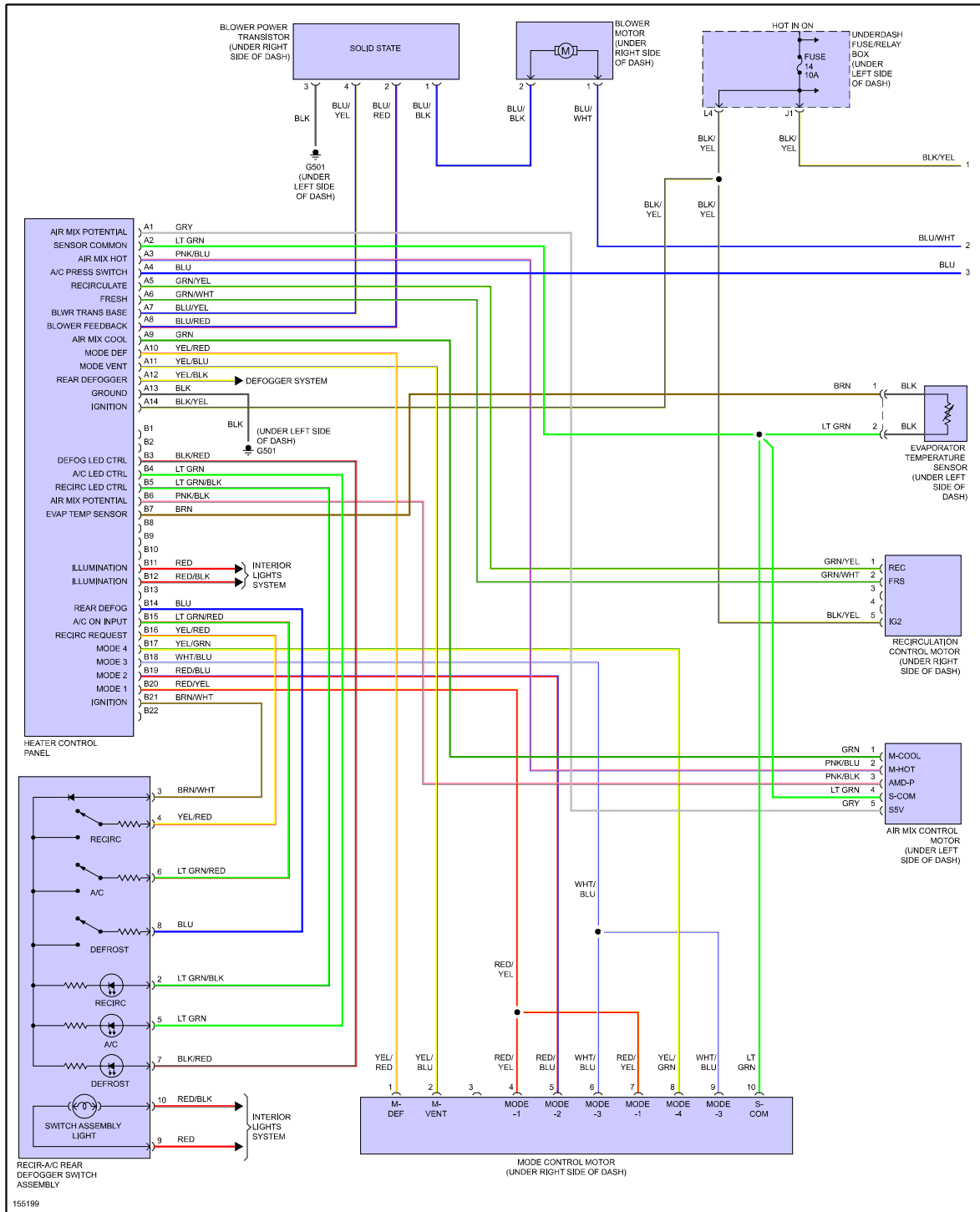
Fig 8: Manual A/C Circuit, Hatchback (1 of 2)
